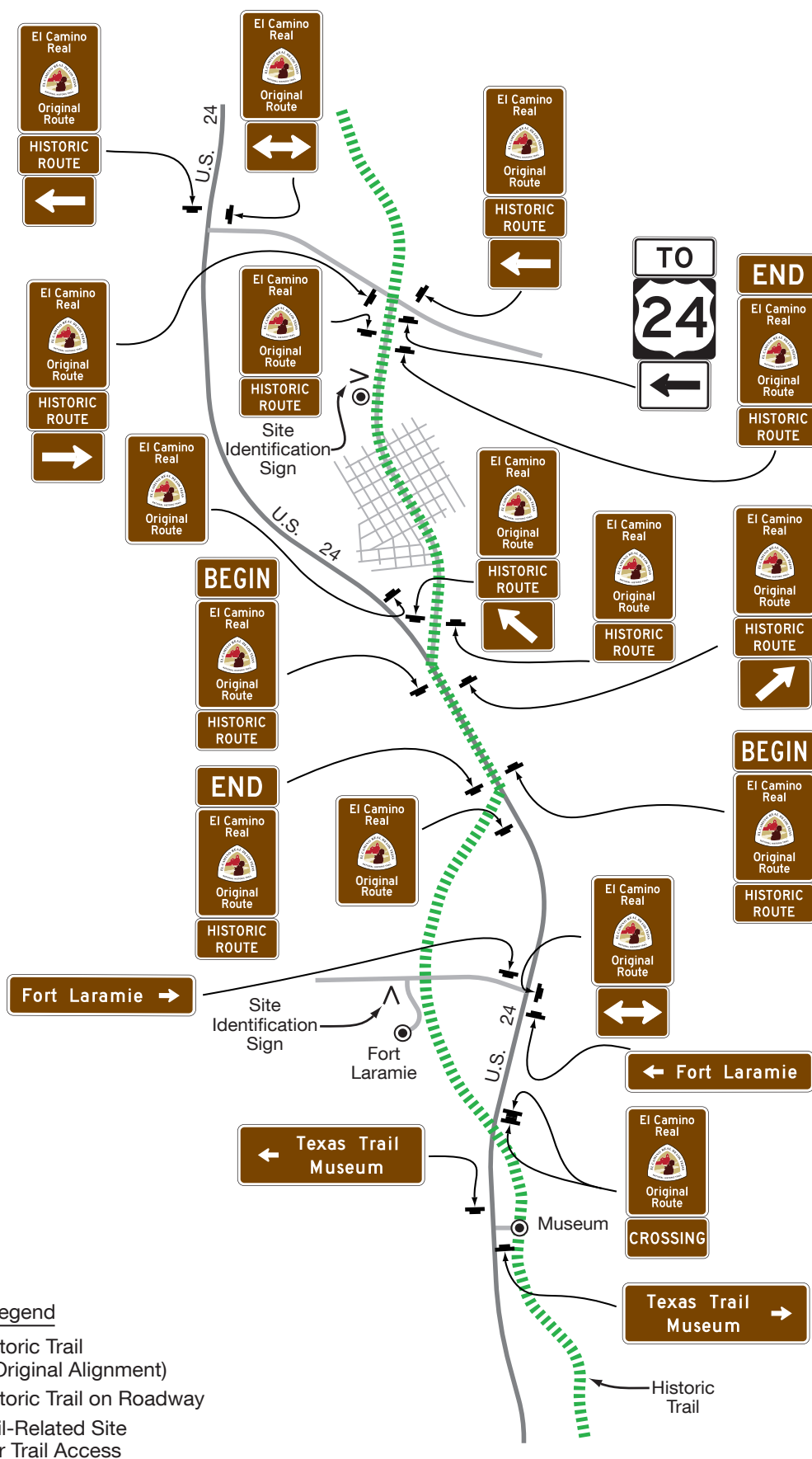
Figure 2D-35. Example of Guide and Directional Signing for a National Historic Trail
