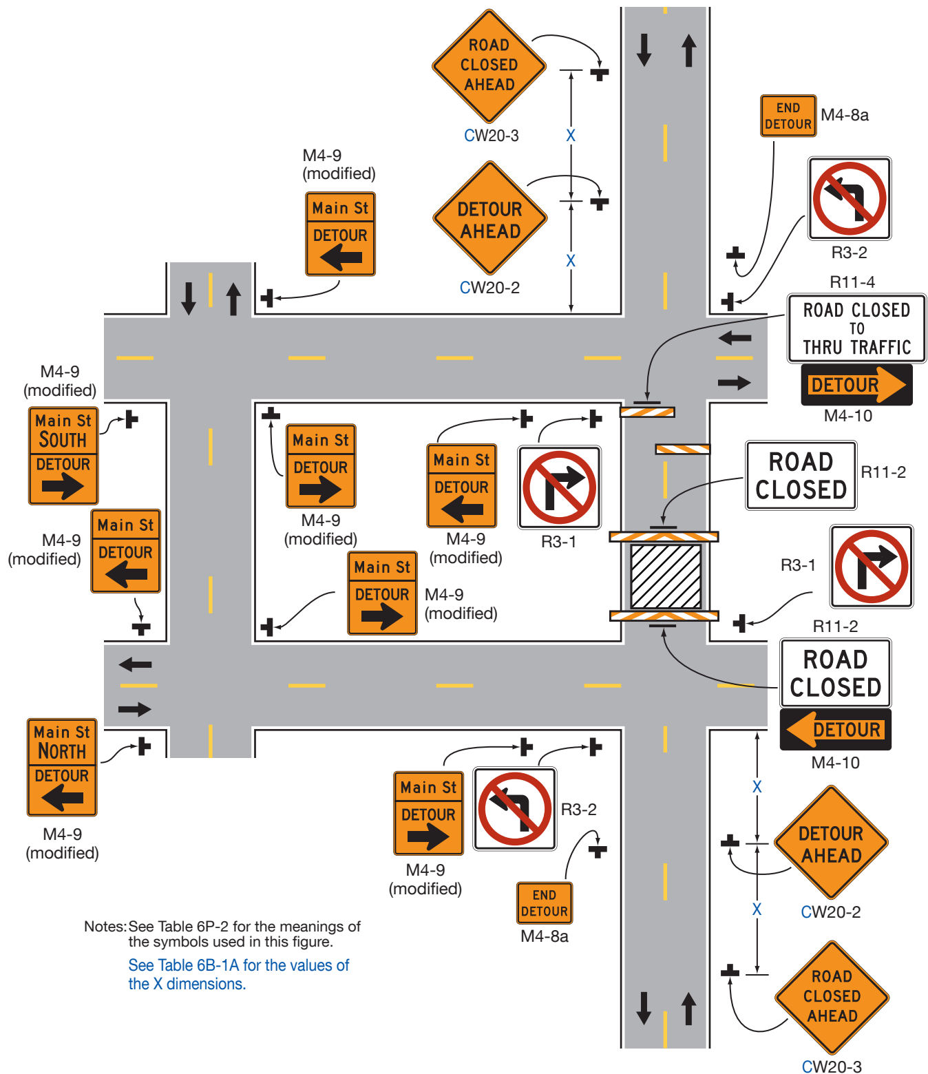
Figure 6P-20. Detour for a Closed Street (TA-20)
