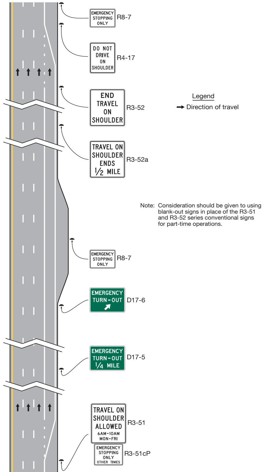
Figure 2G-32. Examples of Signing for Part-Time Travel on Shoulder (Sheet 3 of 4)
