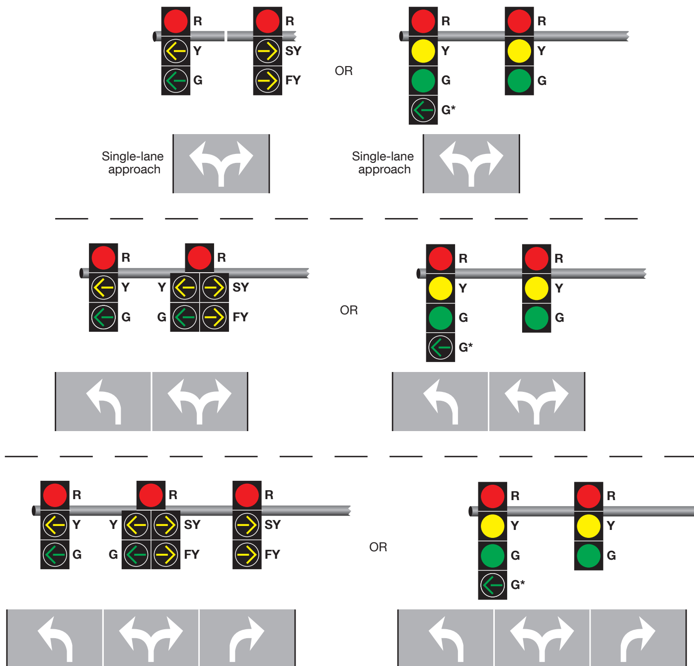
Figure 4F-15. Signal Indications for Approaches with Combined Left-Turn/Right-Turn Lane and No Through Movement (Sheet 2 of 3)
