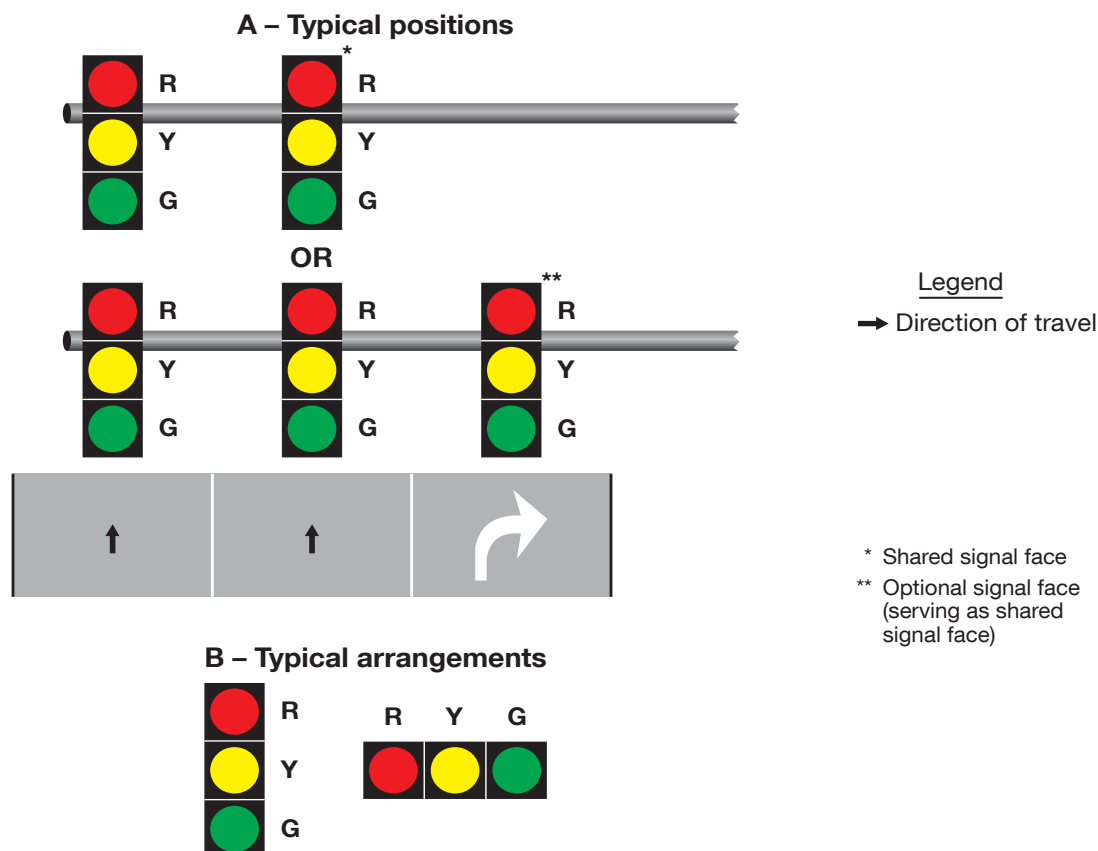
Figure 4F-8. Typical Positions and Arrangements of Shared Signal Faces for Permissive Only Mode Right Turns
