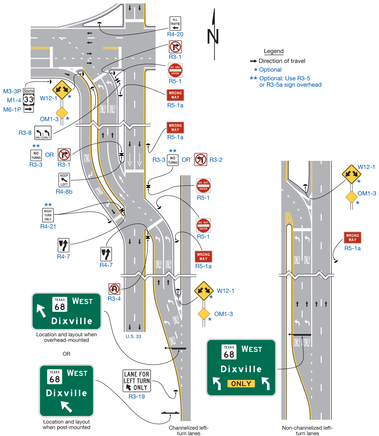
Figure 2D-13. Examples of Signing for Intersections with Indirect Left Turns (Sheet 3 of 3)
