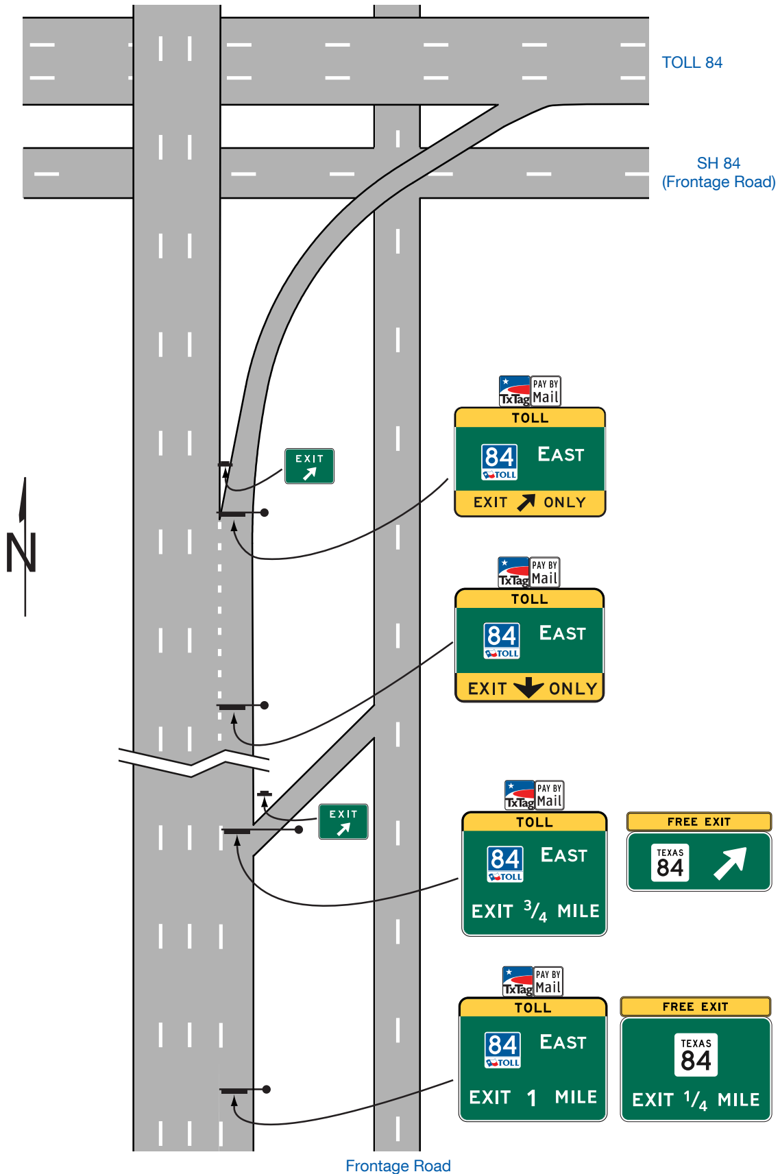
Figure 2F-12A. (TX) Examples of Guide Signs from the Main Lane to a Toll Road with a Non-Toll Frontage Road
