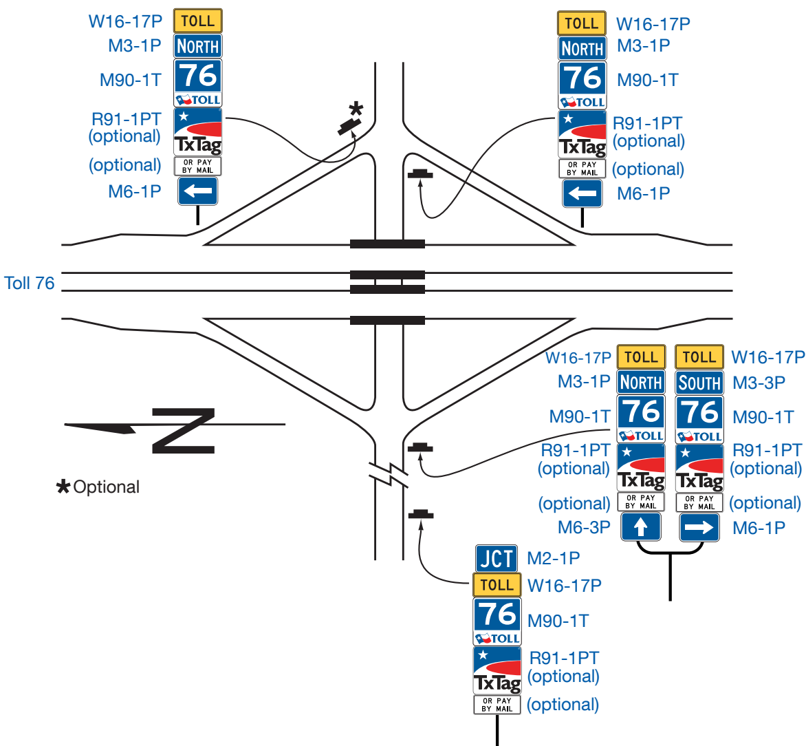
Figure 2F-5. Example of Minor Interchange Crossroad Signing for an Approach to a Toll Highway
