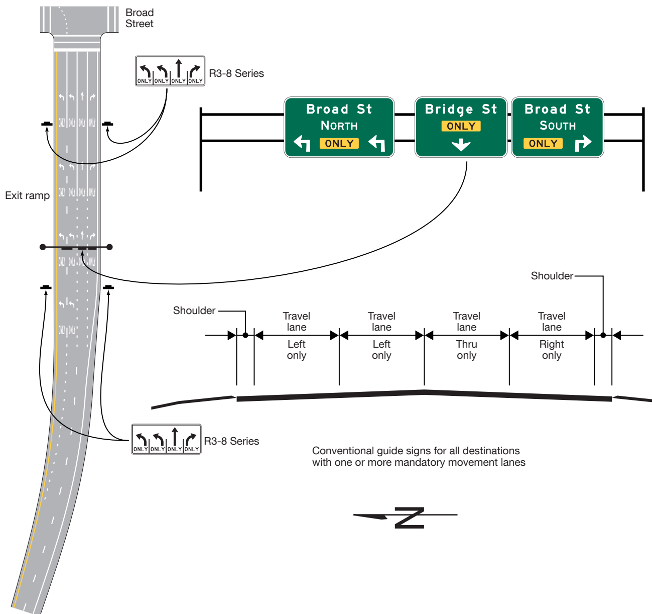
Figure 2D-10. Examples of Overhead Signs at an Intersection (Sheet 3 of 3)
