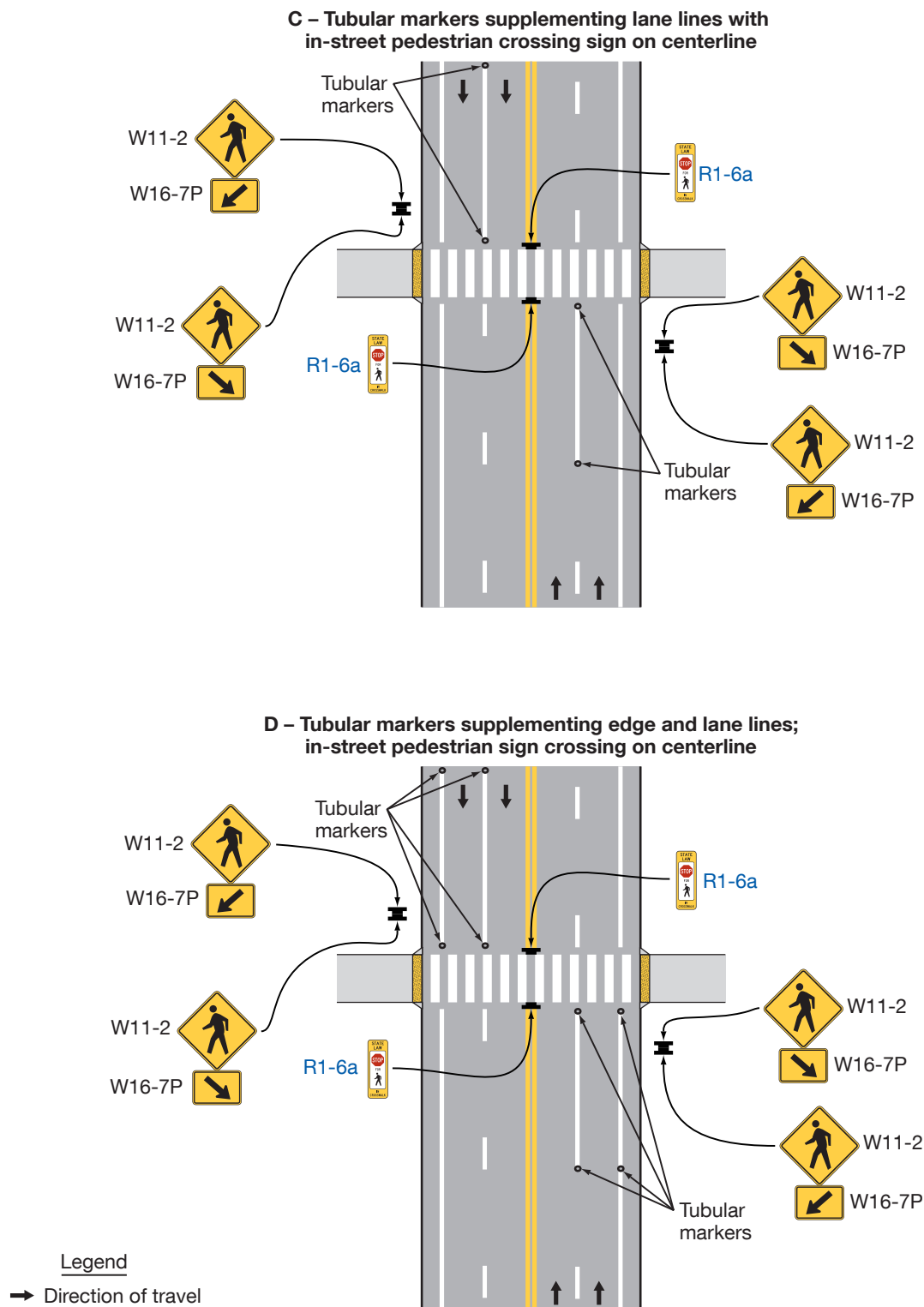
Figure 3I-1. Examples of Tubular Markers Supplementing Pavement Markings in Advance of an Unsignalized Crosswalk (Sheet 2 of 2)
