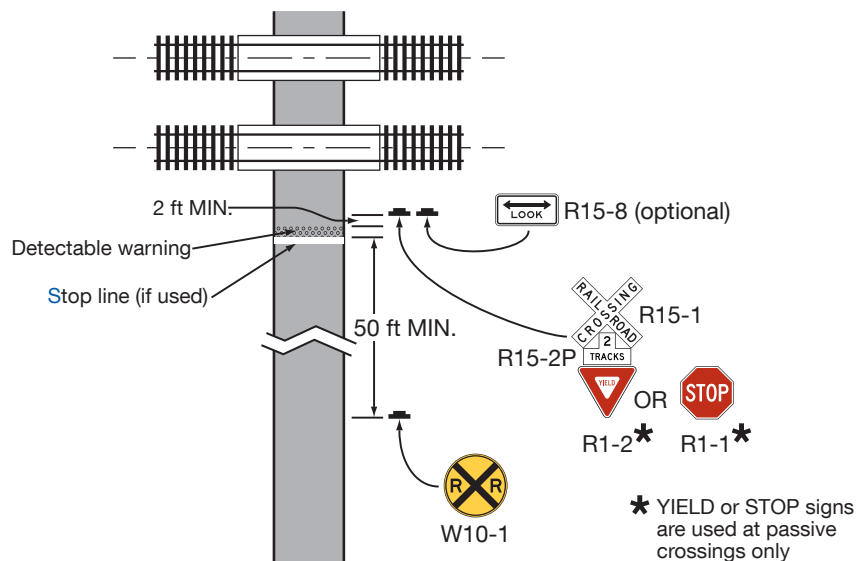
Figure 8E-3. Example of Signing and Markings at a Pathway Grade Crossing
