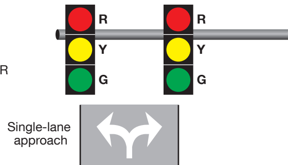
Figure 4F-15. Signal Indications for Approaches with Combined Left-Turn/Right-Turn Lane and No Through Movement (Sheet 3 of 3)
