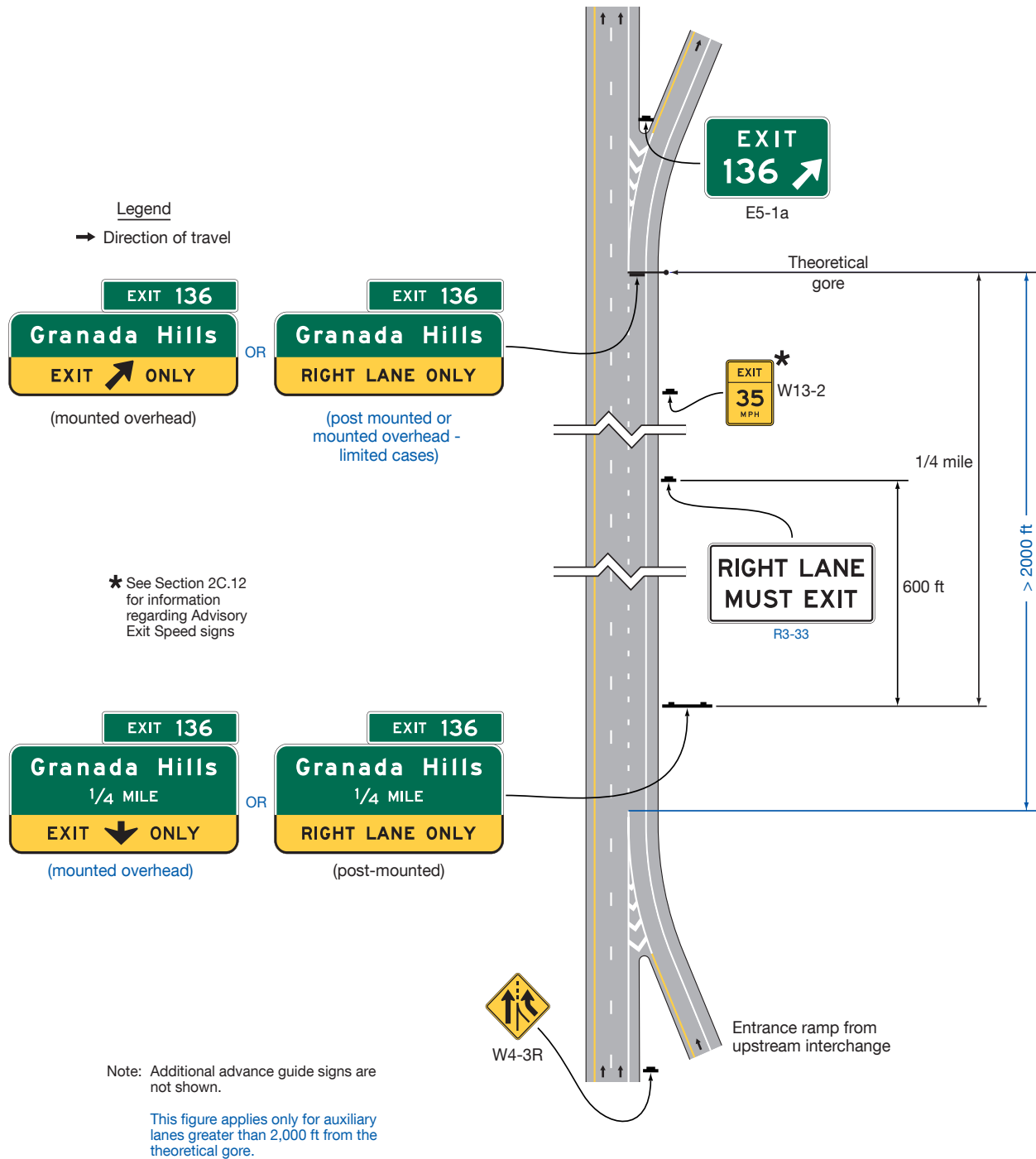
Figure 2E-21. Example of Advance Guide and Supplemental Signs for a Dropped Auxiliary Lane between Separate Interchange Ramps
