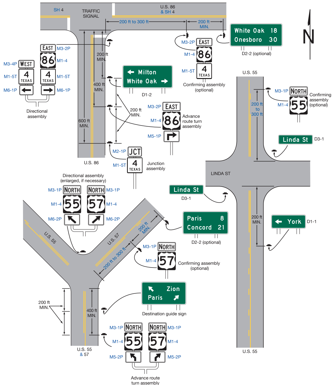
Figure 2D-8. Illustration of Directional Assemblies and Other Route Signs (Sheet 3 of 4)
