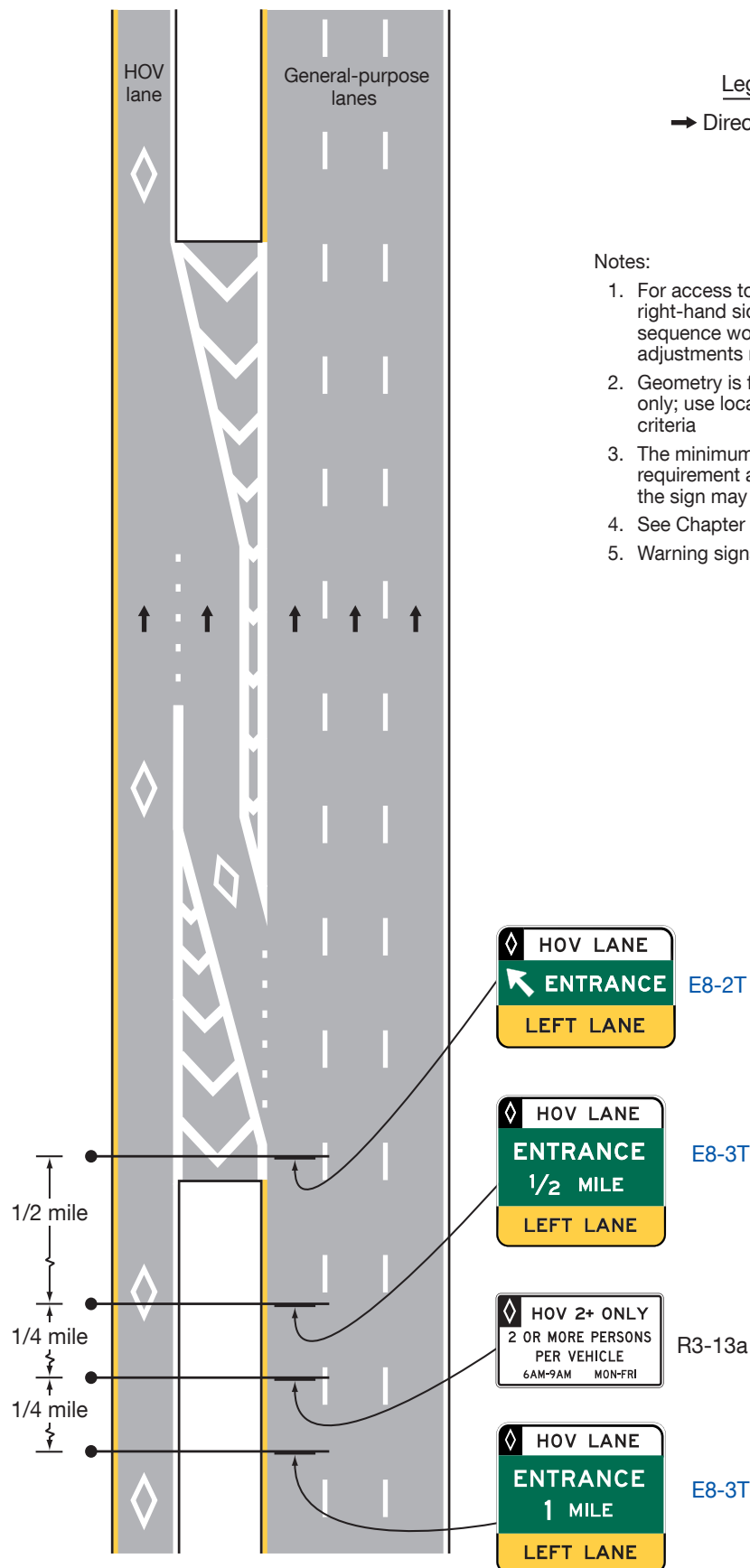
Figure 2G-10. Example of Signing for an Intermediate Entry to a Barrier or Buffer-Separated HOV Lane
