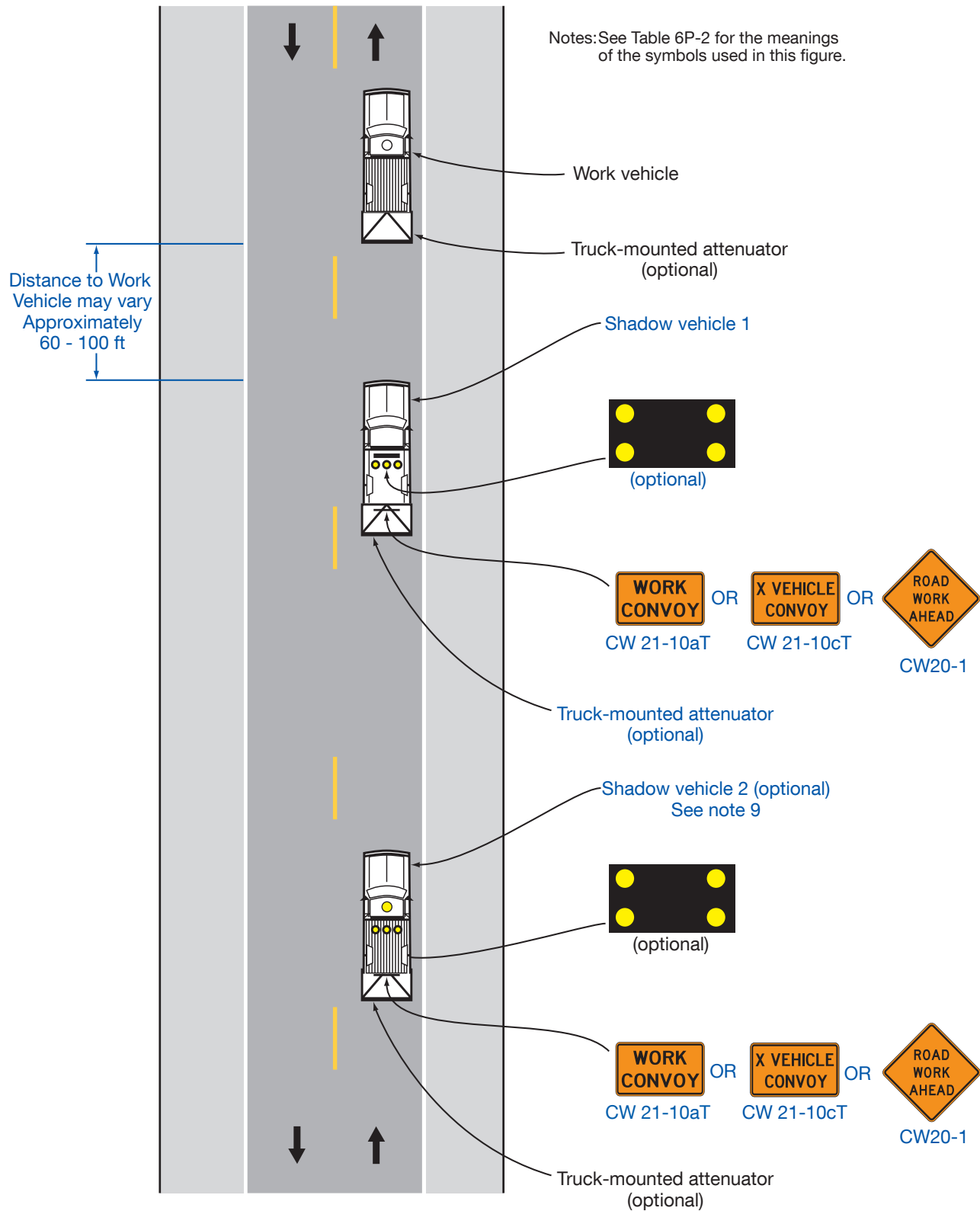
Figure 6P-17. Mobile Operations on a Two-Lane Road (TA-17)
