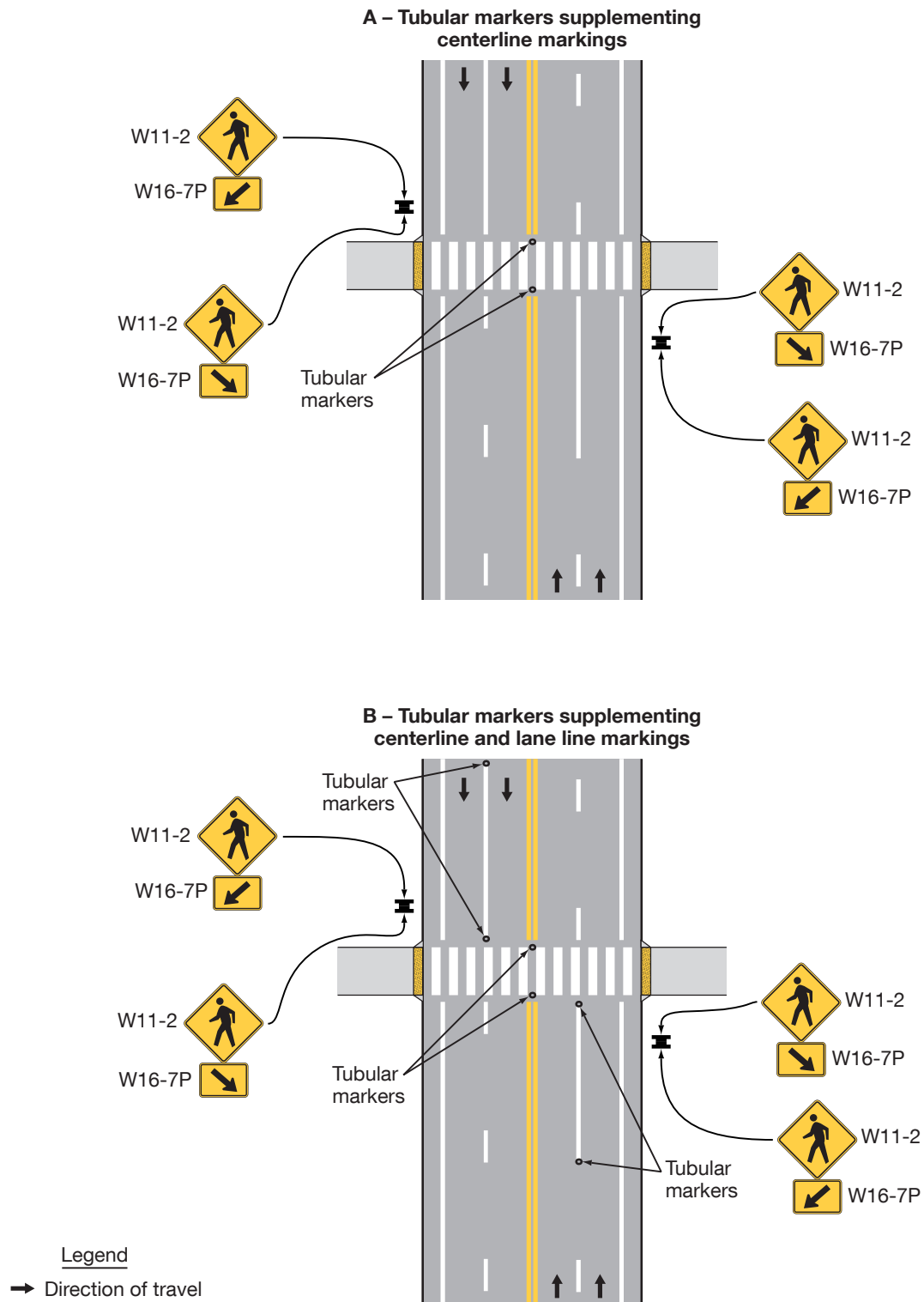
Figure 3I-1. Examples of Tubular Markers Supplementing Pavement Markings in Advance of an Unsignalized Crosswalk (Sheet 1 of 2)
