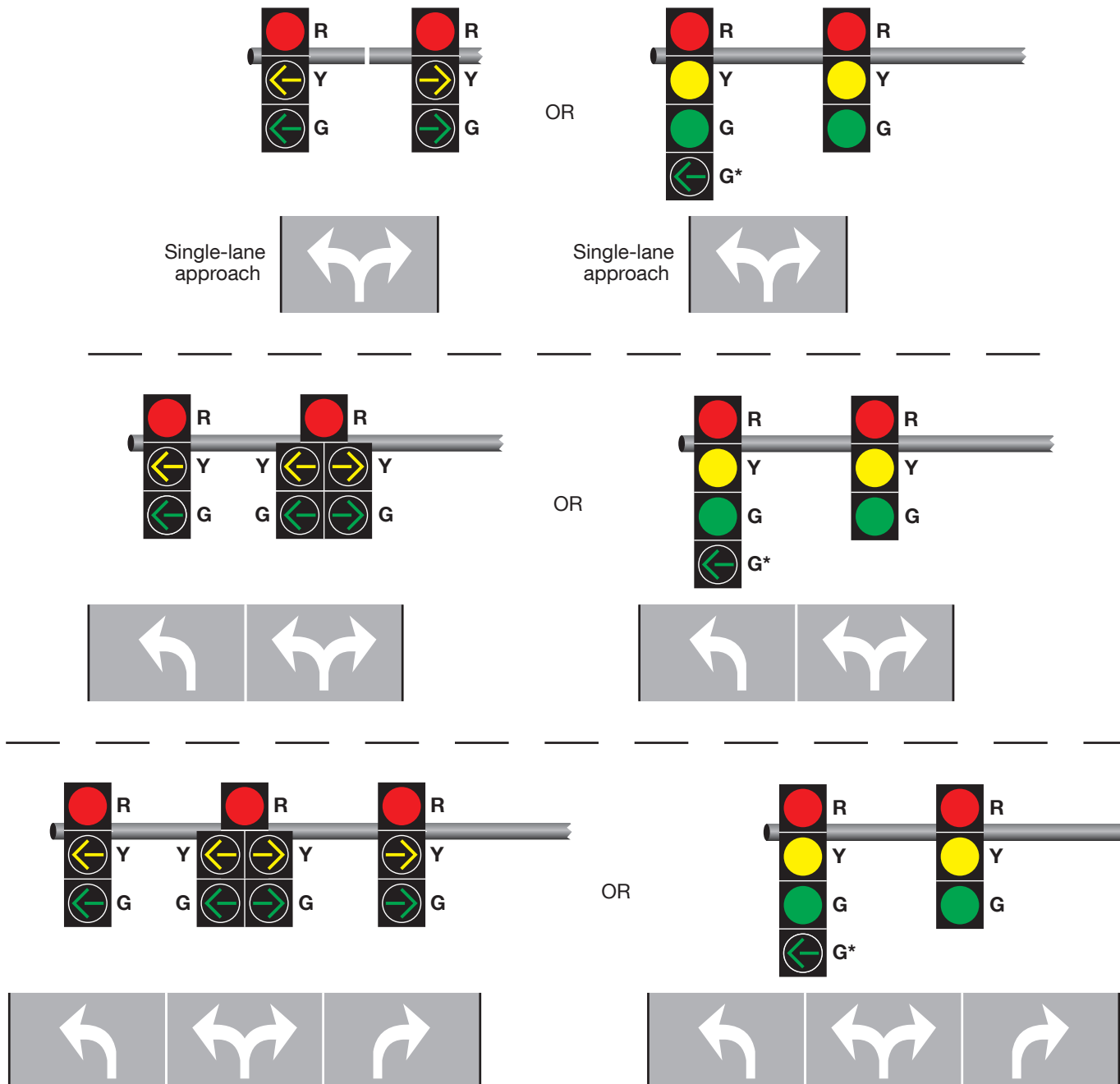
Figure 4F-15. Signal Indications for Approaches with Combined Left-Turn/Right-Turn Lane and No Through Movement (Sheet 1 of 3)
