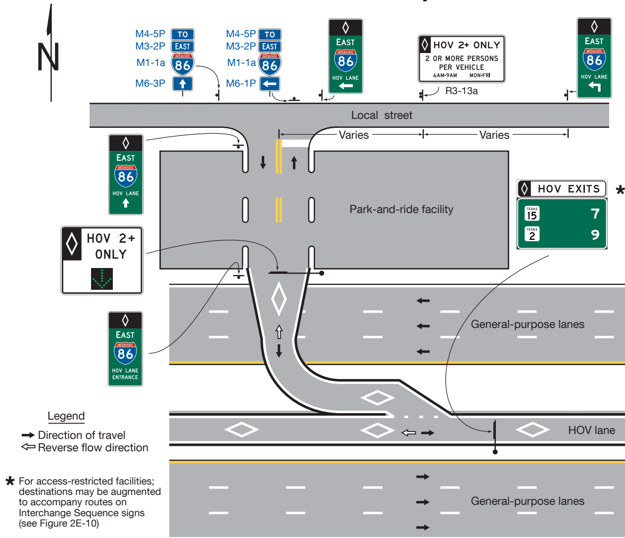
Figure 2G-14. Example of Signing for a Direct Entrance Ramp to an HOV Lane from a Park-and-Ride Facility and a Local Street
