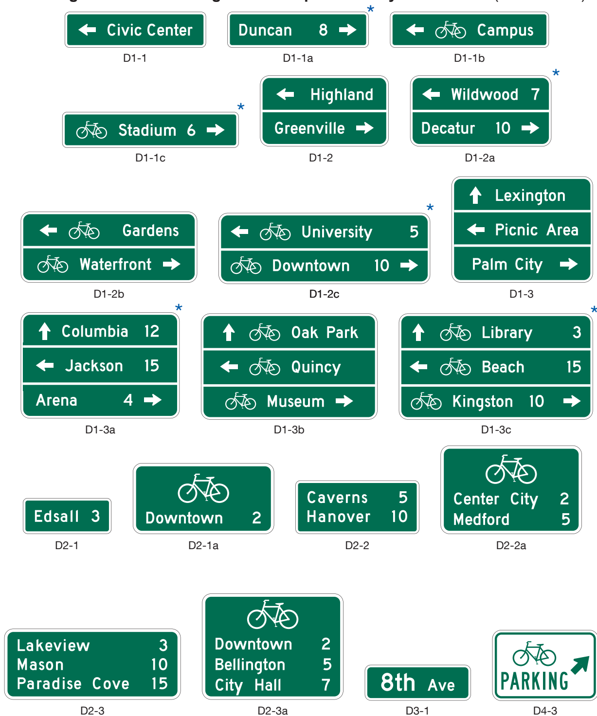
Figure 9D-1. Guide Signs and Plaques for Bicycle Facilities (Sheet 1 of 3)
