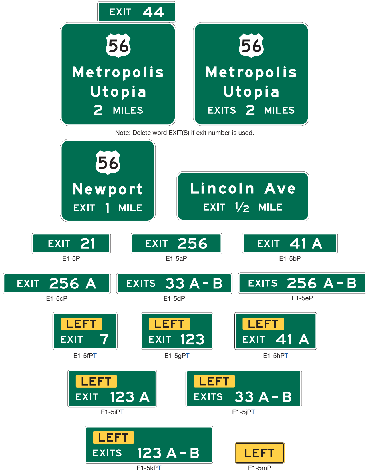
Figure 2E-9. Examples of Interchange Advance Guide Signs, Exit Number Plaques, and LEFT Plaque
