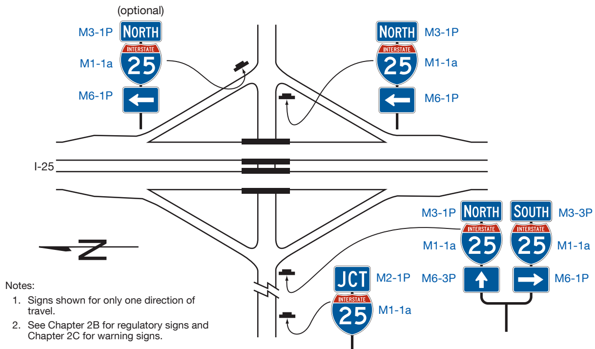
Figure 2D-16. Example of Minor Interchange Crossroad Guide Signing
