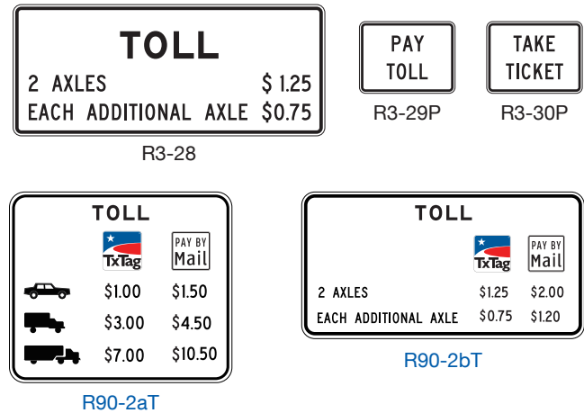
Figure 2F-2. Toll Plaza Regulatory Signs and Plaques
