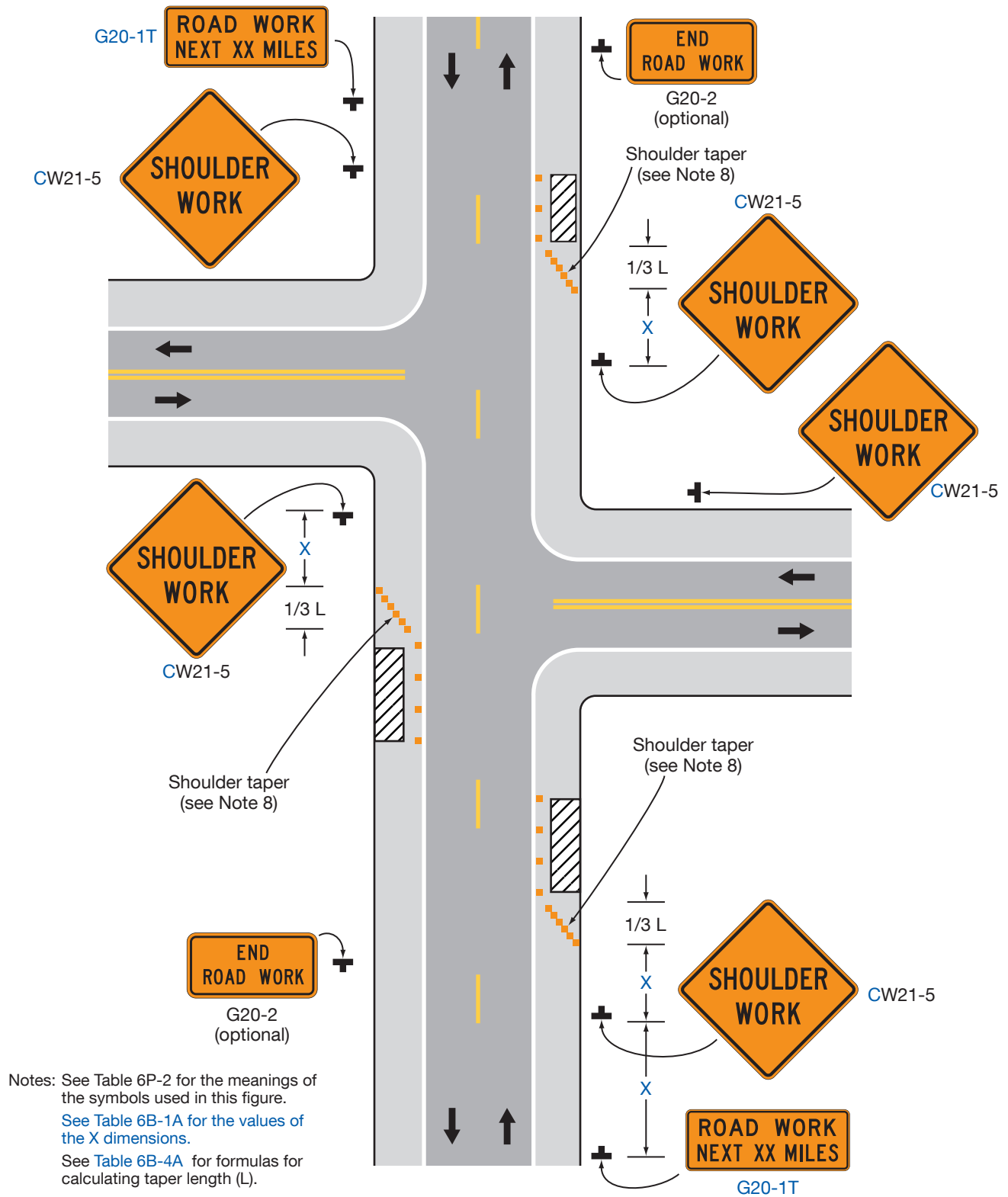
Figure 6P-3. Work on the Shoulders (TA-3)
