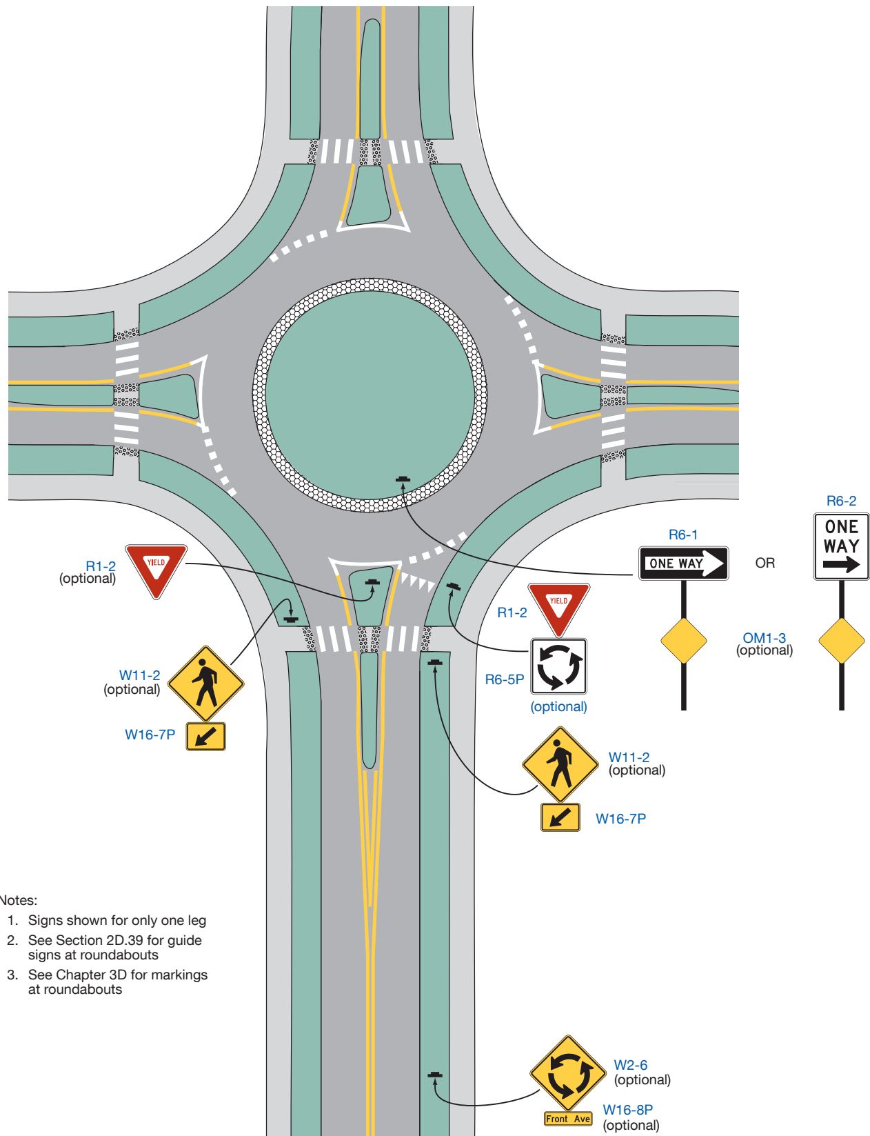
Figure 2B-22. Example of Regulatory and Warning Signs for a One-Lane Roundabout
