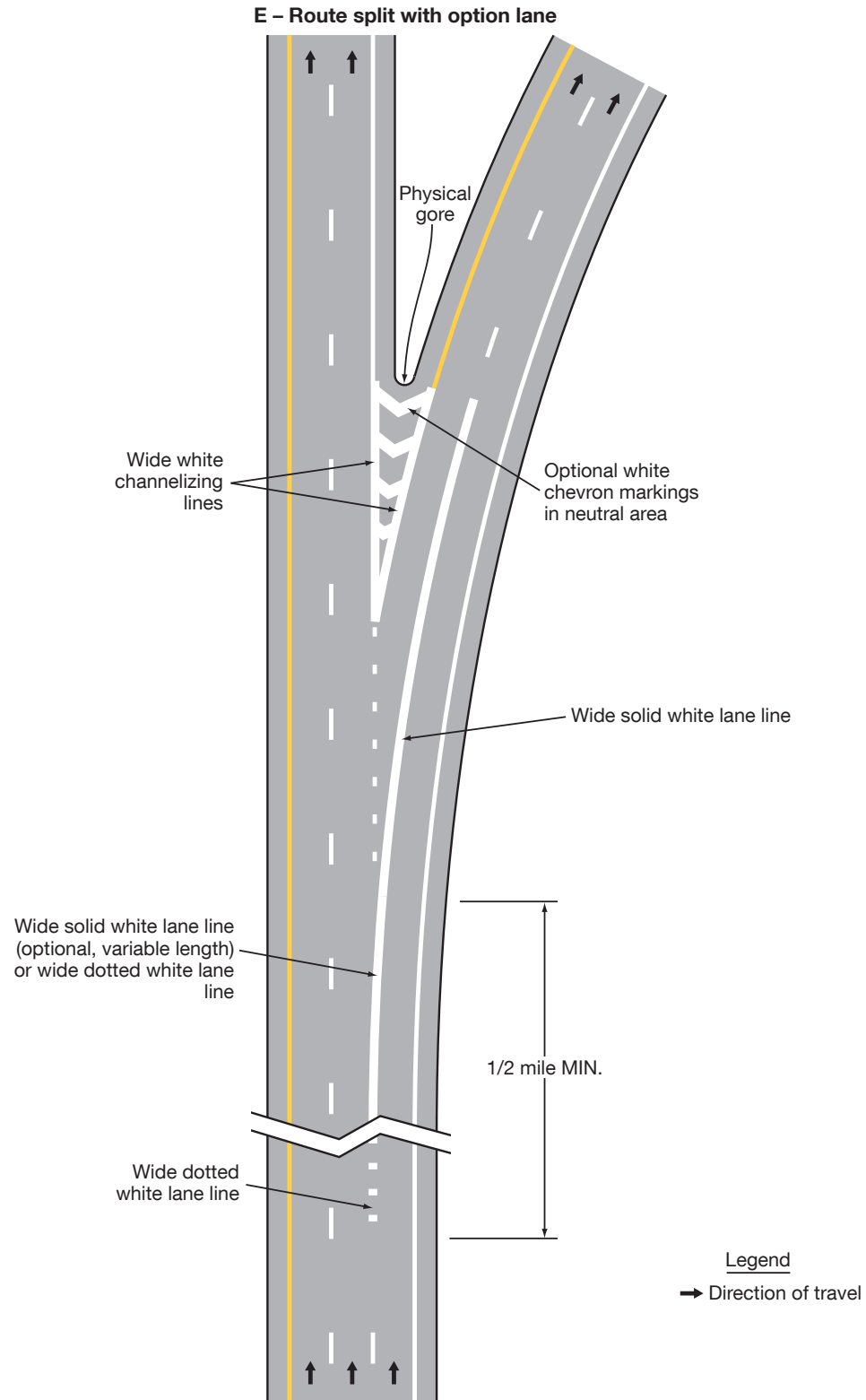
Figure 3B-11. Examples of Applications of Freeway and Expressway Lane-Drop Markings (Sheet 5 of 6)
