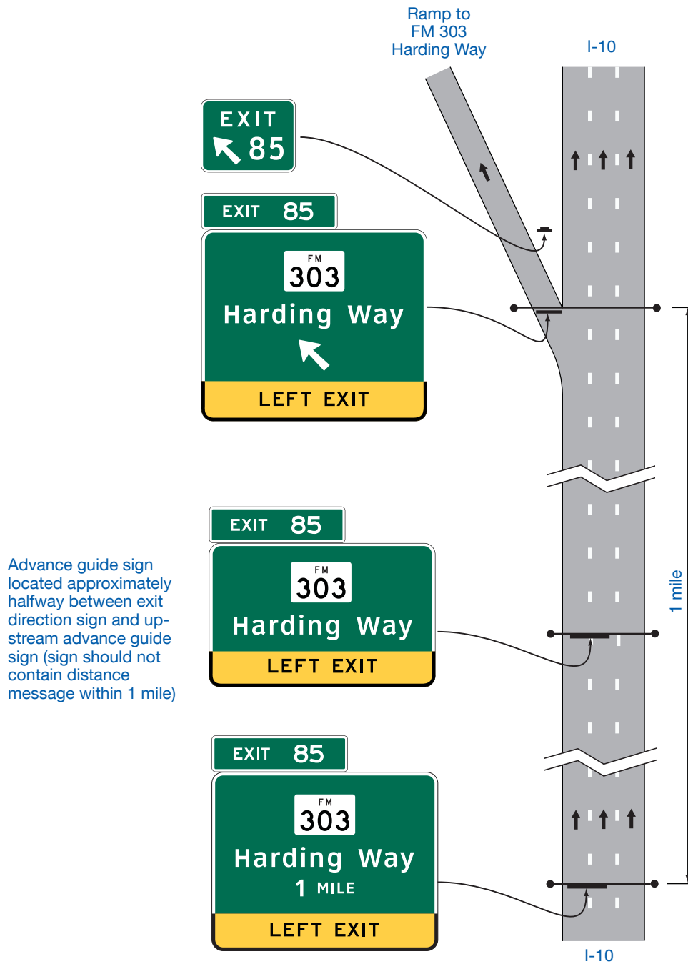
Figure 2E-19A. (TX) Guide Signs for a Single-Left Lane Exit
