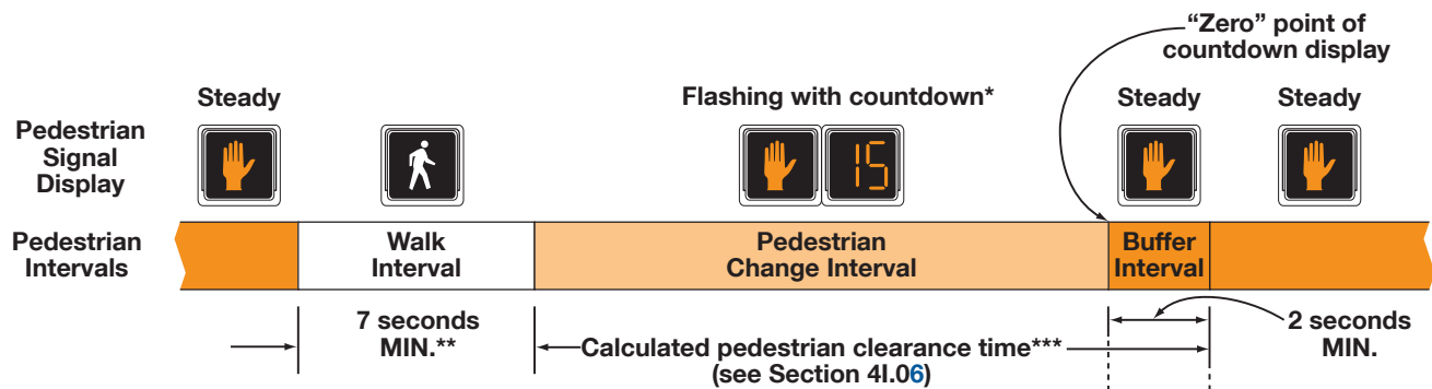
Figure 4I-4. Pedestrian Intervals
