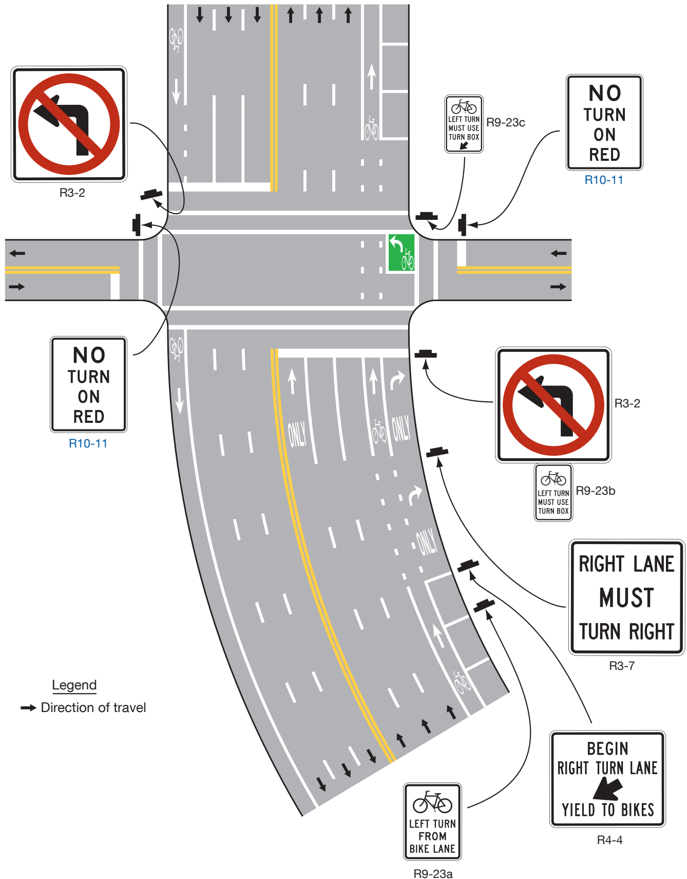
Figure 9B-5. Example of Two-Stage Bicycle Turn Box Where Use is Mandatory
