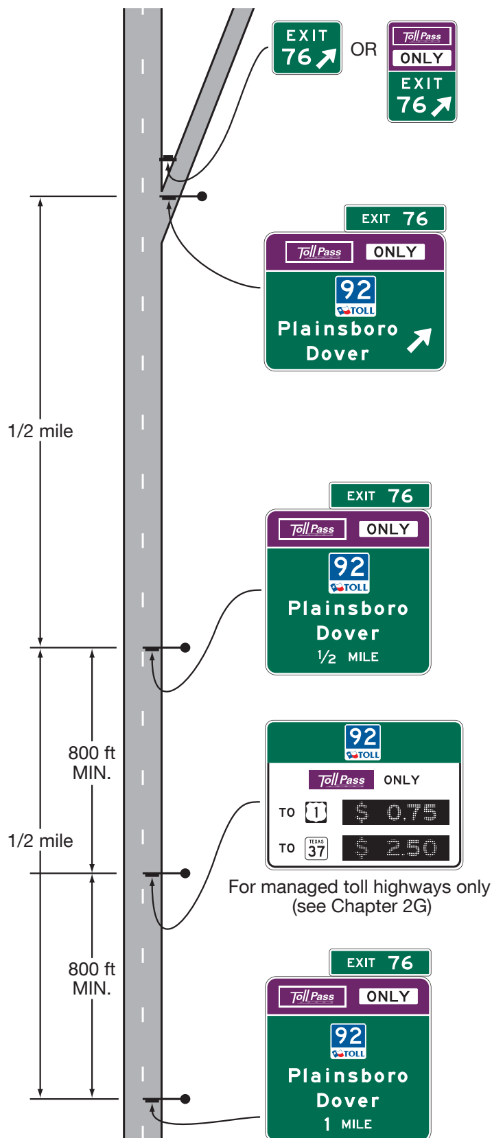
Figure 2F-12. Examples of Guide Signs for the Entrance to a Toll Highway on which Tolls are Collected Electronically Only (Sheet 2 of 3)
