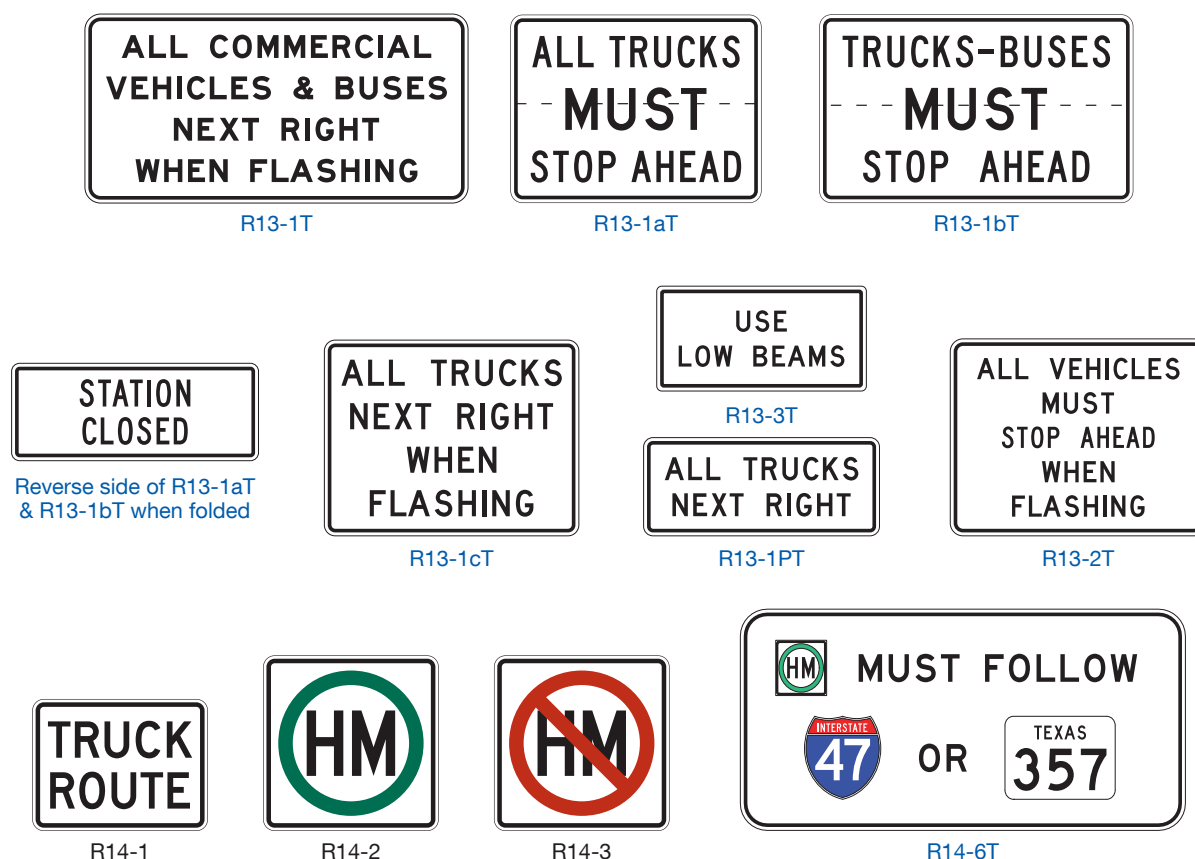
Figure 2B-31. Truck Signs
