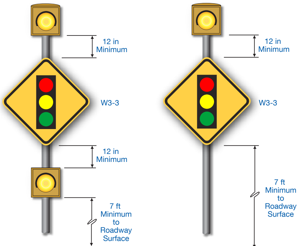
Figure 4S-1A. (TX) Typical Warning Sign and Hazard Identification Beacon
