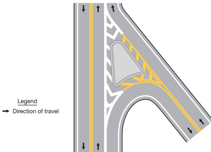
Figure 3J-5. Example of Optional Chevron and Diagonal Pavement Markings at a Raised Island
