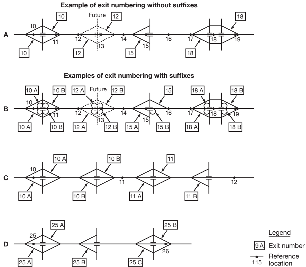
Figure 2E-3. Examples of Interchange Exit Numbering
