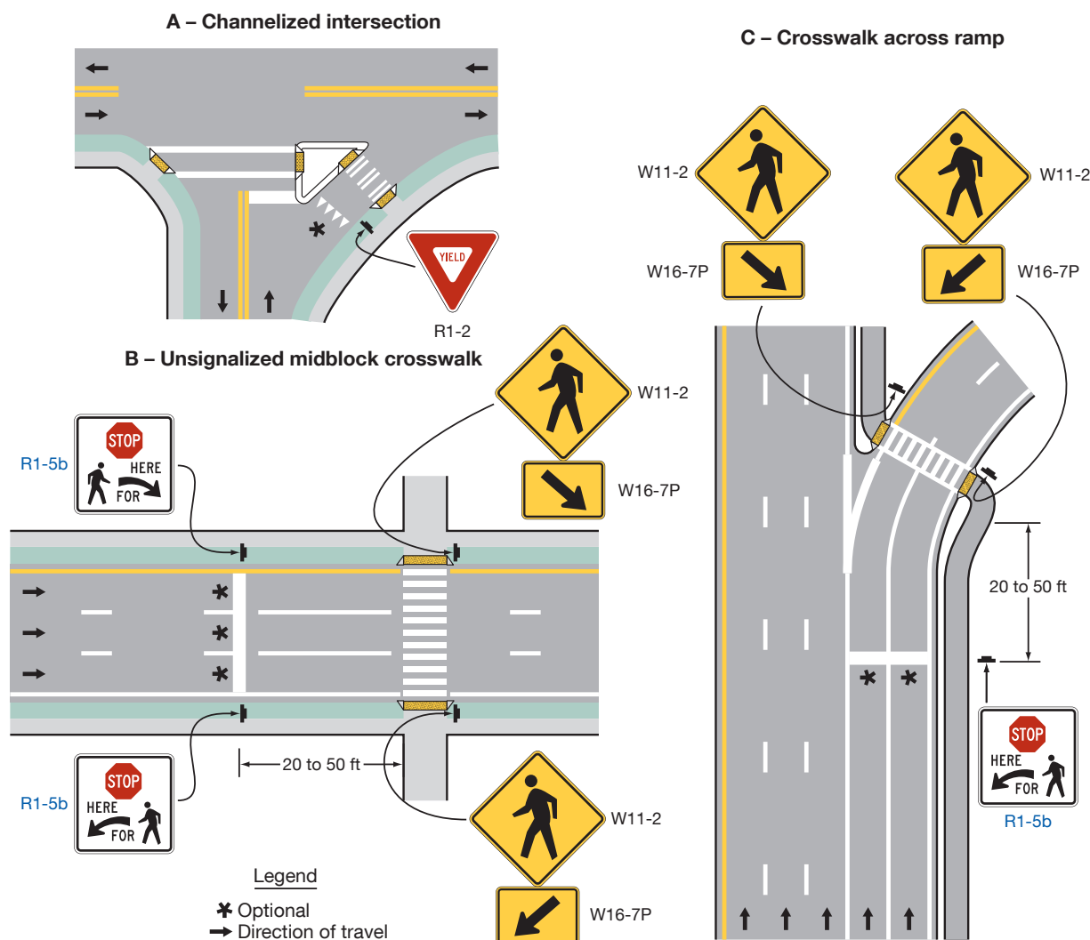
Figure 3B-16. Examples of Yield and Stop Line Applications
