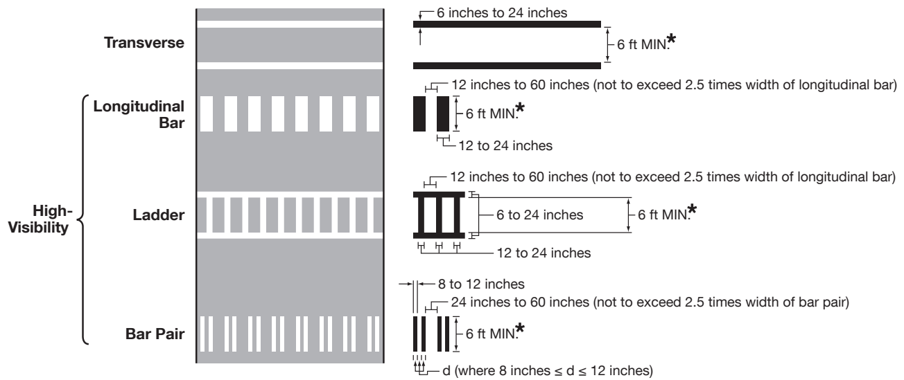
Figure 3C-1. Crosswalk Markings
