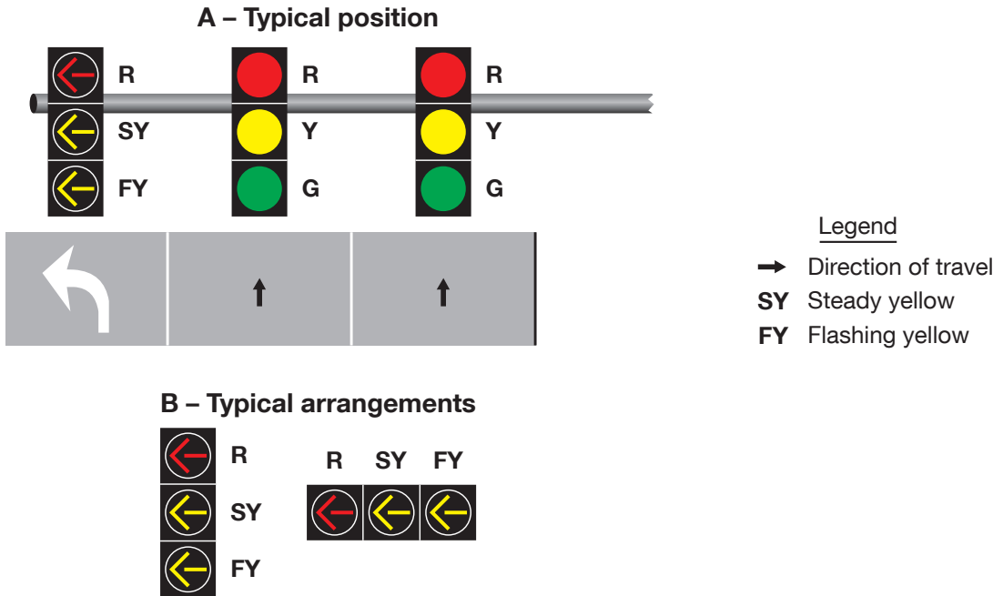
Figure 4F-2. Typical Position and Arrangements of Separate Signal Faces with Flashing Yellow Arrow for Permissive Only Mode Left Turns
