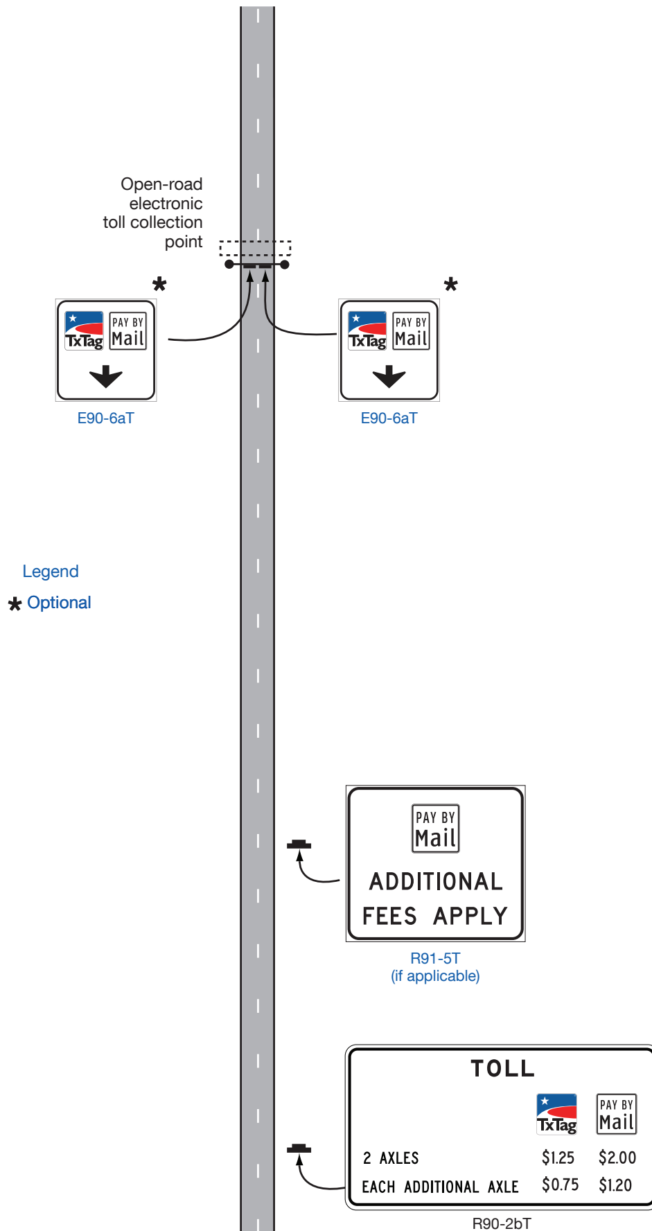
Figure 2F-15A. (TX) Examples of Signage for an Open-Road Electronic Toll Collection Point
