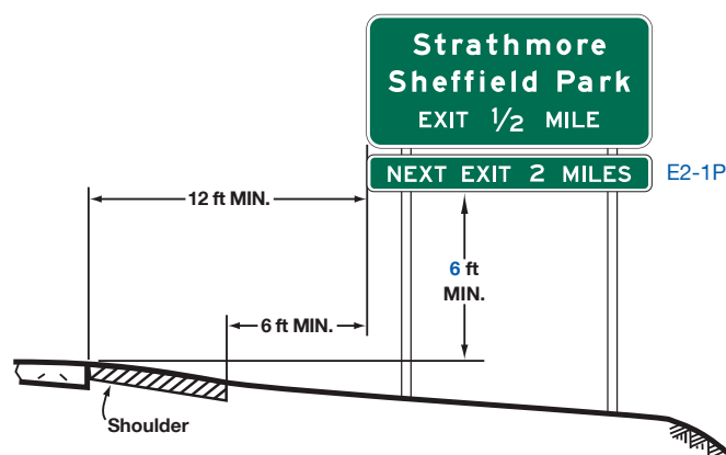
G – Freeway or expressway sign with supplemental plaque
