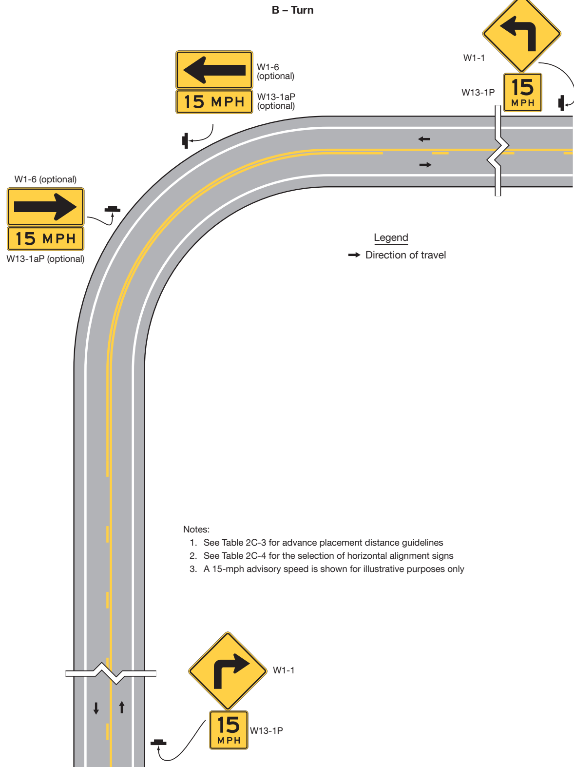
Figure 2C-2. Examples of Warning Signs for Changes in Horizontal Alignment (Sheet 2 of 2)
