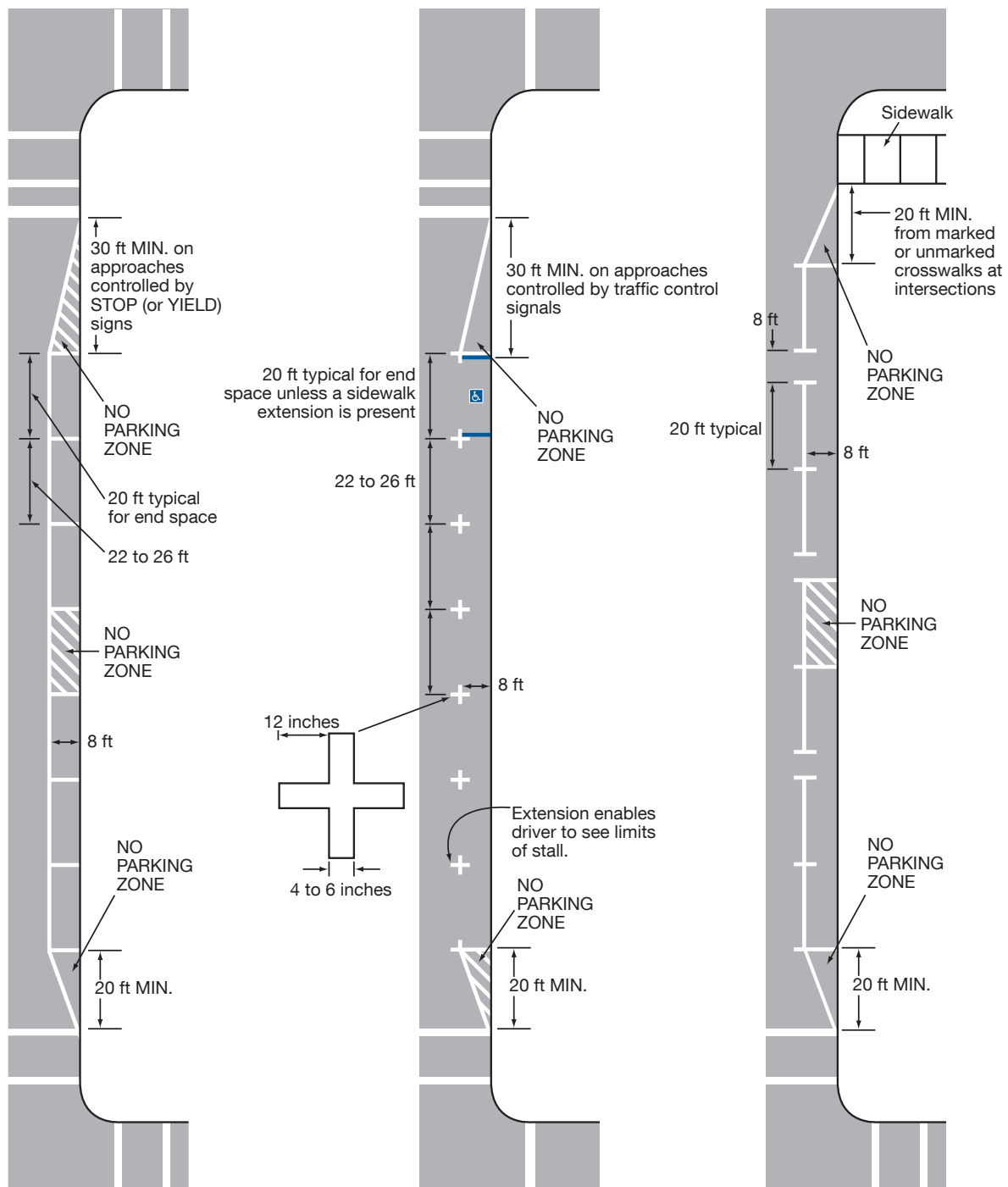
Figure 3B-23. Examples of Parking Space Markings
