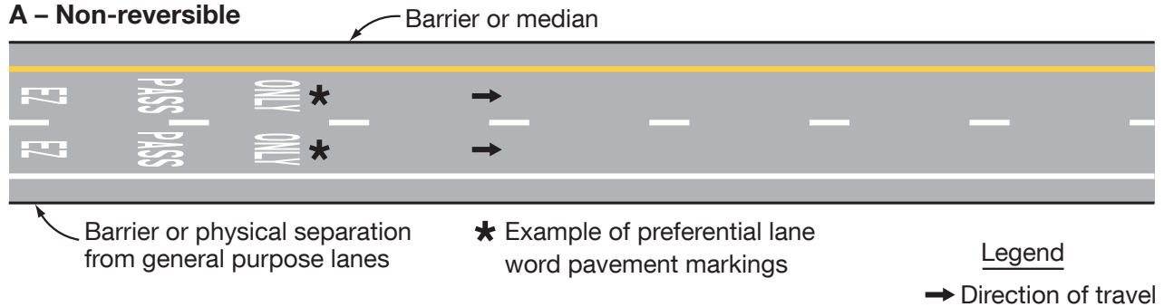
Figure 3E-1. Markings for Barrier-Separated Preferential Lanes
