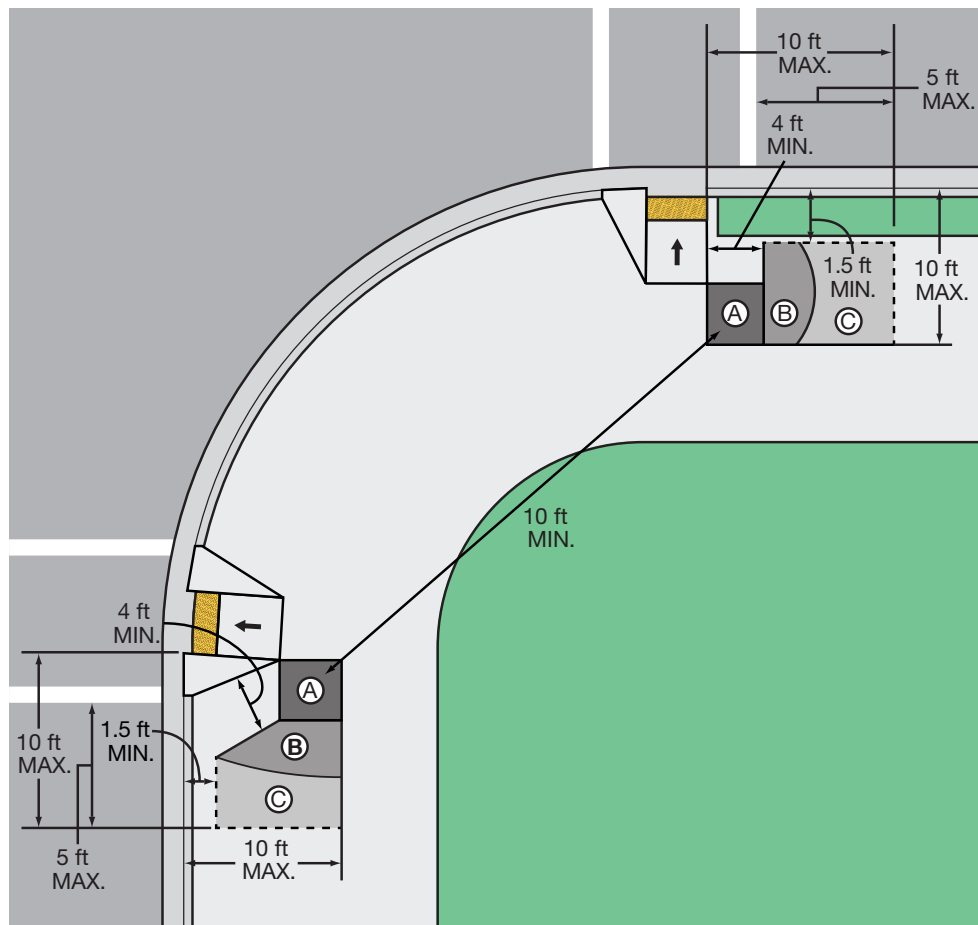
Figure 4I-2. Preferred Push Button Location Area
