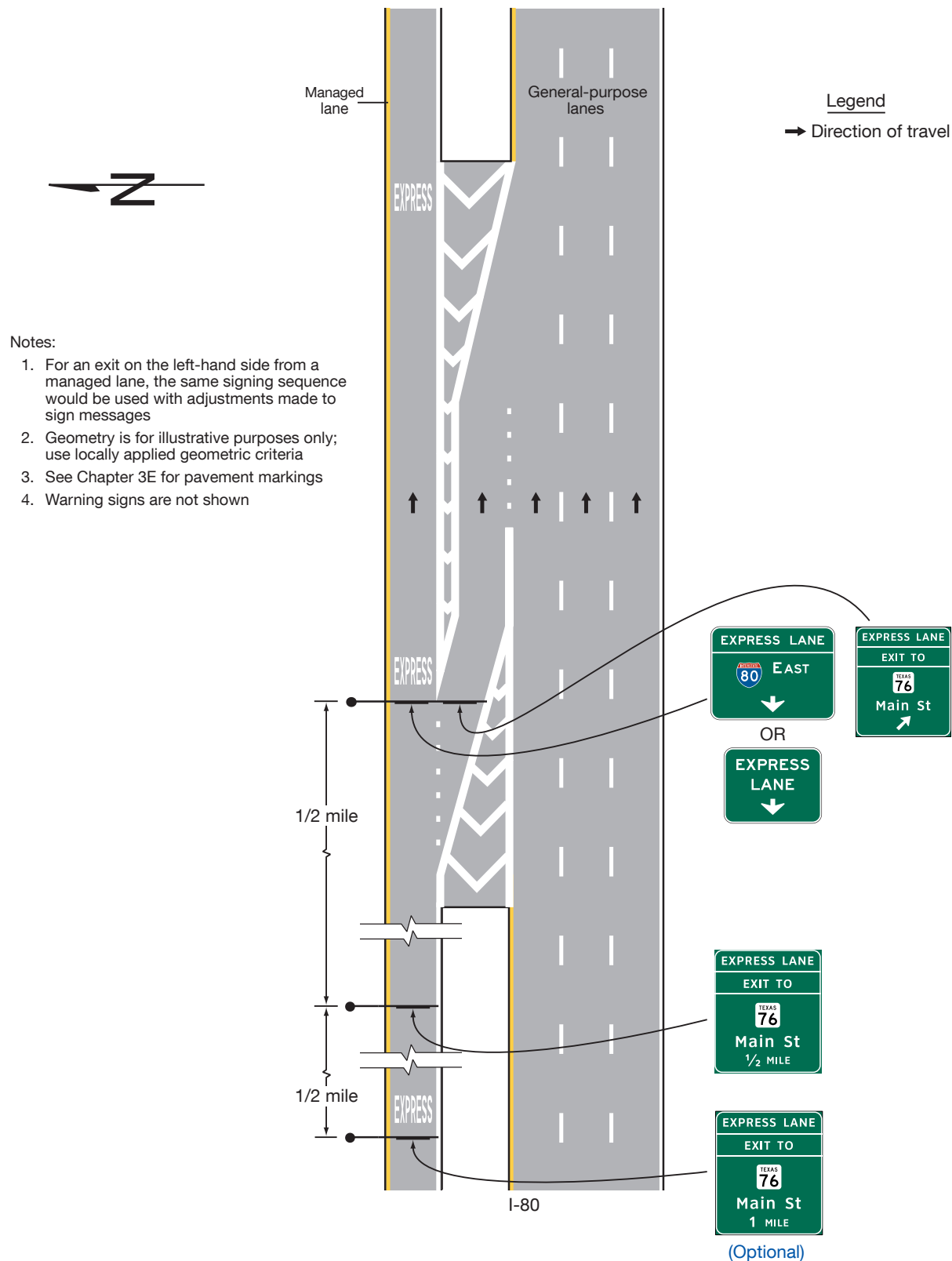
Figure 2G-27. Examples of Guide Signs for an Intermediate Egress from a Barrier-Separated or Buffer-Separated Managed Lane
