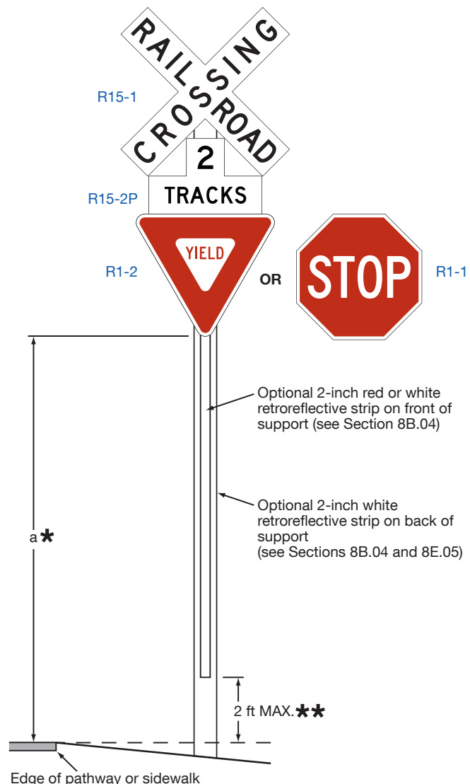
Figure 8E-5. Example of Crossbuck Assembly at a Pathway or Sidewalk Grade Crossing
