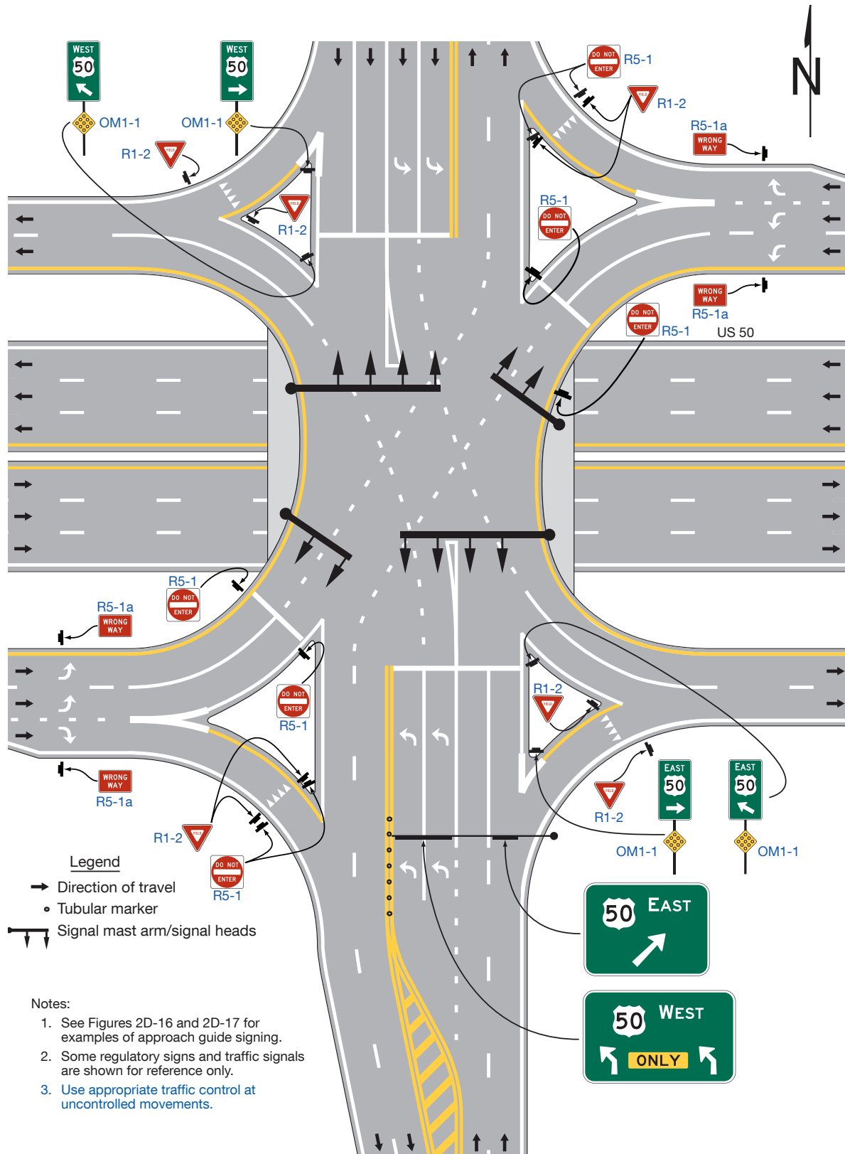
Figure 2D-22. Example of Crossroad Intersection Guide Signs for a Single-Point Urban Interchange
