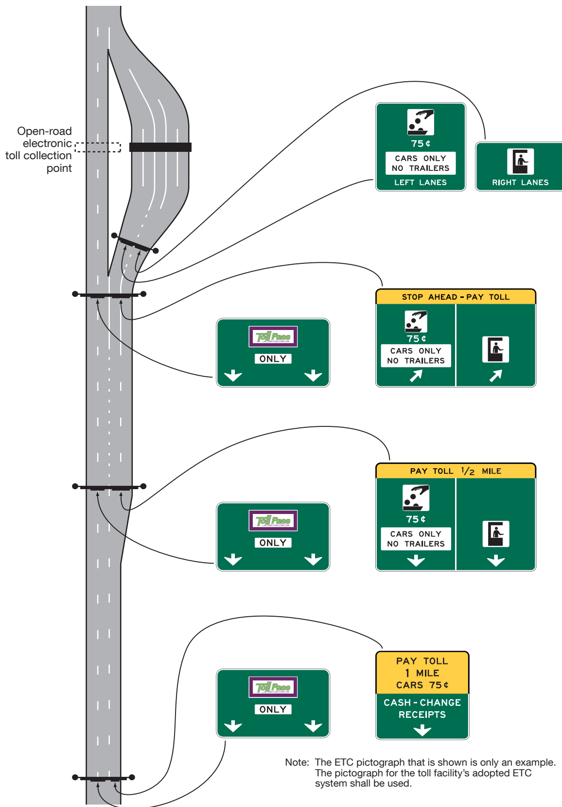
Figure 2F-15. Examples of Guide Signs for a Mainline Toll Plaza on a Diverging Alignment from Open-Road ETC Lanes
