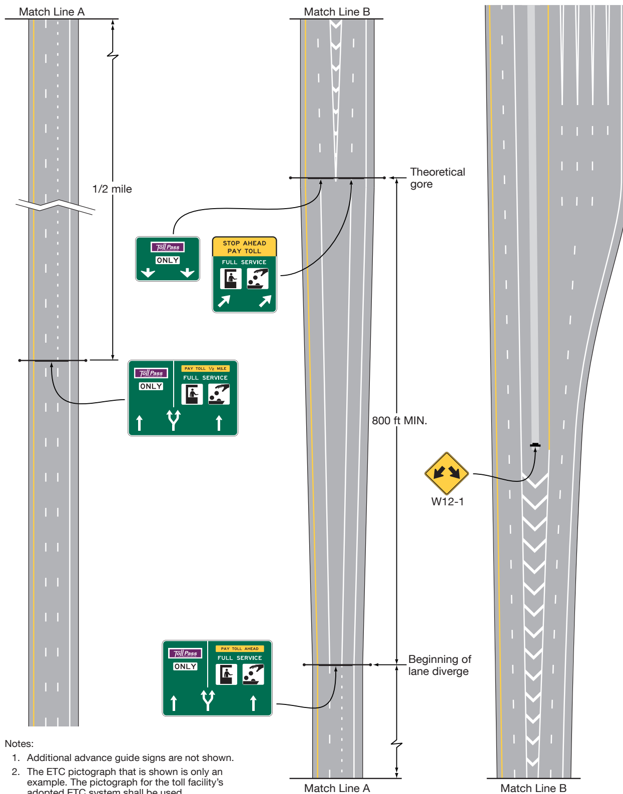
Figure 2F-11. Examples of Guide Signs for a Split with an Option Lane for a Mainlane Toll Plaza on a Diverging Alignment from Open-Road ETC Lanes
