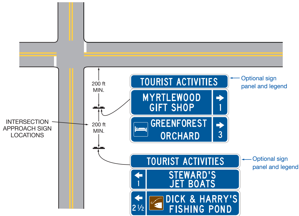
Figure 2K-2. Examples of Tourist-Oriented Directional Signs on an Intersection Approach
