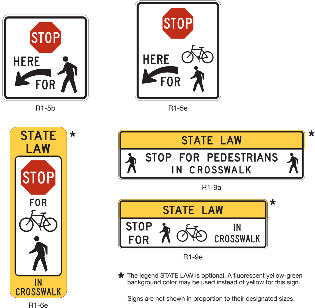
Figure 2B-2. Unsignalized Pedestrian Crosswalk Signs
