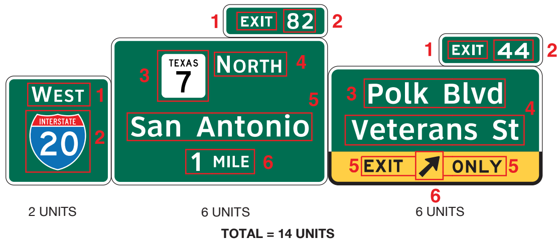
Figure 2E-47A. (TX) Example of Guide Sign Information Units
