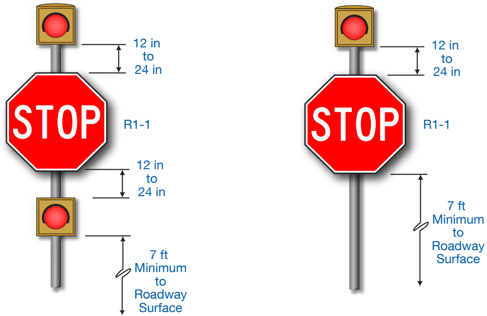
Figure 4S-2A. (TX) Typical Stop Sign Beacon Installation at Intersection
