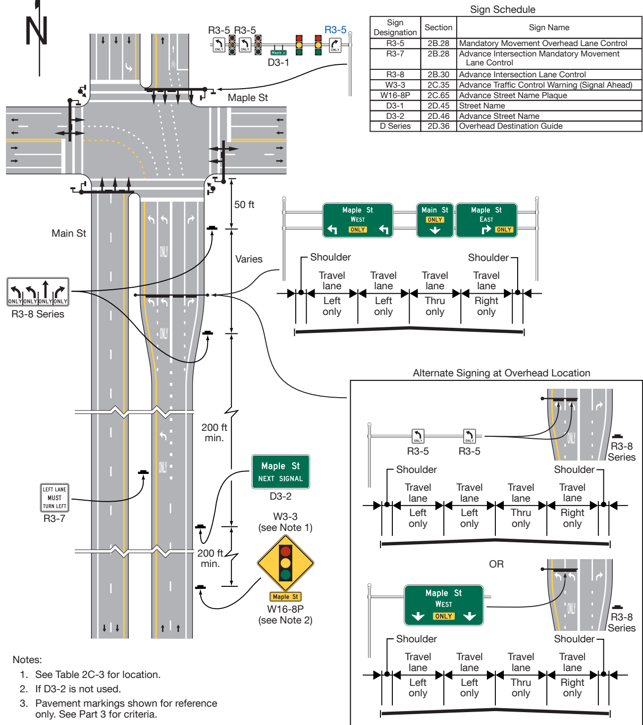
Figure 2A-4. Relative Locations of Regulatory, Warning, and Guide Signs On an Intersection Approach (Sheet 3 of 4)
