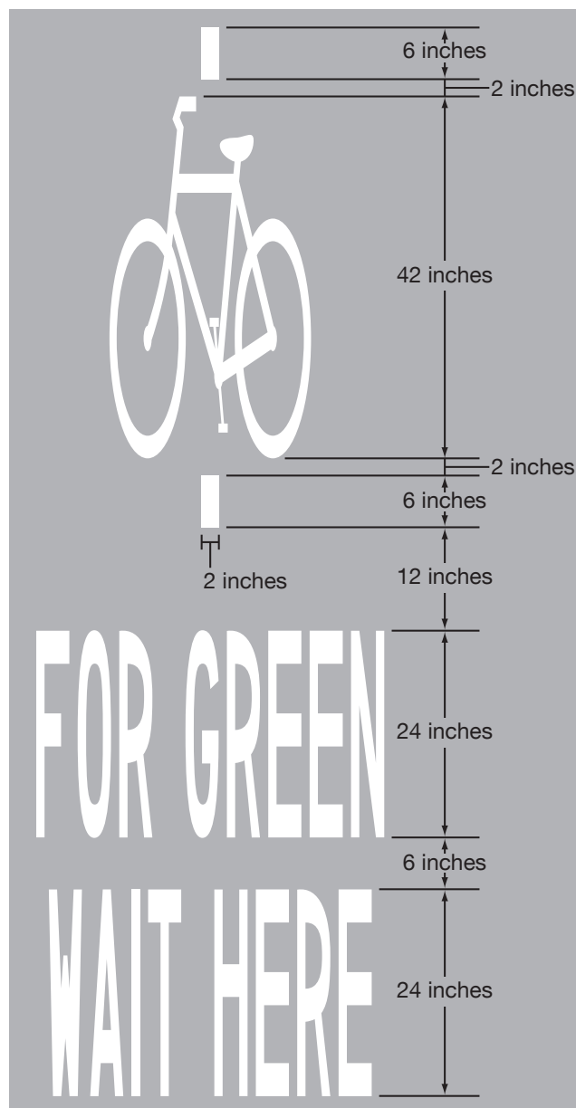
Figure 9E-16. Bicycle Detector Pavement Marking
