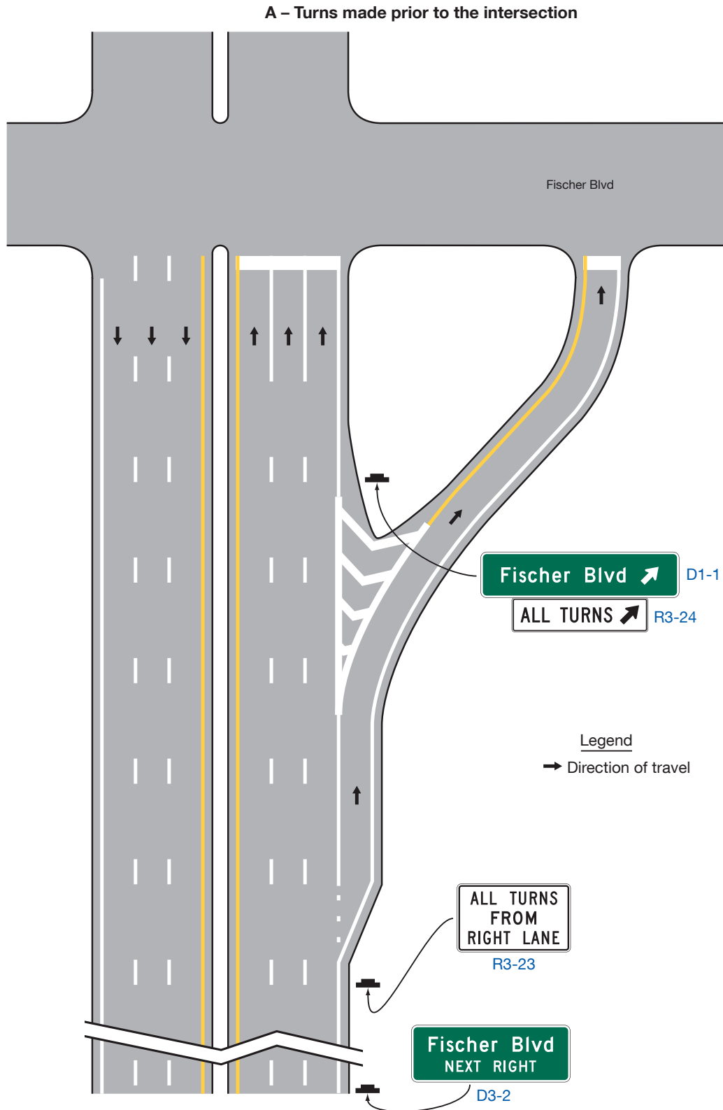
Figure 2B-9. Examples of Applications of Jughandle Regulatory and Guide Signing (Sheet 1 of 3)
