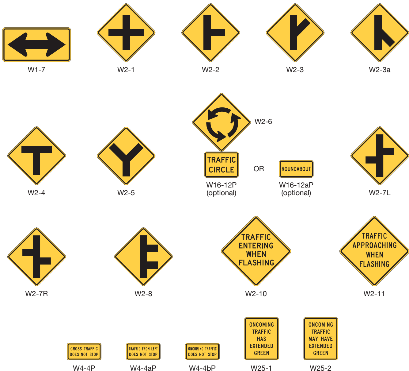
Figure 2C-10. Intersection Warning Signs and Plaques
