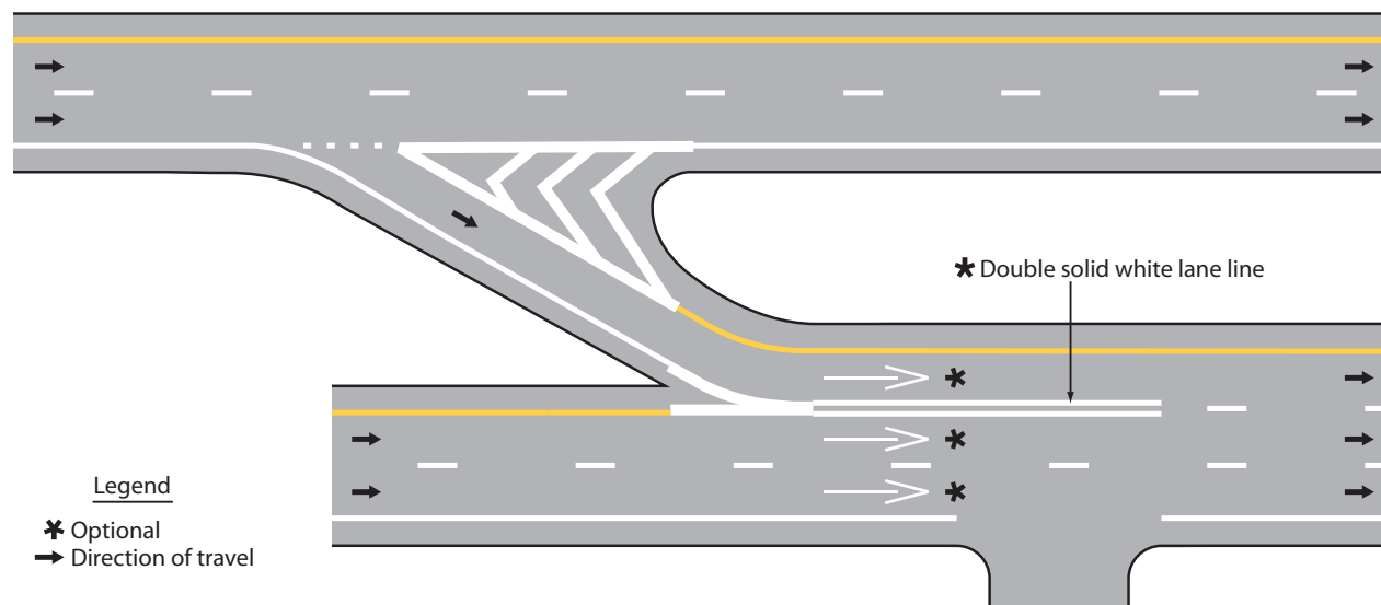
Figure 3B-8. Example of Double Solid White Line Used to Prohibit Lane Changing
