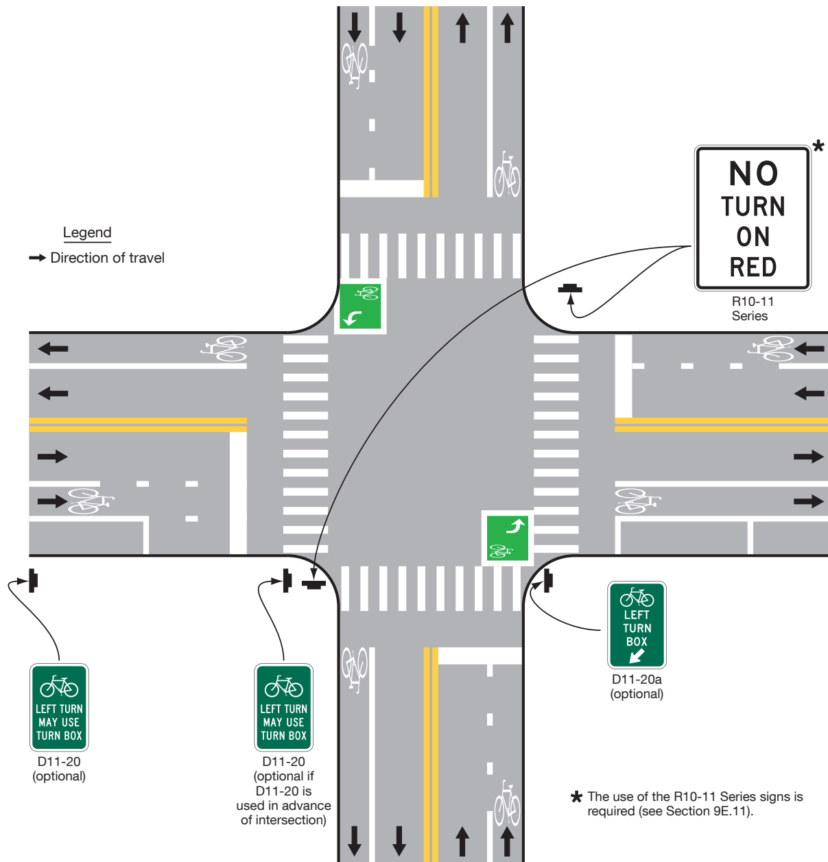
Figure 9D-7. Example of Two-Stage Bicycle Turn Box Where Use is Optional
