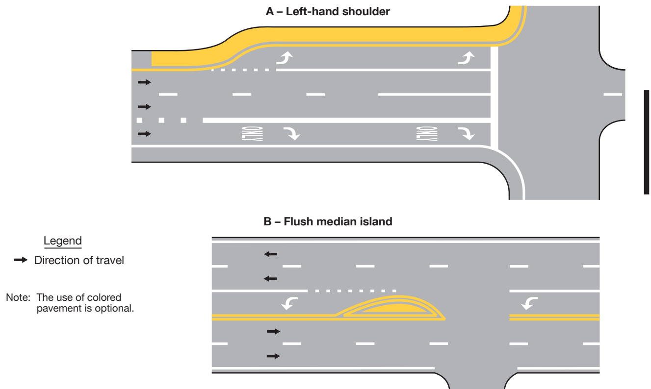
Figure 3H-2. Examples of Yellow-Colored Pavement Applications
