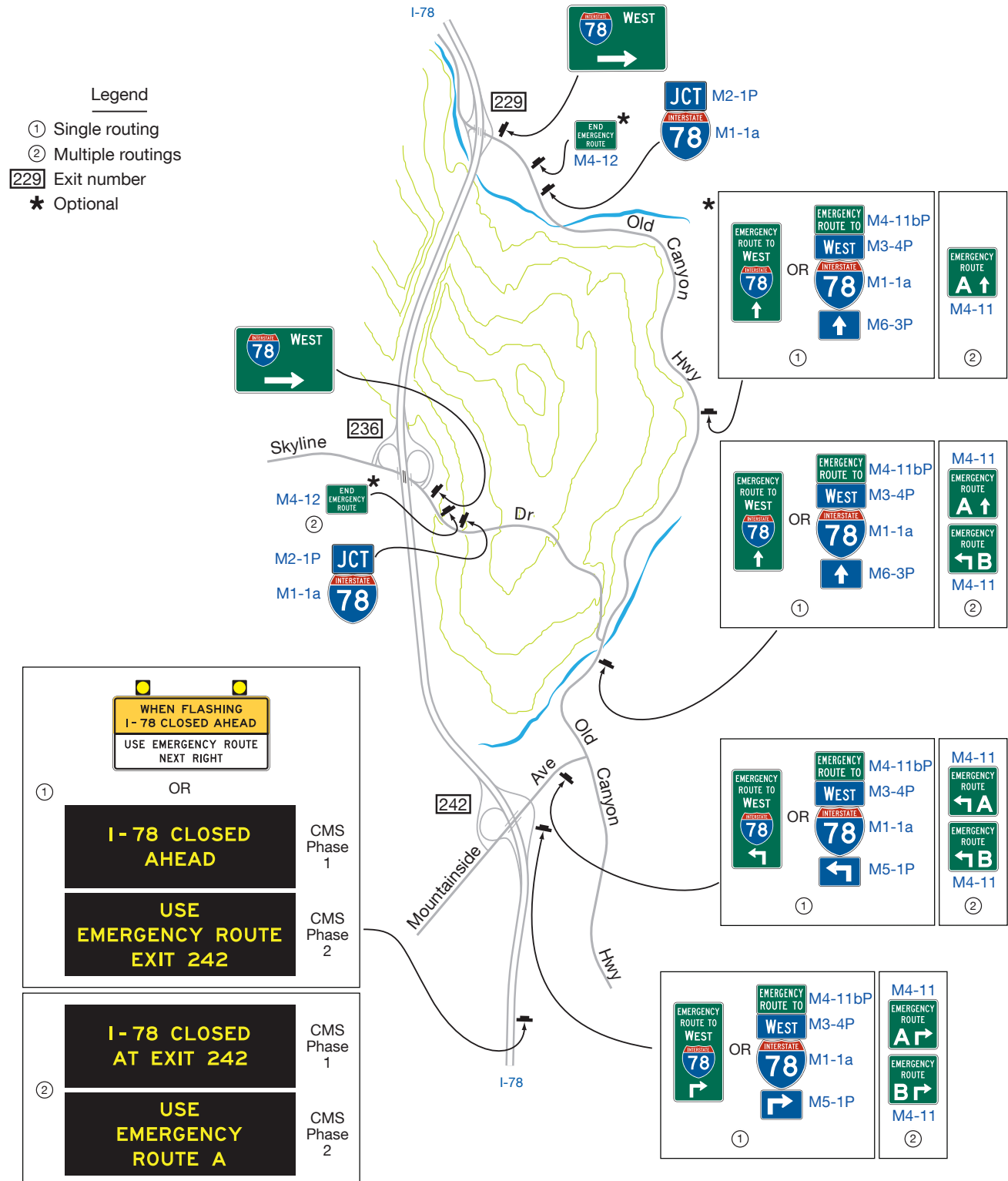
Figure 2D-38. Example of Permanent Guide Signing for Rerouting Because of Recurring Events
