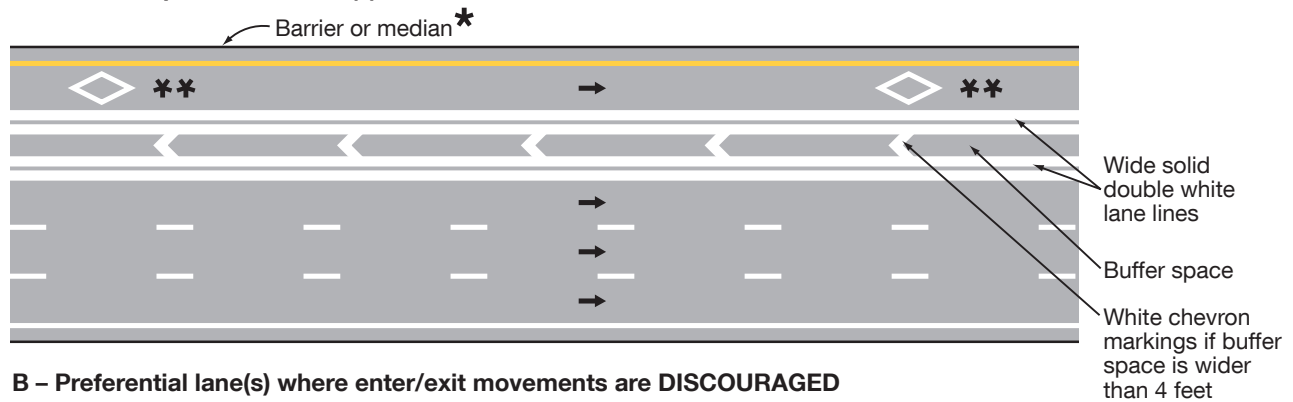
Figure 3E-2. Markings for Buffer-Separated Preferential Lanes (Sheet 1 of 2)
