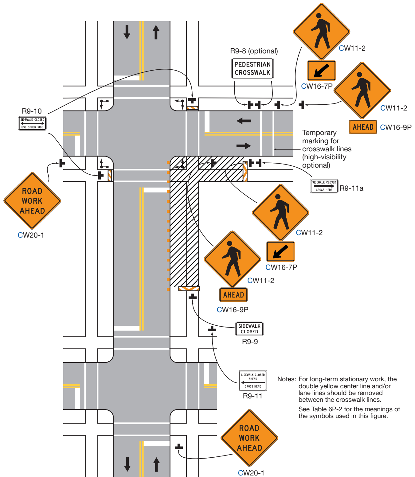
Figure 6P-29. Crosswalk Closures and Pedestrian Detours (TA-29)
