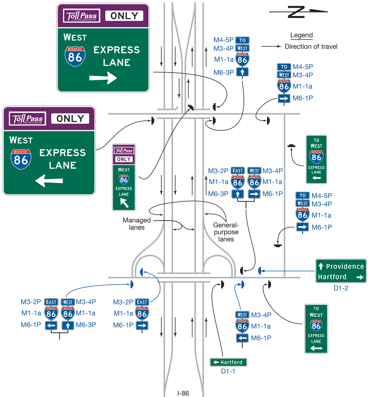
Figure 2G-30. Examples of Guide Signs for a Direct Entrance Ramp to a Priced Managed Lane and Trailblazing to a Nearby Entrance to the General-Purpose Lanes
