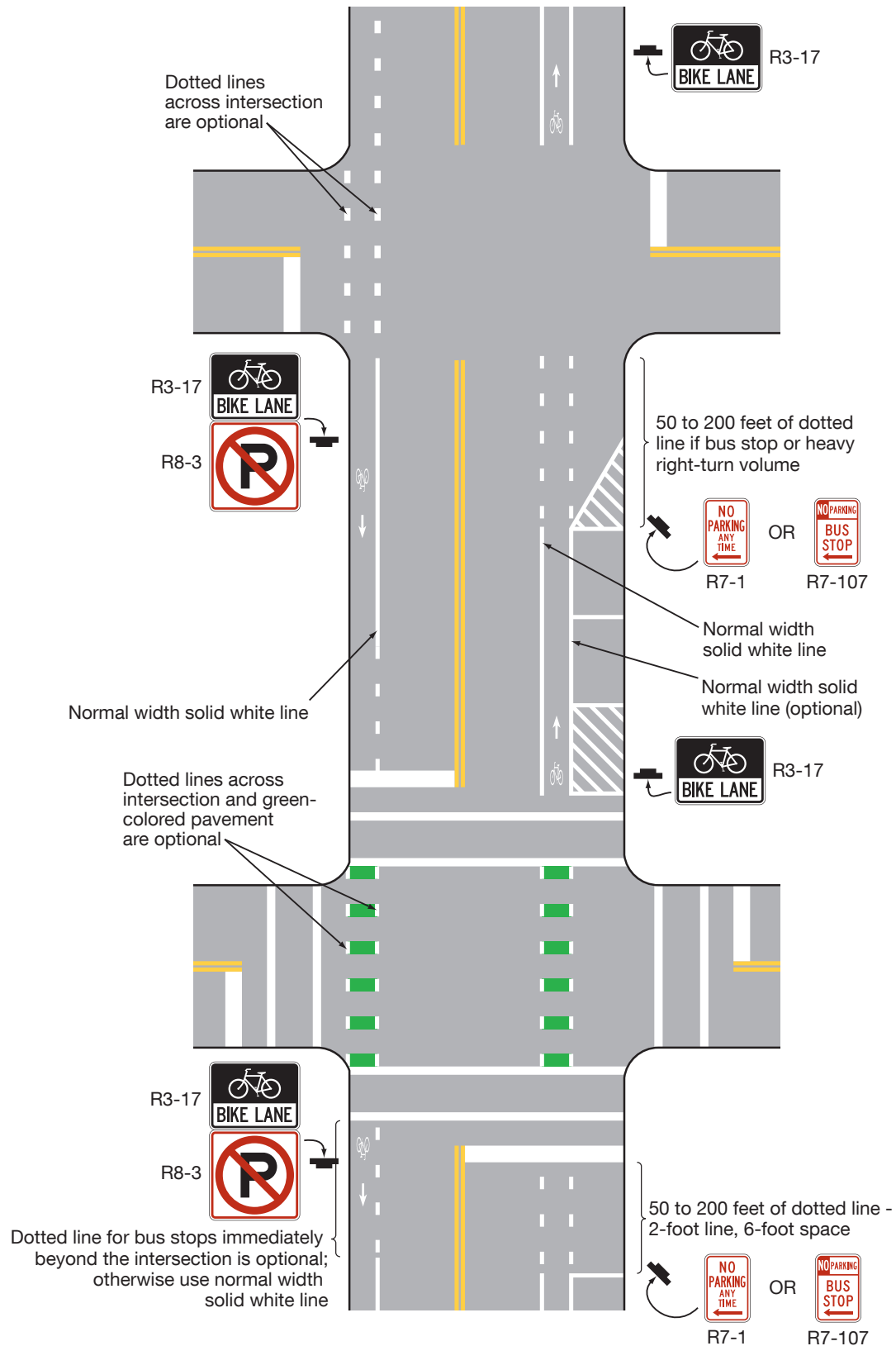
Figure 9E-2. Example of Pavement Markings for Bicycle Lanes on a Two-Way Street
