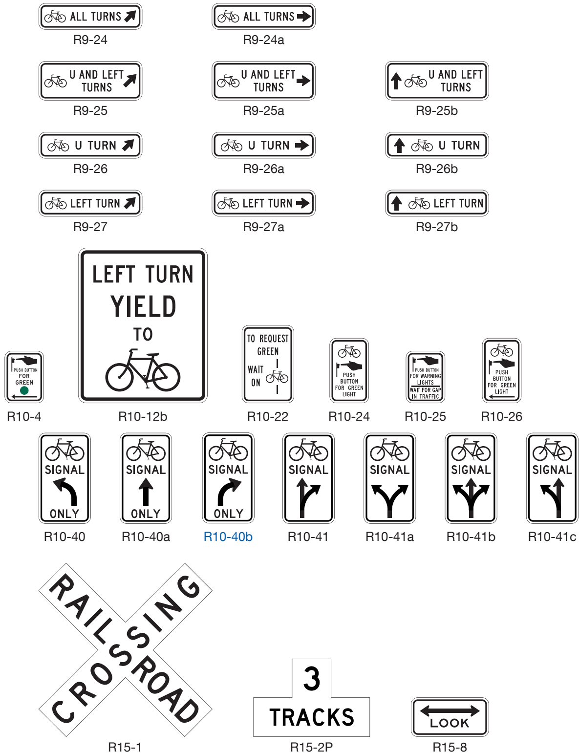
Figure 9B-1. Regulatory Signs and Plaques for Bicycle Facilities (Sheet 2 of 2)
