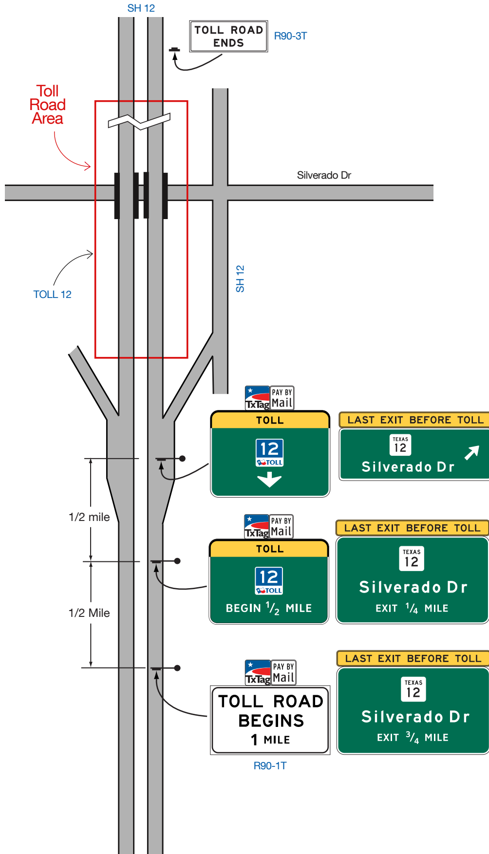
Figure 2F-13A. (TX) Non-Toll Roadway Converts to a Toll Roadway
