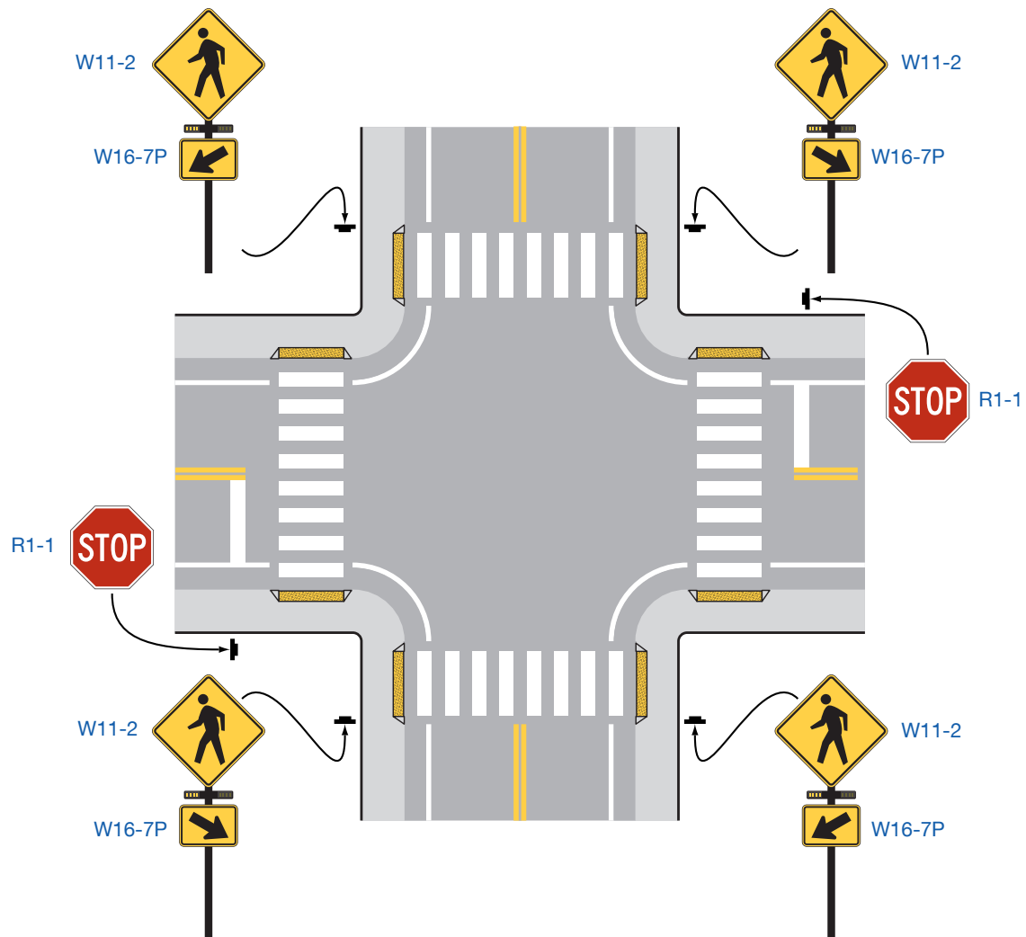
Figure 4L-1. Example of RRFBs at Uncontrolled, Marked Crosswalks at an Intersection
