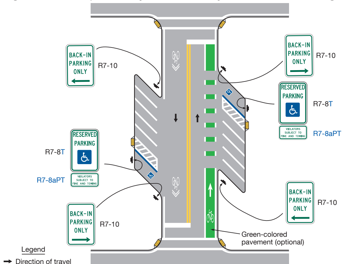
Figure 9B-3. Examples of Bicycle Facilities Adjacent to Back-In Parking
