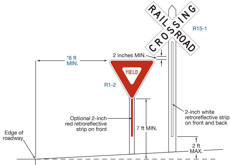
Figure 8B-3. Crossbuck Assembly with a YIELD or STOP Sign on a Separate Sign Support
