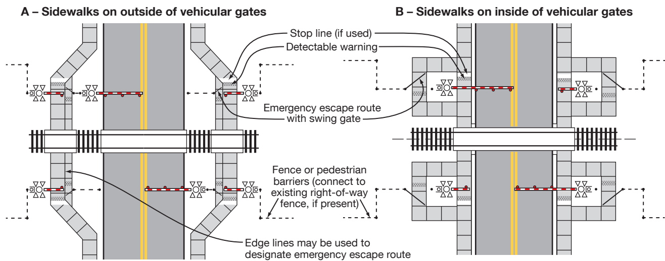
Figure 8E-9. Example of Active Traffic Control Systems with Automatic Pedestrian Gates and Swing Gates at a Sidewalk Grade Crossing
