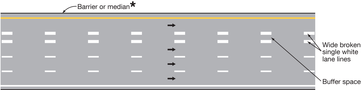
Figure 3E-2. Markings for Buffer-Separated Preferential Lanes (Sheet 2 of 2)
