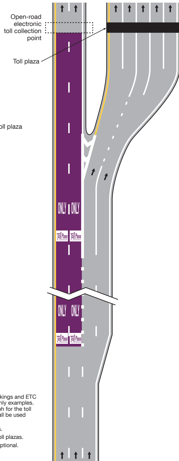
Figure 3H-6. Examples of Purple-Colored Pavement Applications (Sheet 2 of 2)
