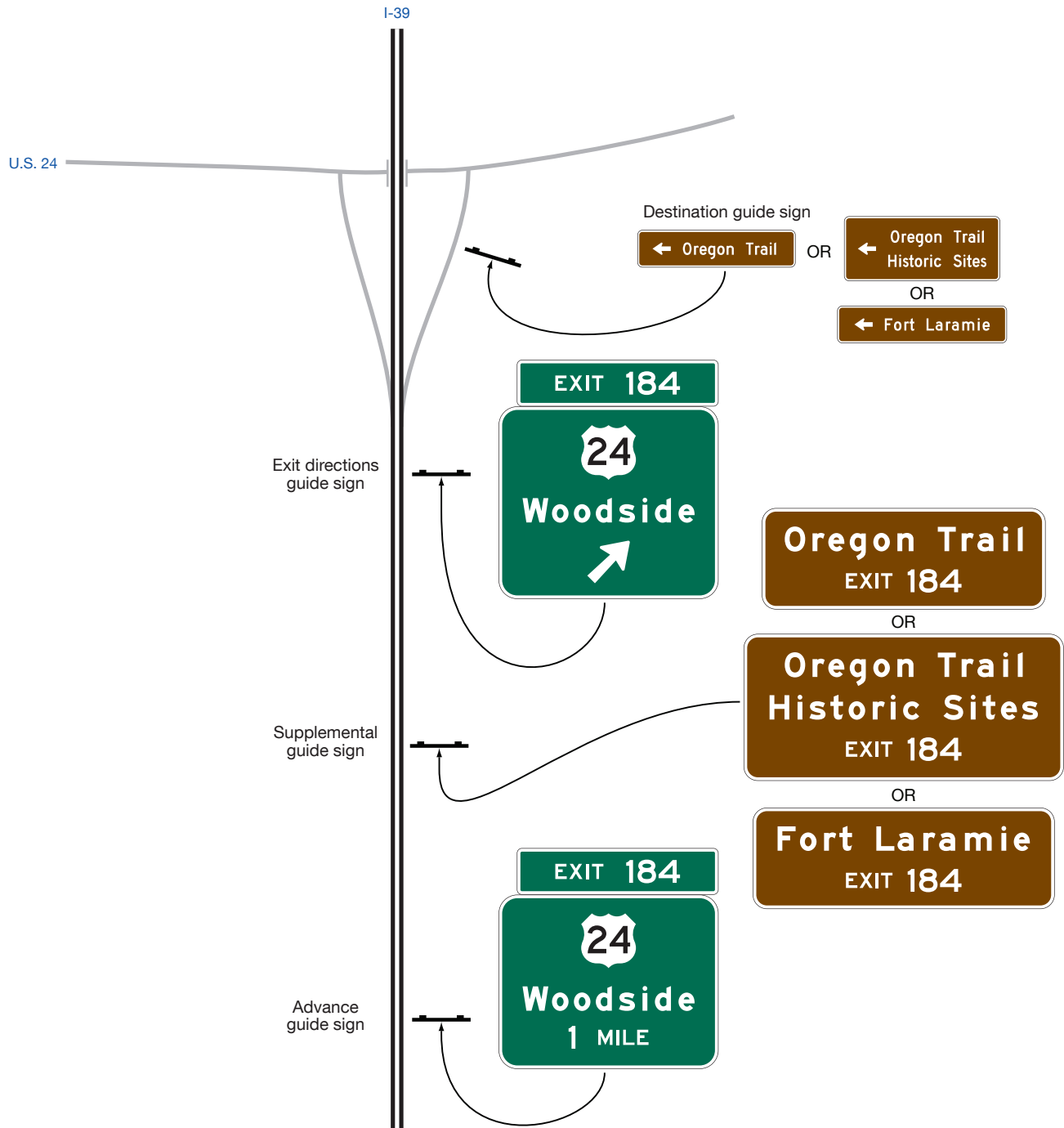
Figure 2D-36. Example of Historic Trails Signing from an Expressway or Freeway
