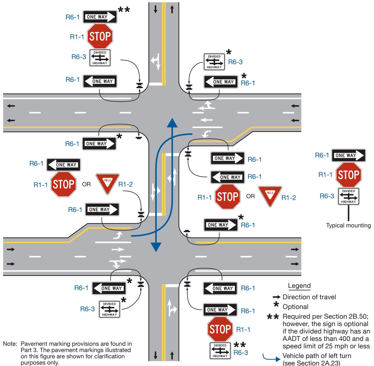
Figure 2B-19. ONE WAY Signing for Divided Highway Crossings that Function as Two Separate Intersections
