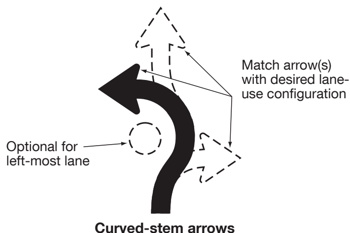
Figure 2B-5. Intersection Lane Control Sign Arrow Options for Roundabouts
