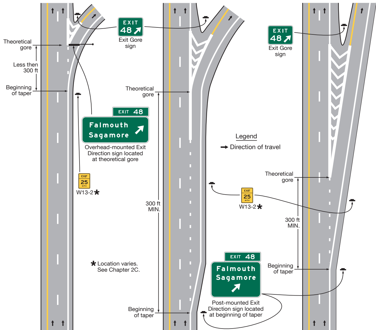
Figure 2E-13. Exit Direction Sign Placement
