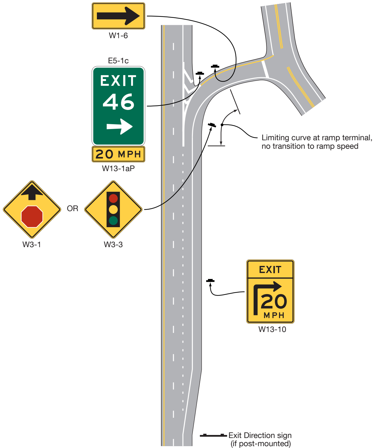
Figure 2C-3. Examples of Exit Ramp Advisory Speed and Other Warning Signs (Sheet 5 of 5)
