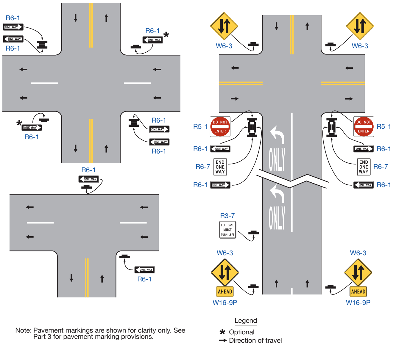
Figure 2B-18. Locations of ONE WAY Signs
