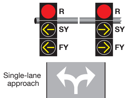
Figure 4F-15. Signal Indications for Approaches with Combined Left-Turn/Right-Turn Lane and No Through Movement (Sheet 3 of 3)
