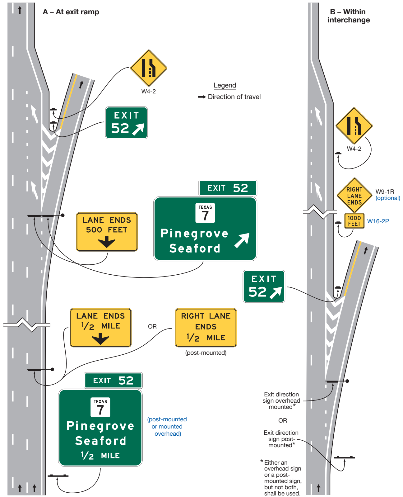
Figure 2E-23. Examples of Signing for Mainline Terminations within an Interchange
