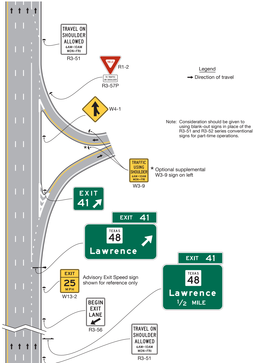
Figure 2G-32. Examples of Signing for Part-Time Travel on Shoulder (Sheet 2 of 4)
