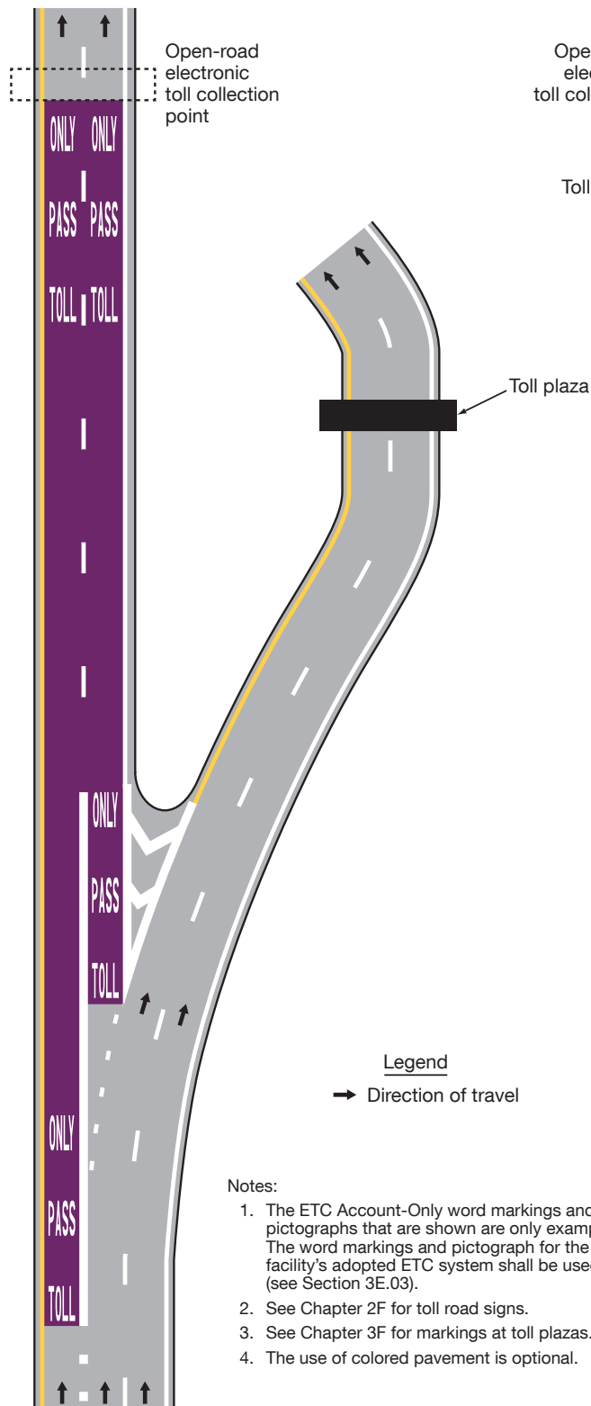
Figure 3H-6. Examples of Purple-Colored Pavement Applications (Sheet 2 of 2)
