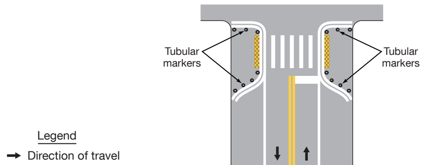
Figure 3J-6. Examples of Sidewalk Extensions Designated by Pavement Markings and Channelization
