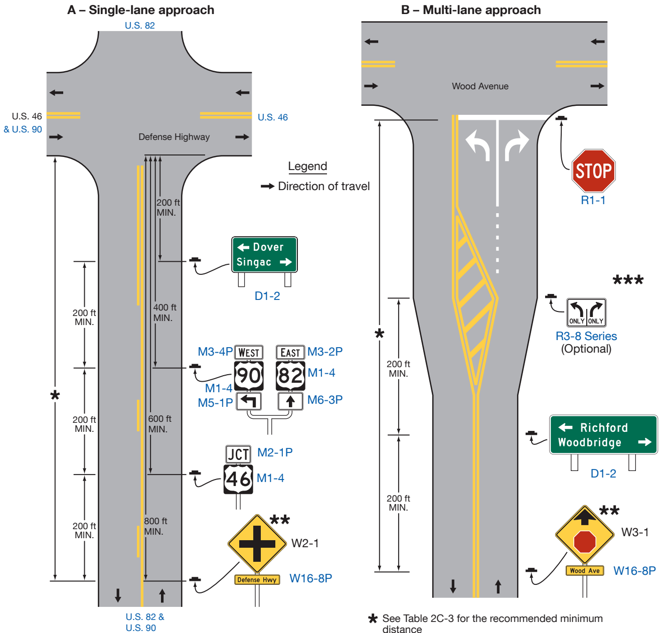
Figure 2A-4. Relative Locations of Regulatory, Warning, and Guide Signs On an Intersection Approach (Sheet 1 of 4)
