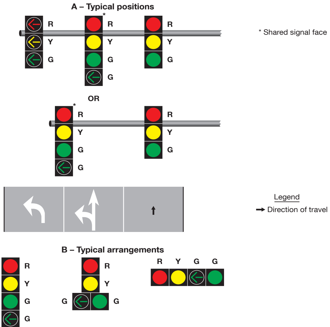
Figure 4F-4. Typical Positions and Arrangements of Shared Signal Faces for Protected Only Mode Left Turns
