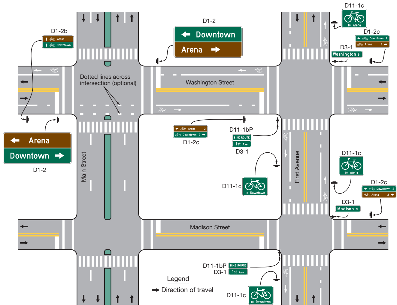
Figure 9D-3. Examples of Bicycle Route Guide Signing
