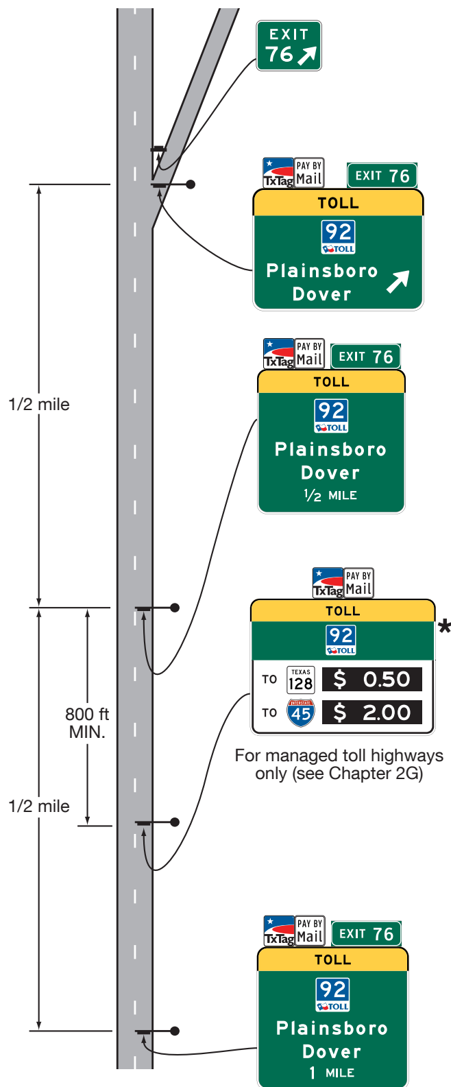
Figure 2F-12. Examples of Guide Signs for the Entrance to a Toll Highway on which Tolls are Collected Electronically Only (Sheet 3 of 3)
