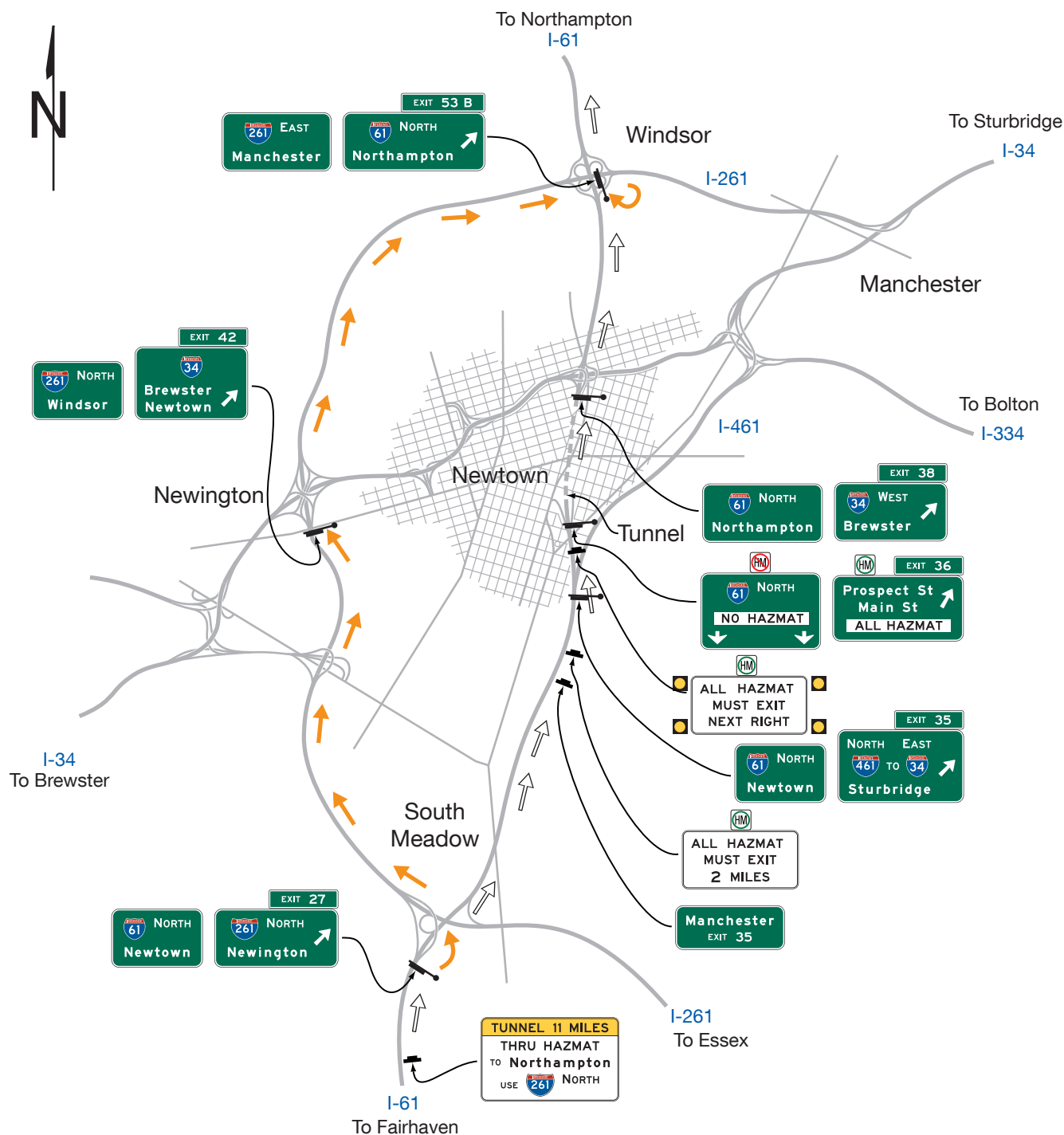
Figure 2E-62. Example of Signing for Route Diversion by Vehicle Class
