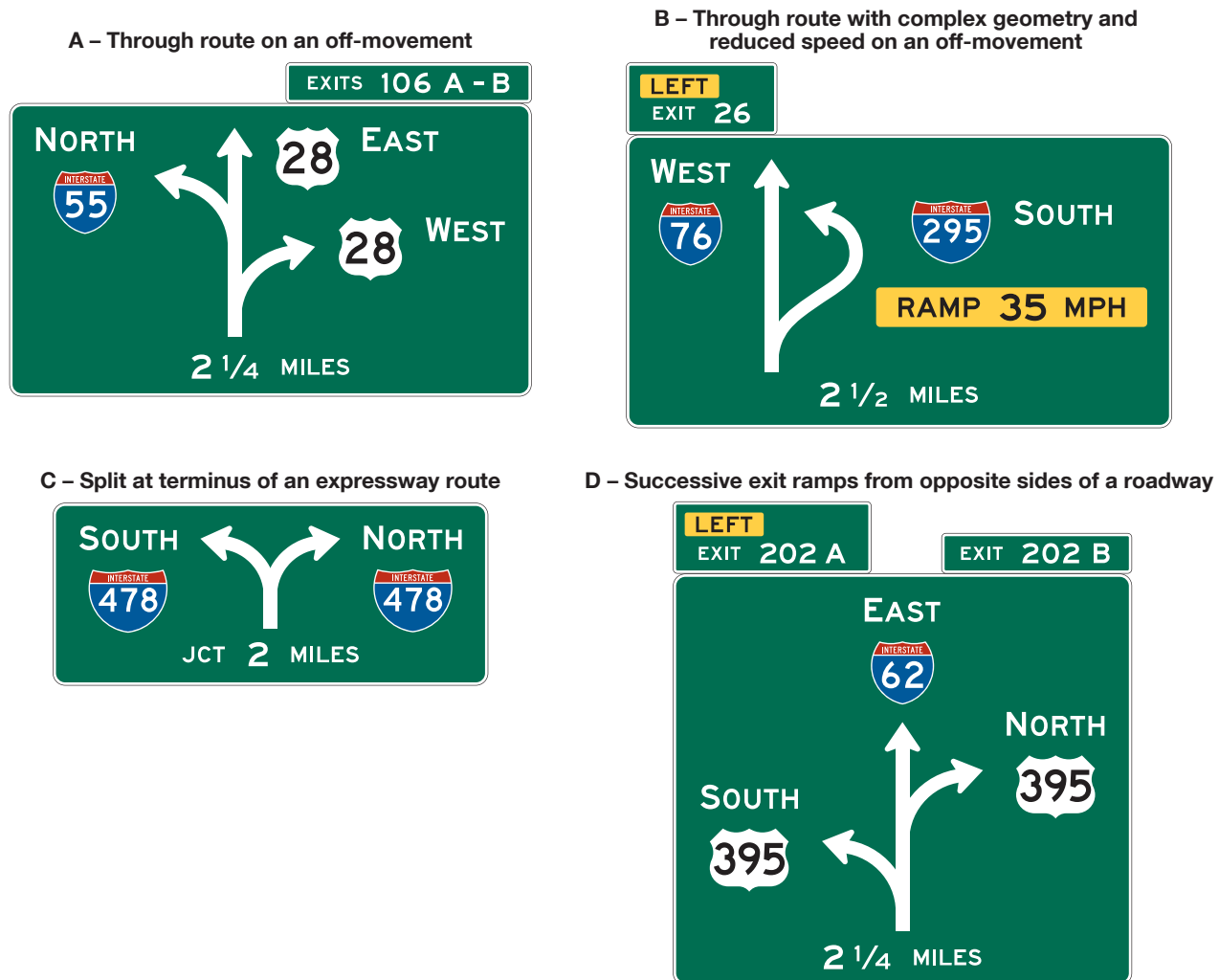
Figure 2E-41. Examples of Diagrammatic Advance Guide Signs
