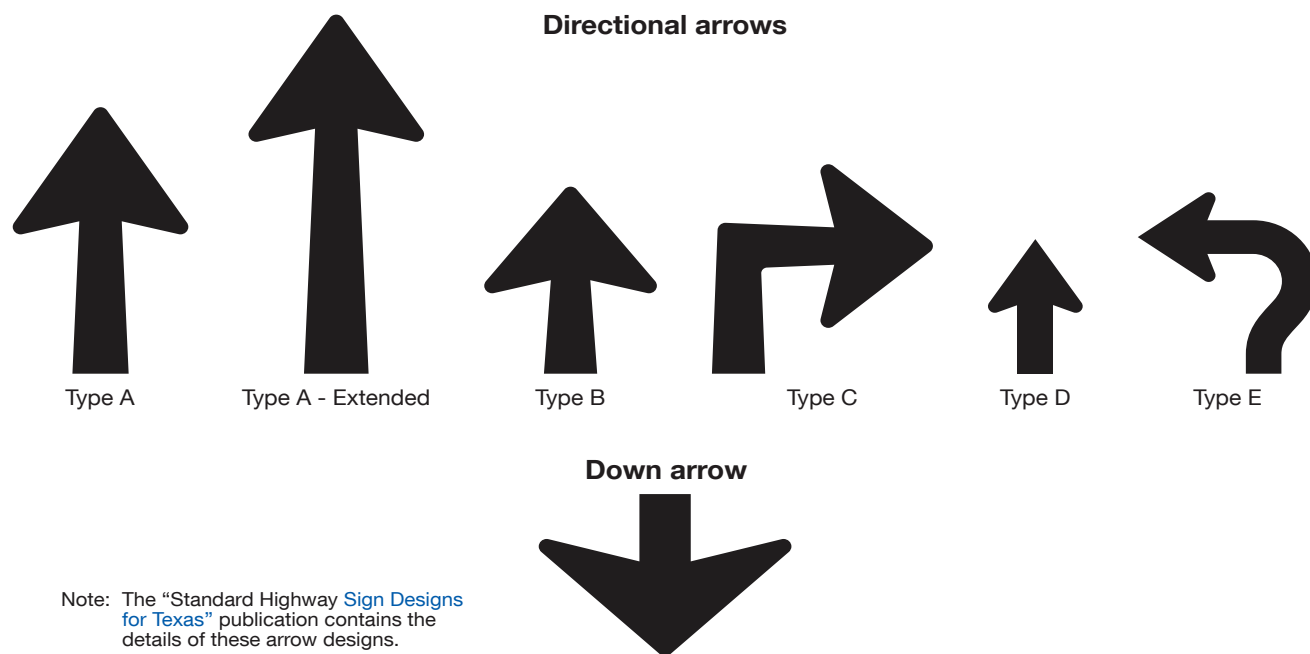
Figure 2D-3. Arrows for Use on Guide Signs
