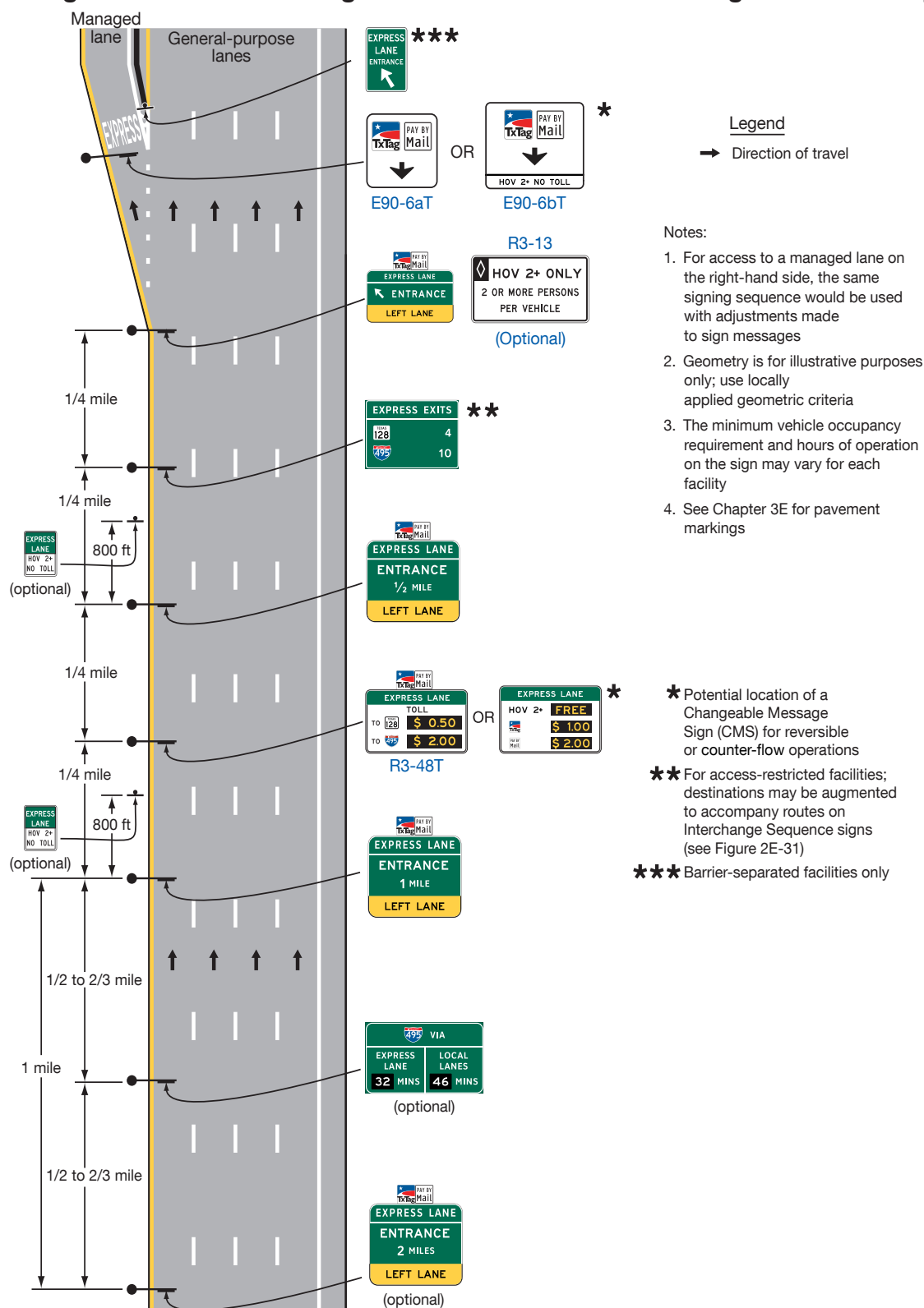
Figure 2G-20. Example of Signing for the Entrance to an Access-Restricted Priced Managed Lane on which Registration in a Toll Account Program is Not Required
