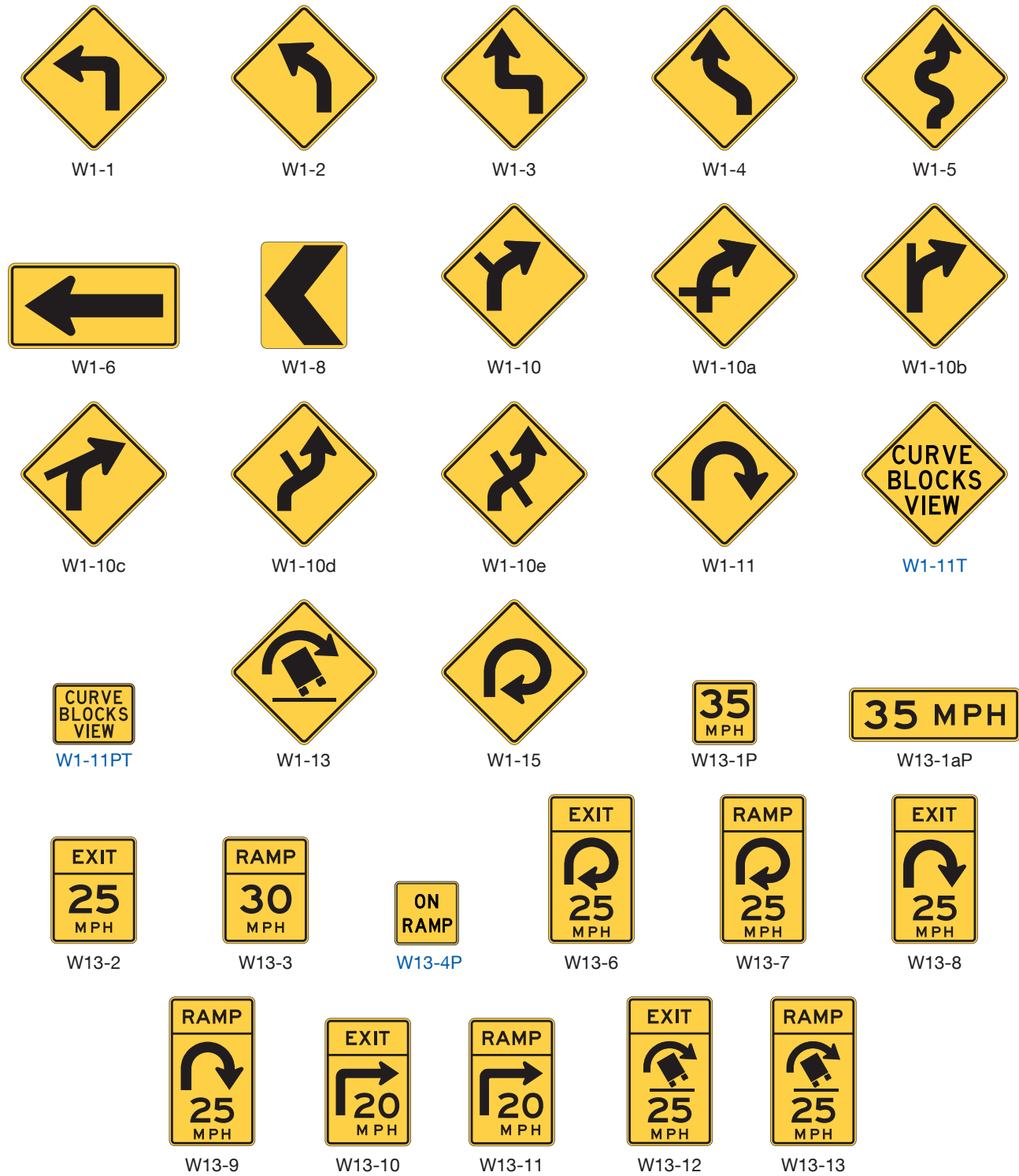
Figure 2C-1. Horizontal Alignment Signs and Plaques
