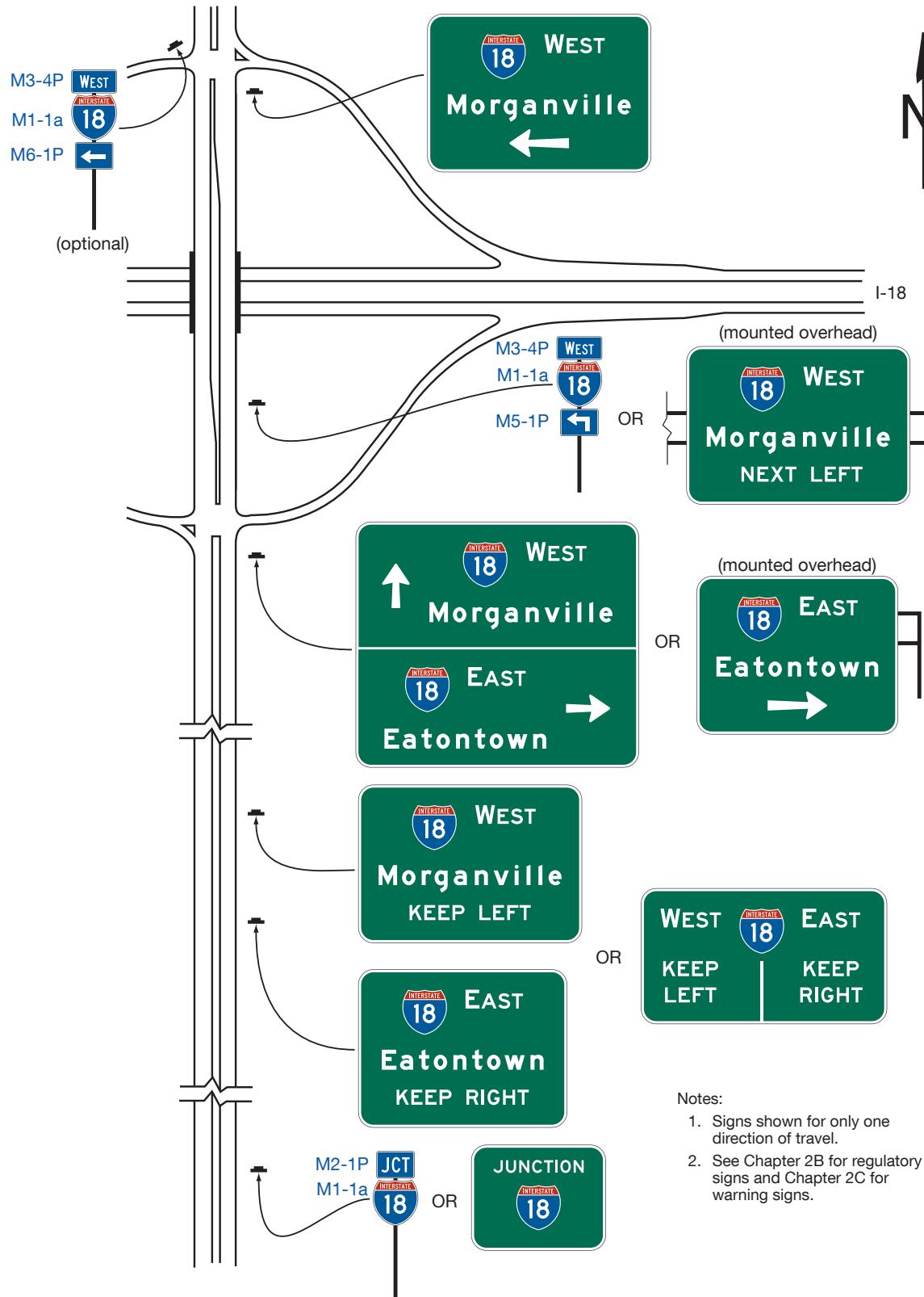
Figure 2D-17. Examples of Multi-Lane Crossroad Guide Signing for a Diamond Interchange
