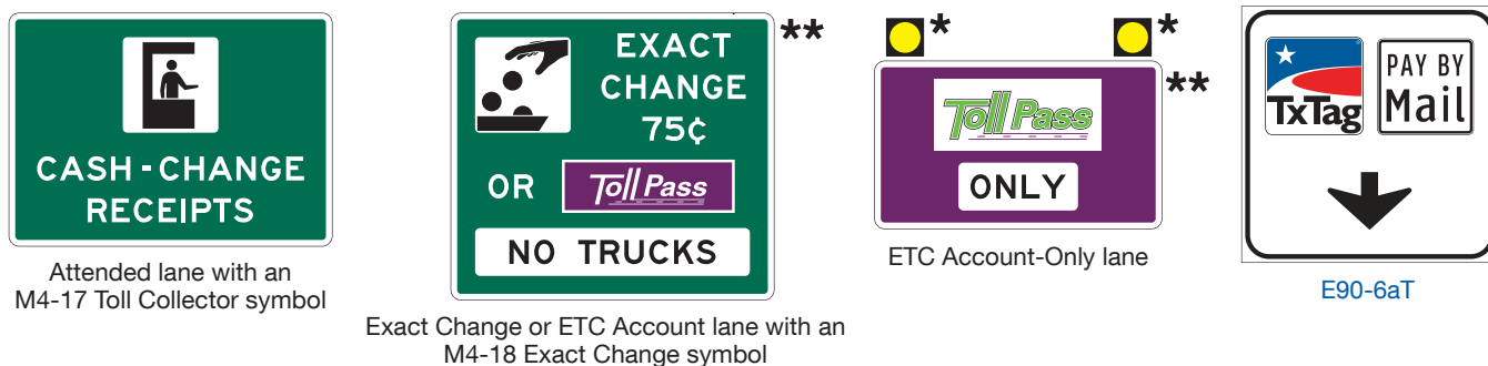
Figure 2F-16. Examples of Toll Plaza Canopy Signs
