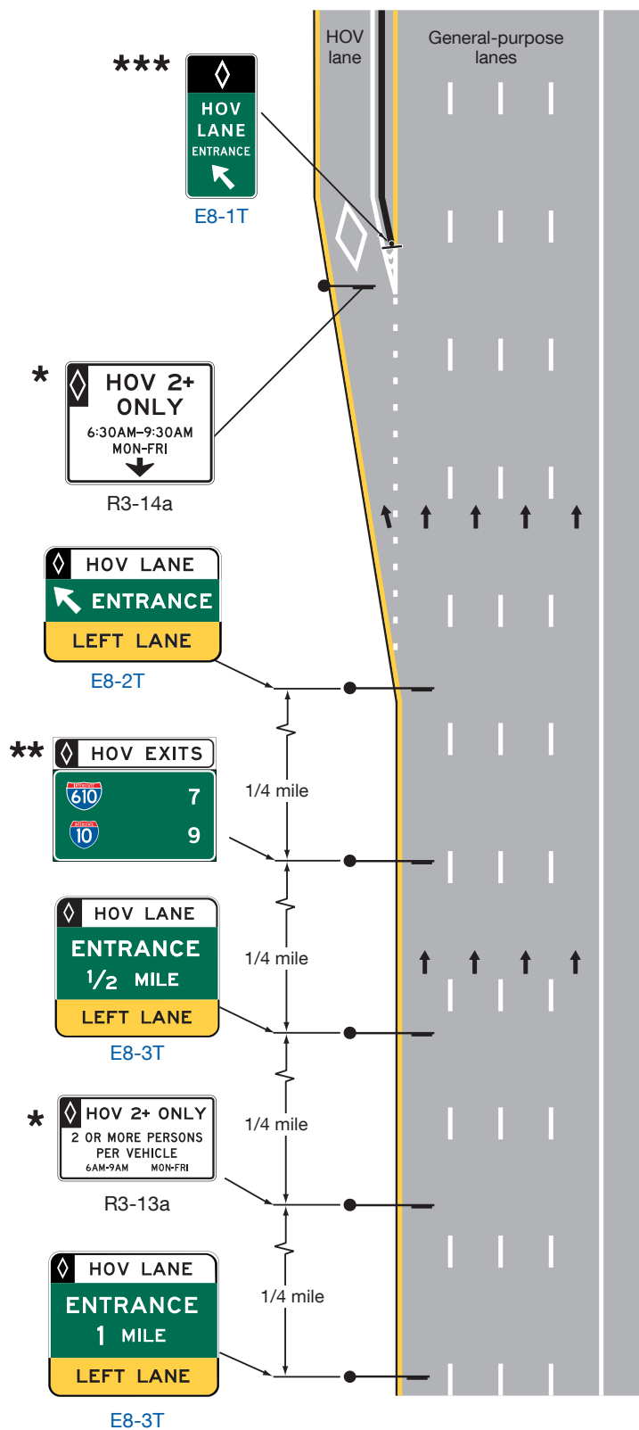
Figure 2G-9. Example of Signing for an Entrance to Access-Restricted HOV Lanes
