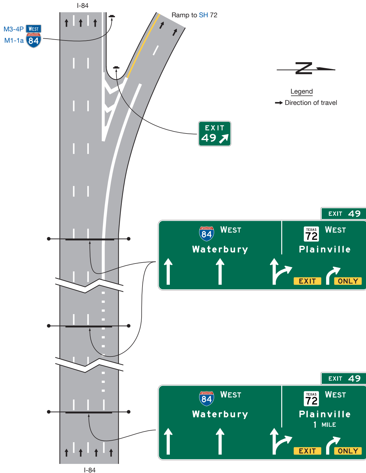
Figure 2E-36. Example of Overhead Arrow-per-Lane Guide Signs for a Two-Lane Exit to the Right with an Option Lane
