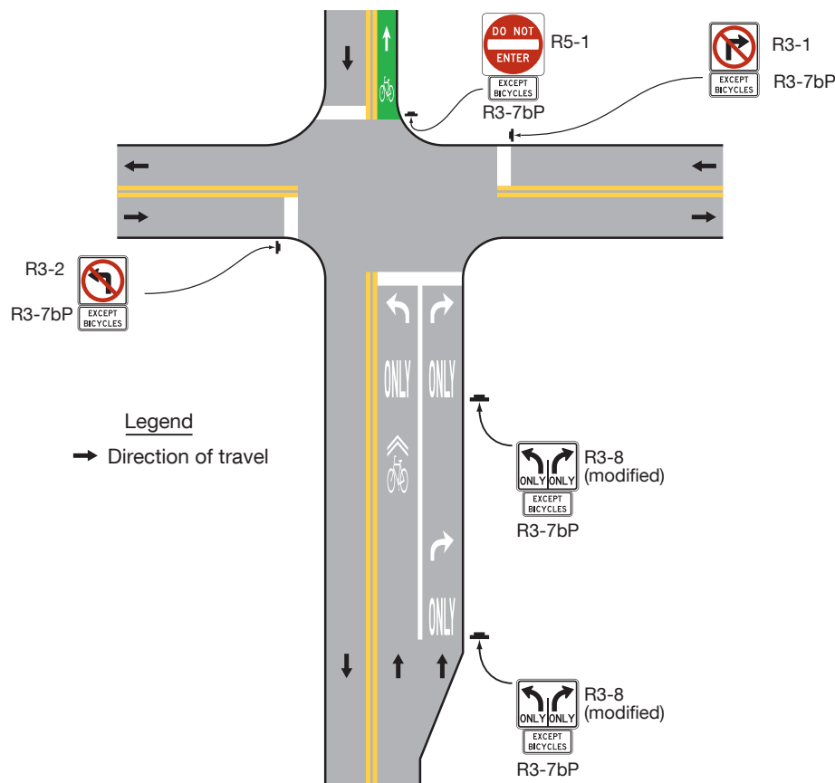
Figure 9B-2. Examples of Applications of EXCEPT BICYCLES Regulatory Plaques
