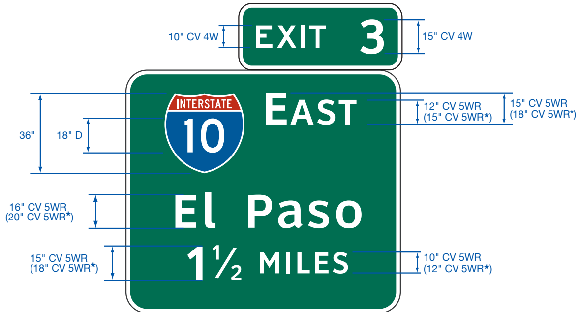
Figure 2E-1A. (TX) Letter Style and Minimum Letter/Numeral Sizes for Advance Guide Signs
