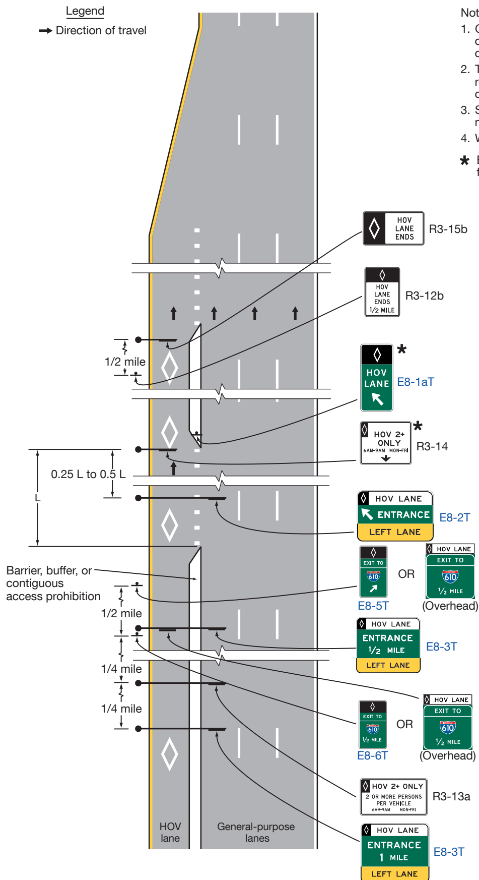
Figure 2G-11. Example of Signing for the Intermediate Entry to, Egress from, and End of Access-Restricted HOV Lanes
