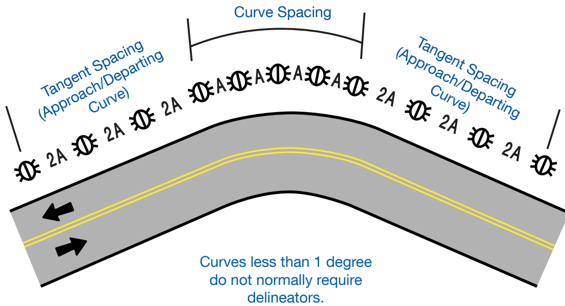
Figure 3G-1A. (TX) Suggested Spacing for Highway Delineators on Horizontal Curves
