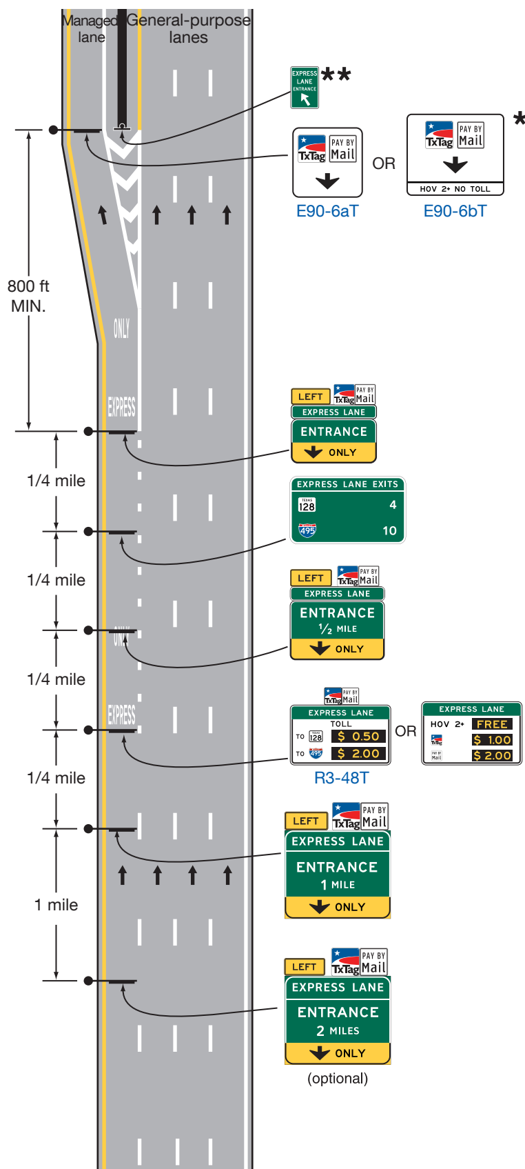
Figure 2G-22. Examples of Signing for the Entrance to an Access-Restricted Priced Managed Lane Where a General-Purpose Lane Becomes the Managed Lane
