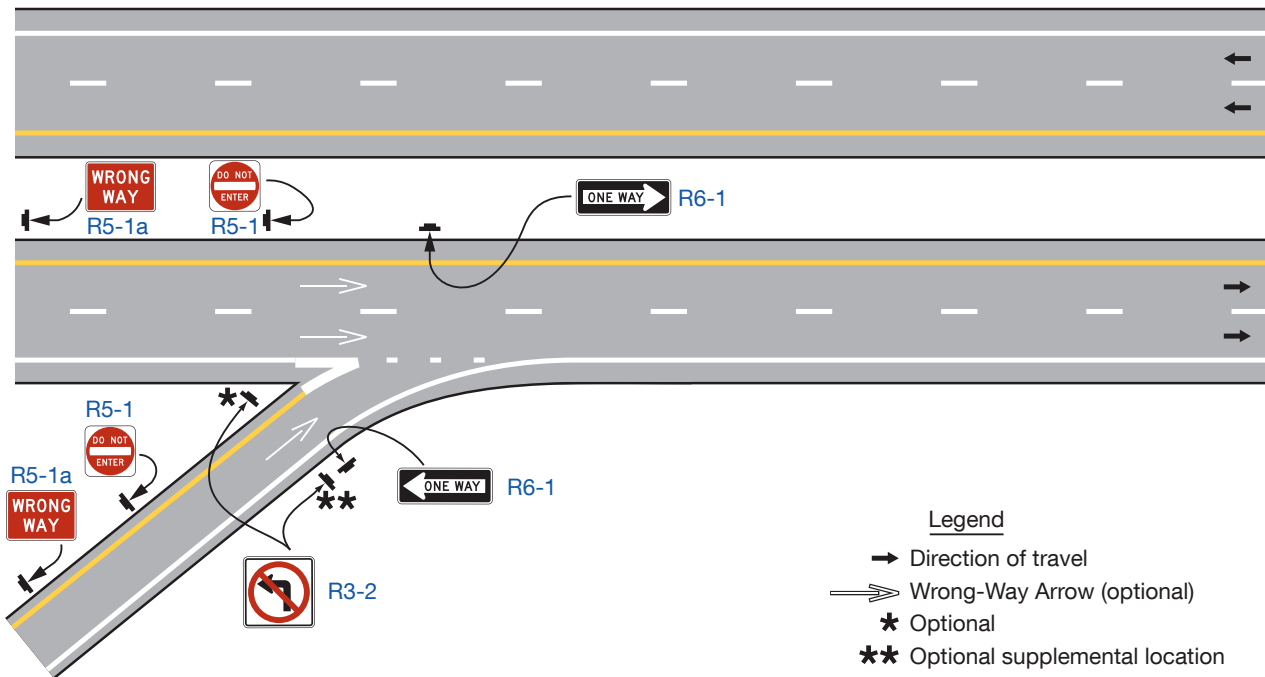
Figure 2B-16. Example of Application of Regulatory Signing and Pavement Marking at an Entrance Ramp Terminal
