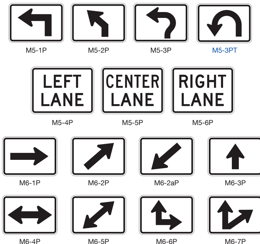
Figure 2D-6. Advance Turn and Directional Arrow Auxiliary Plaques
