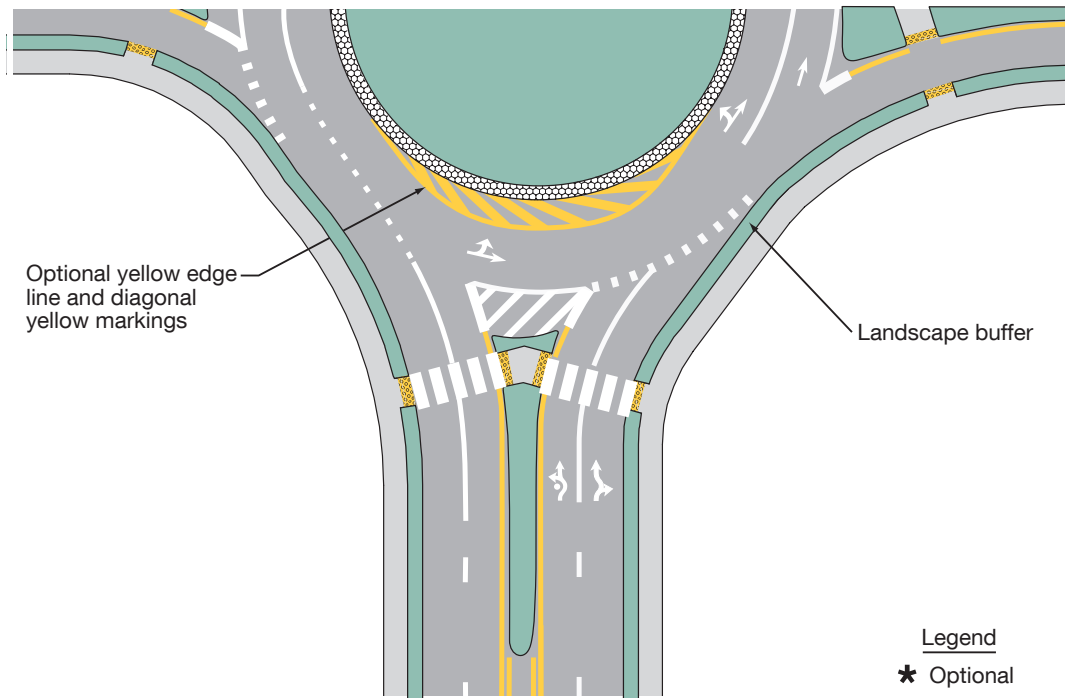
Figure 3D-3. Example of Markings for a Two-Lane Roundabout with One-Lane and Two-Lane Approaches (Sheet 2 of 2)
