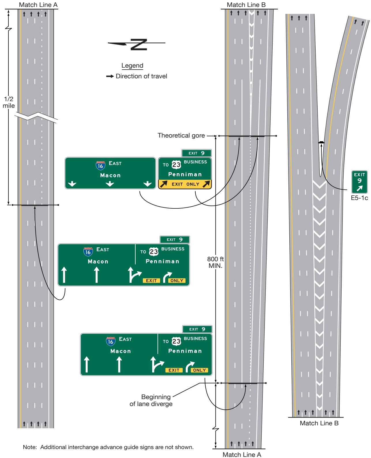
Figure 2E-40. Example of Guide Signing for a Narrow Gore at a Two-Lane Exit with an Option Lane
