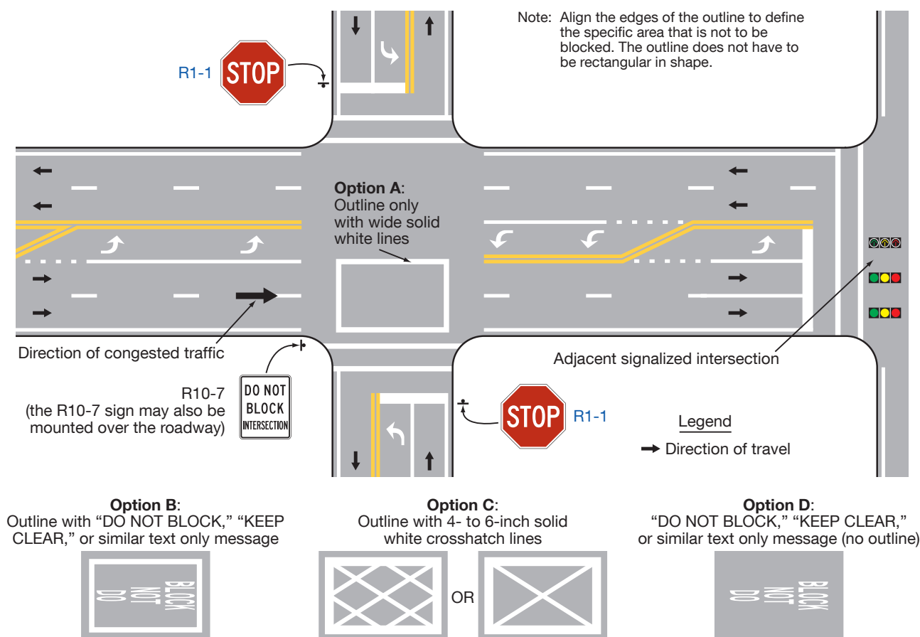
Figure 3B-24. Do Not Block Intersection Markings
