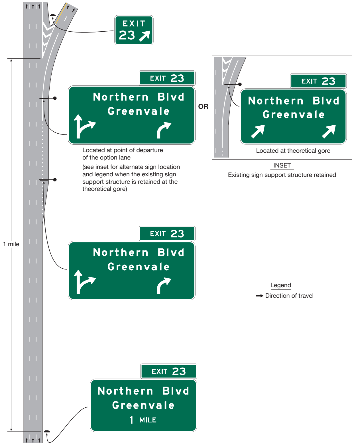
Figure 2E-45. Example of Signing for a Two-Lane Intermediate or Minor Interchange Exit with Option and Auxiliary Lanes using Partial-Width Overhead Arrow-per-Lane Sign
