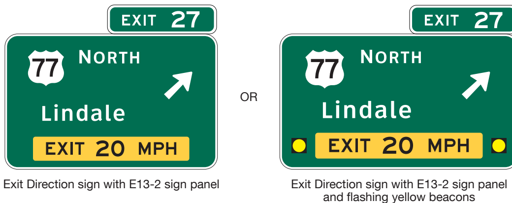
Figure 2E-14. Examples of Exit Direction Signs with Advisory Speed Panels and Flashing Yellow Beacons
