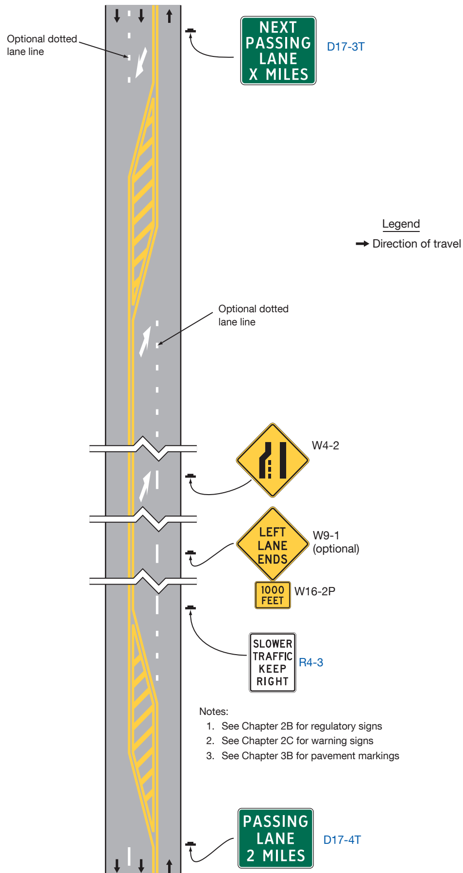
Figure 2D-27. Example of Signing for an Intermittent Passing Lane
