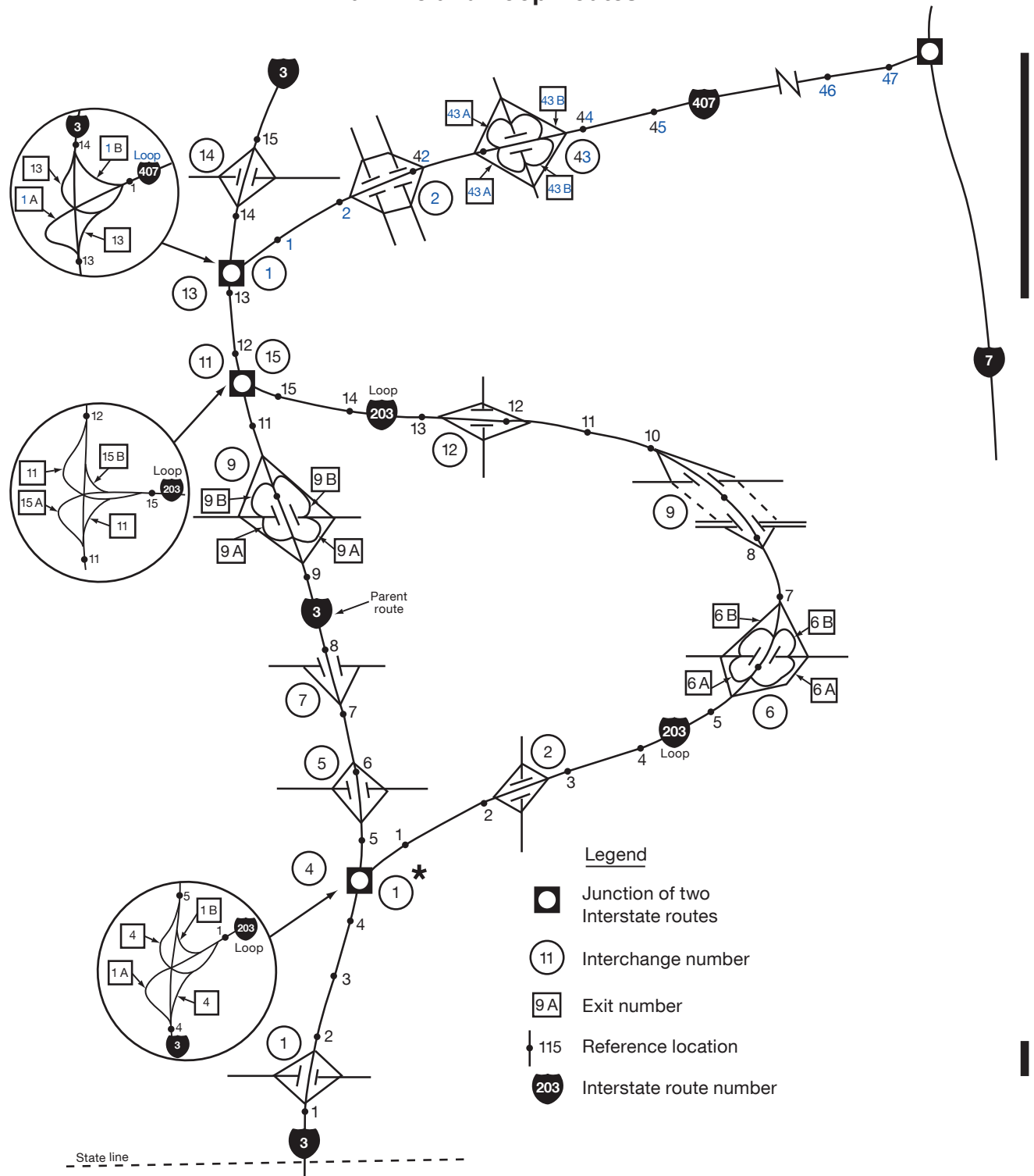
Figure 2E-6. Example of Interchange Numbering for Mainline and Loop Routes
