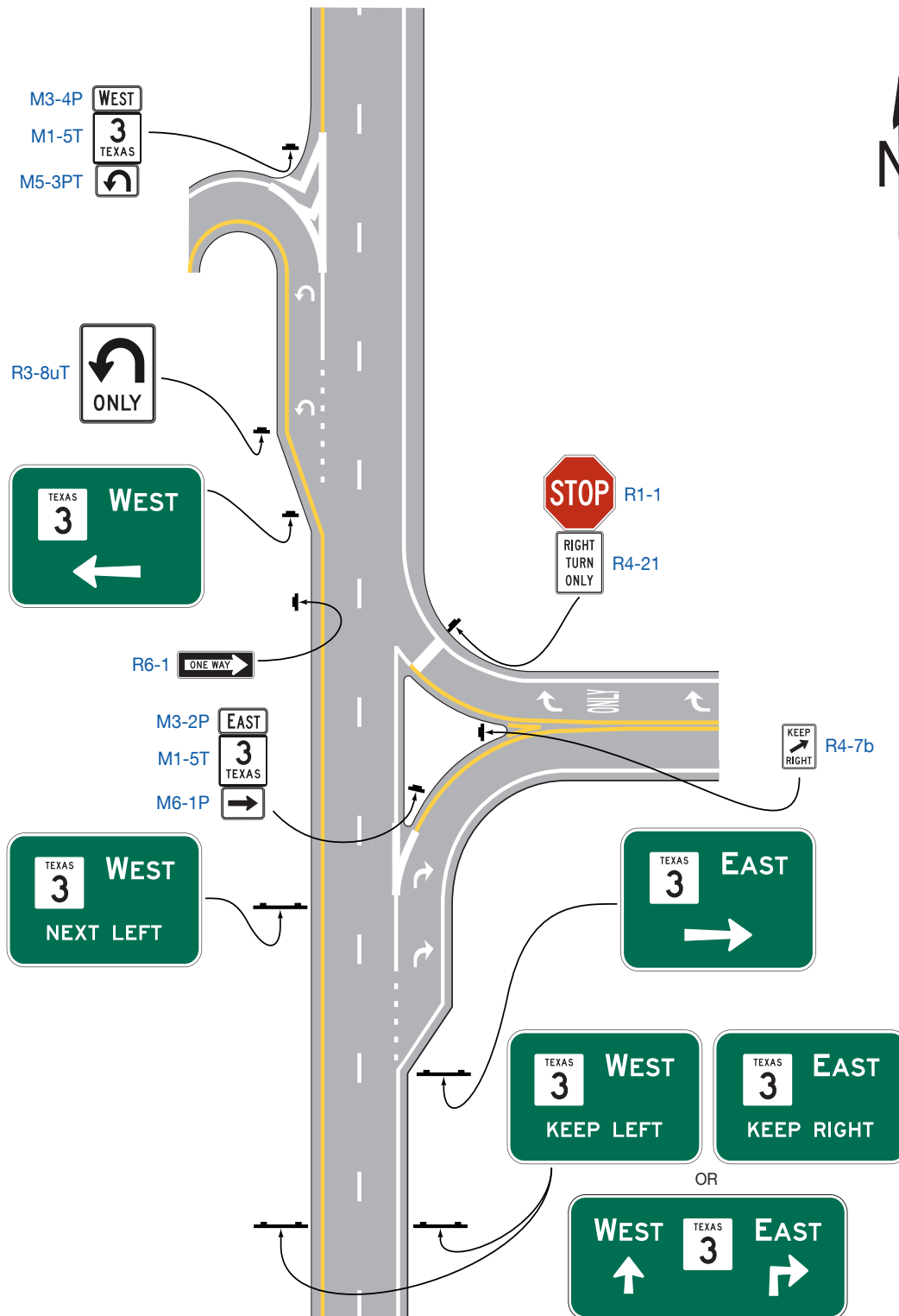
Figure 2D-13. Examples of Signing for Intersections with Indirect Left Turns (Sheet 1 of 3)
