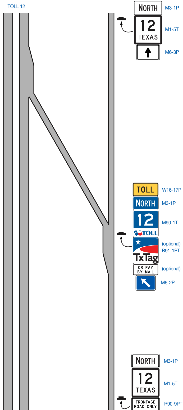
Figure 2F-13B. (TX) Independent Sign Assemblies for Toll Road
