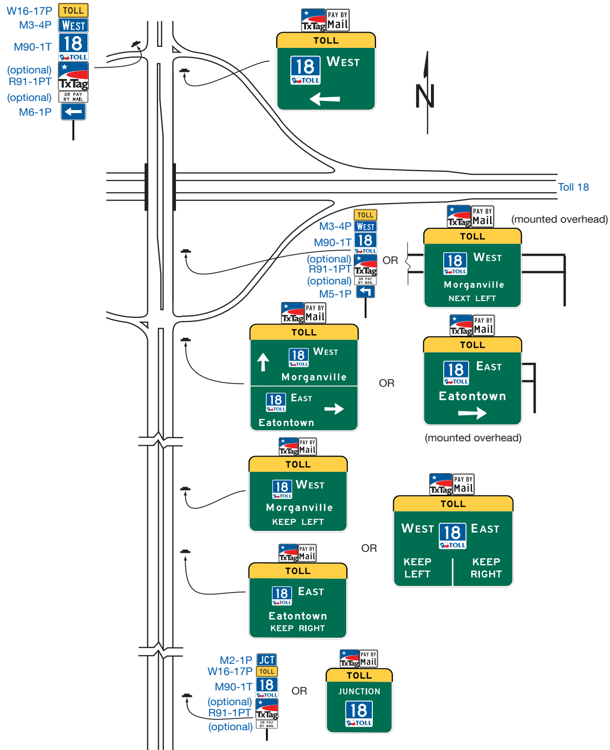
Figure 2F-7. Examples of Multi-Lane Crossroad Signing for a Diamond Interchange
