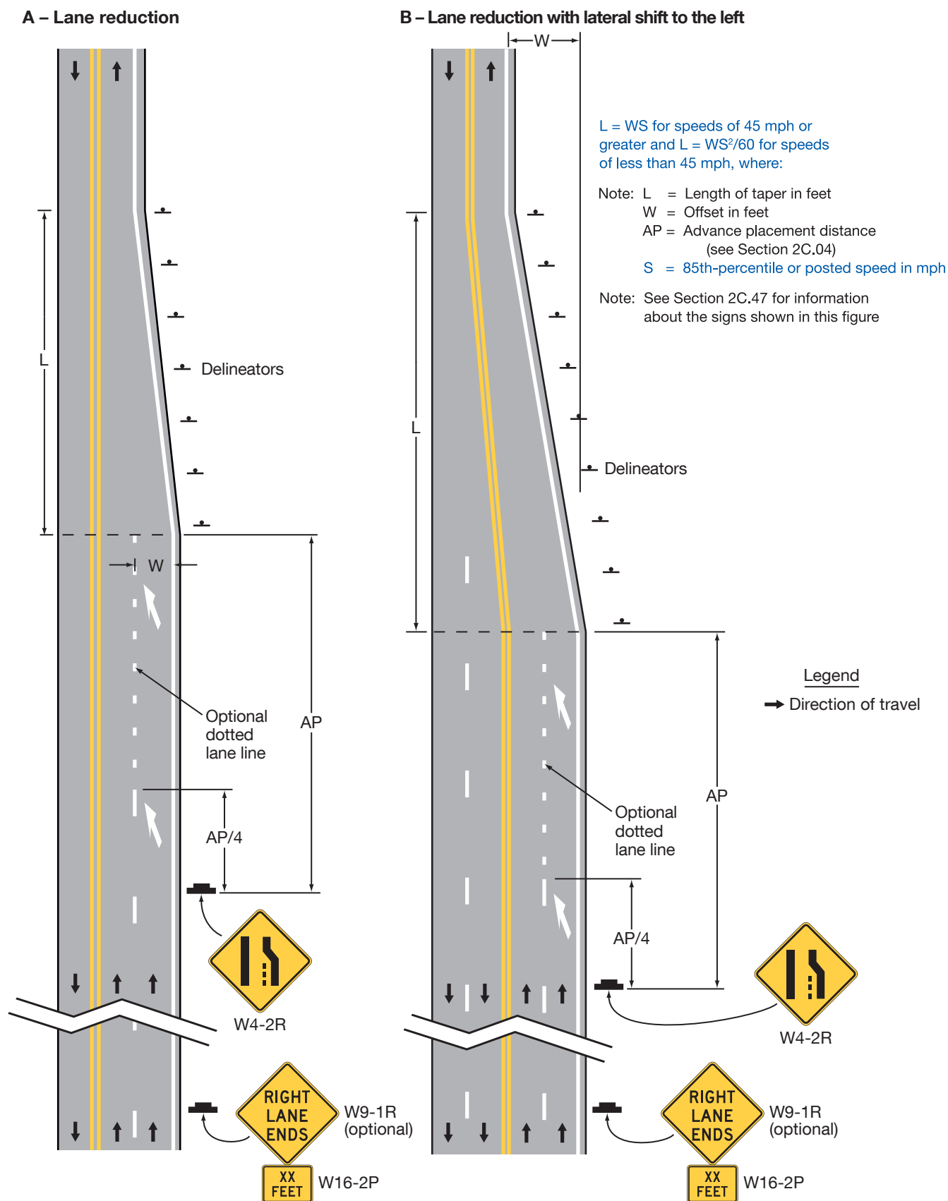
Figure 3B-14. Examples of Applications of Lane-Reduction Transition Markings
