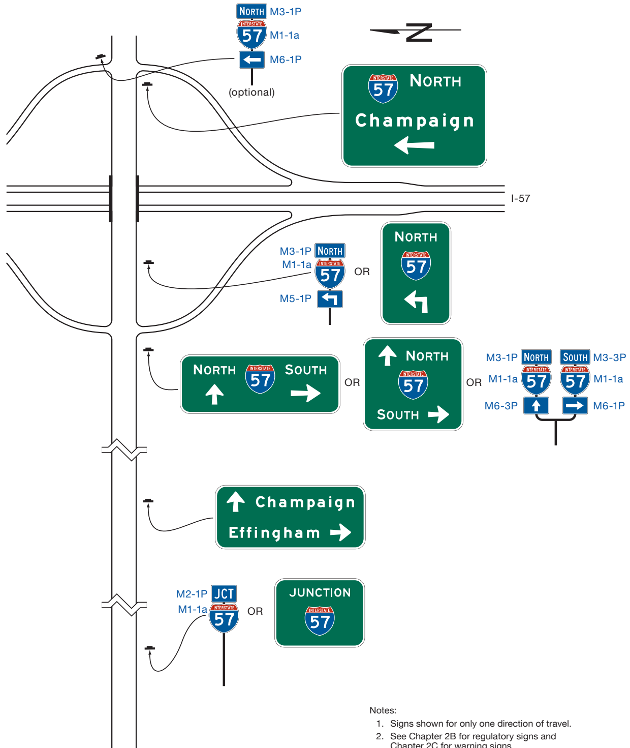
Figure 2D-15. Example of Interchange Crossroad Guide Signing for a One-Lane Approach
