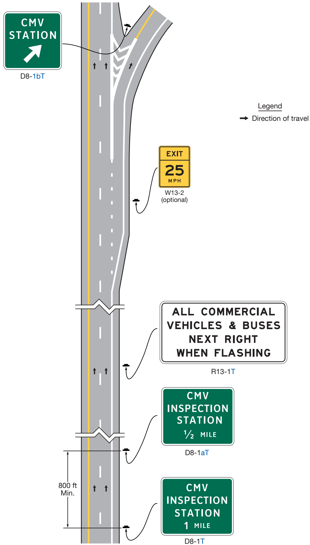
Figure 2E-59. Example of Commercial Vehicle Station Signing on Freeways
