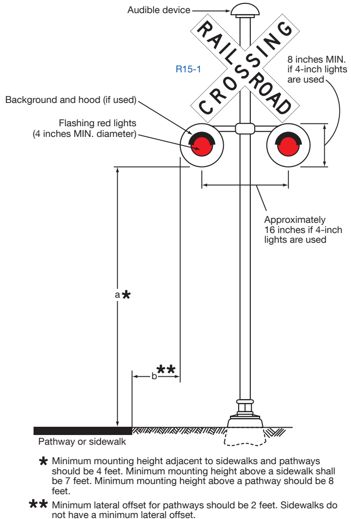
Figure 8E-7. Example of a Flashing-Light Signal Assembly at a Pathway or Sidewalk Grade Crossing
