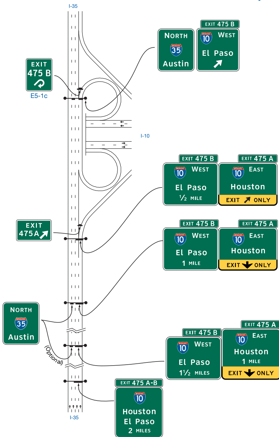
Figure 2E-30A. (TX) Example of Guide Signs for a Full Cloverleaf Interchange without Collector-Distributor Roadways
