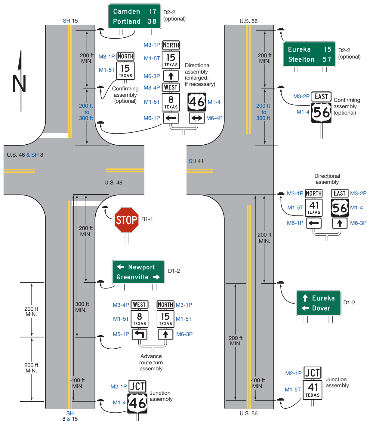
Figure 2D-8. Illustration of Directional Assemblies and Other Route Signs (Sheet 2 of 4)
