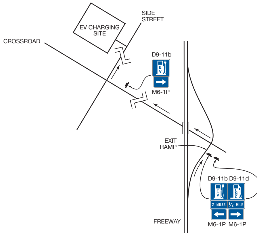
Figure 2H-11. Typical Signing from a Freeway Exit Ramp to a Service Facility
