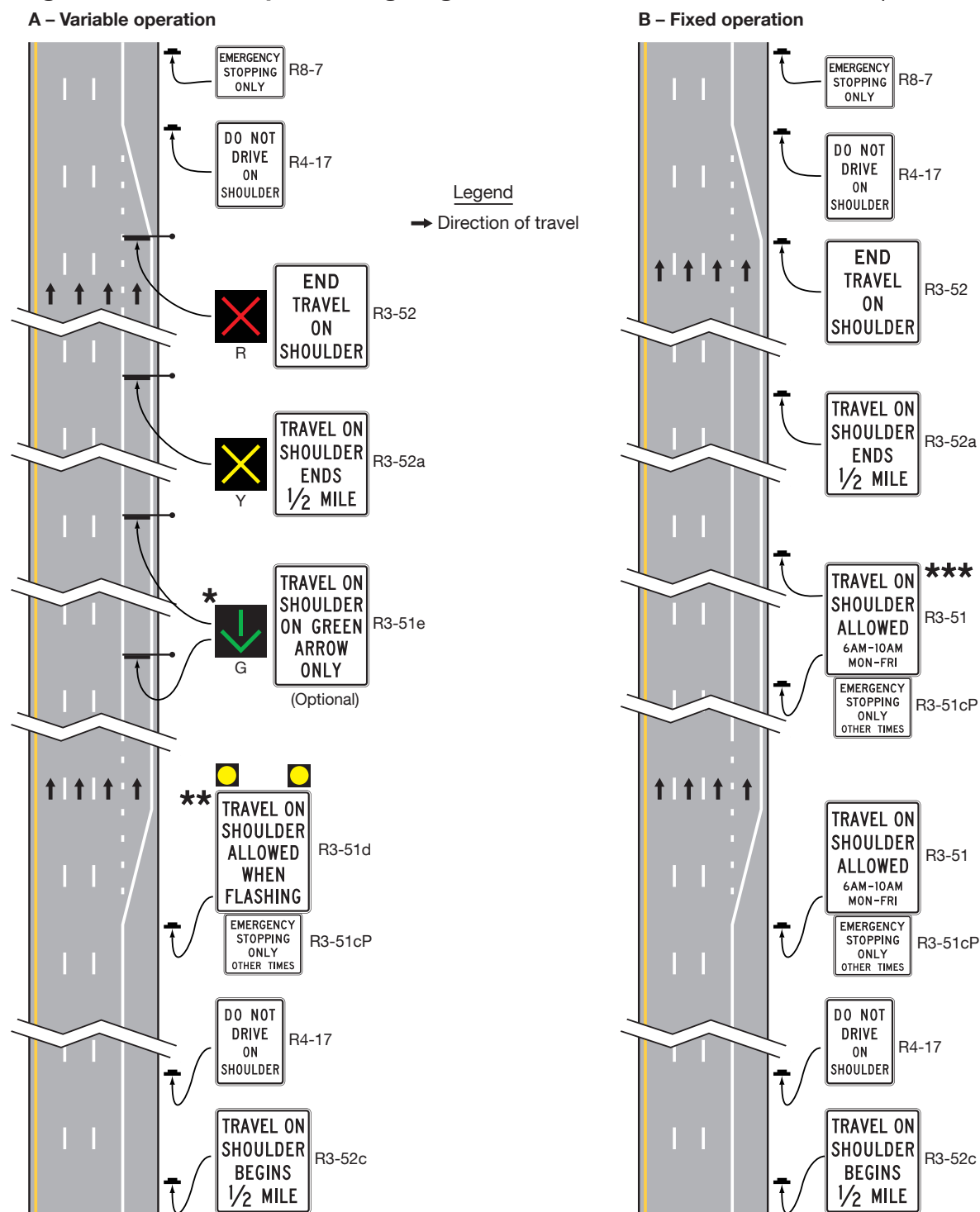
Figure 2G-32. Examples of Signing for Part-Time Travel on Shoulder (Sheet 1 of 4)
