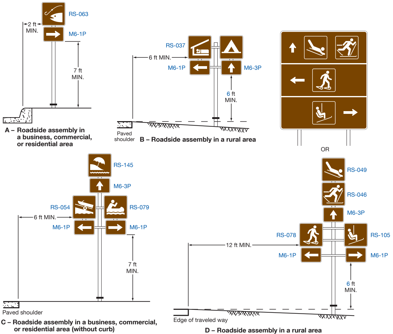
Figure 2M-3. Arrangement, Height, and Lateral Position of Signs Located within Recreational and Cultural Interest Areas
