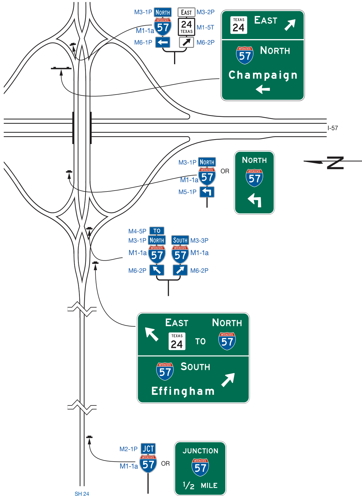
Figure 2D-21. Example of Transposed Alignment Crossroad Guide Signing at a Diamond Interchange
