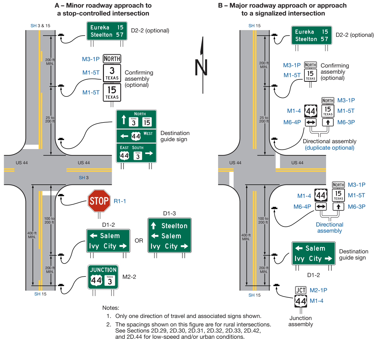
Figure 2D-7. Examples of Consolidation of Route Sign Assemblies into Guide Signs (Sheet 1 of 2)
