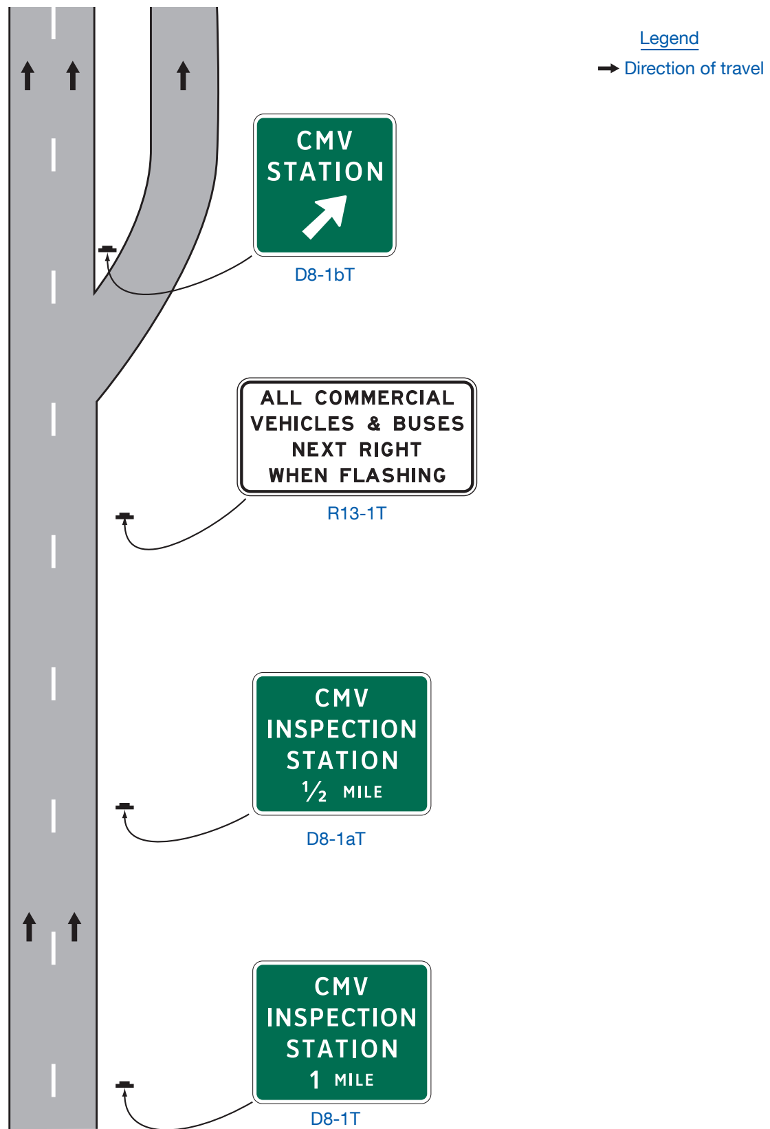
Figure 2D-23A. (TX) Commercial Motor Vehicle (CMV) Inspection Station Signing
