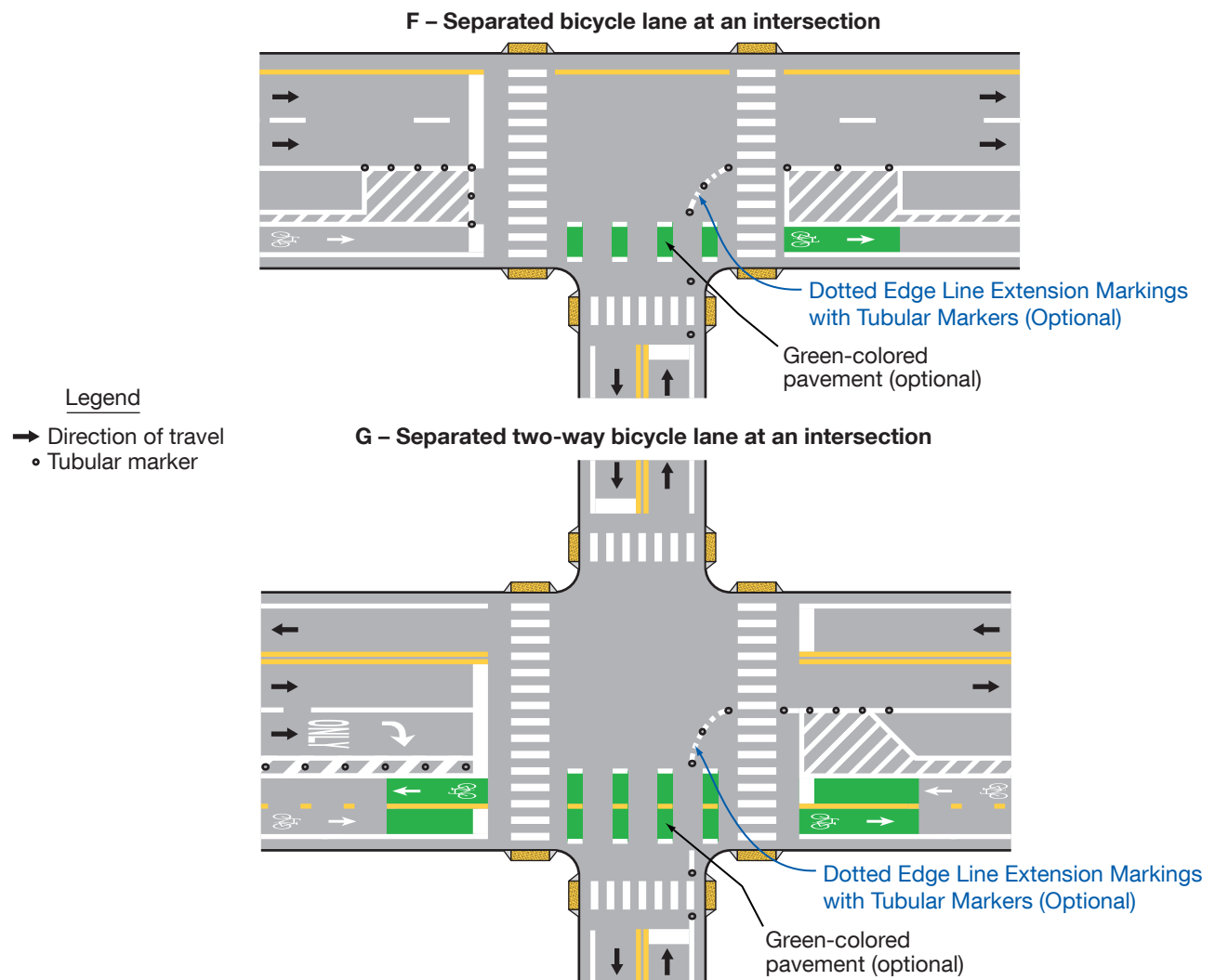
Figure 9E-7. Examples of Lane Markings for Separated Bicycle Lanes (Sheet 2 of 2)
