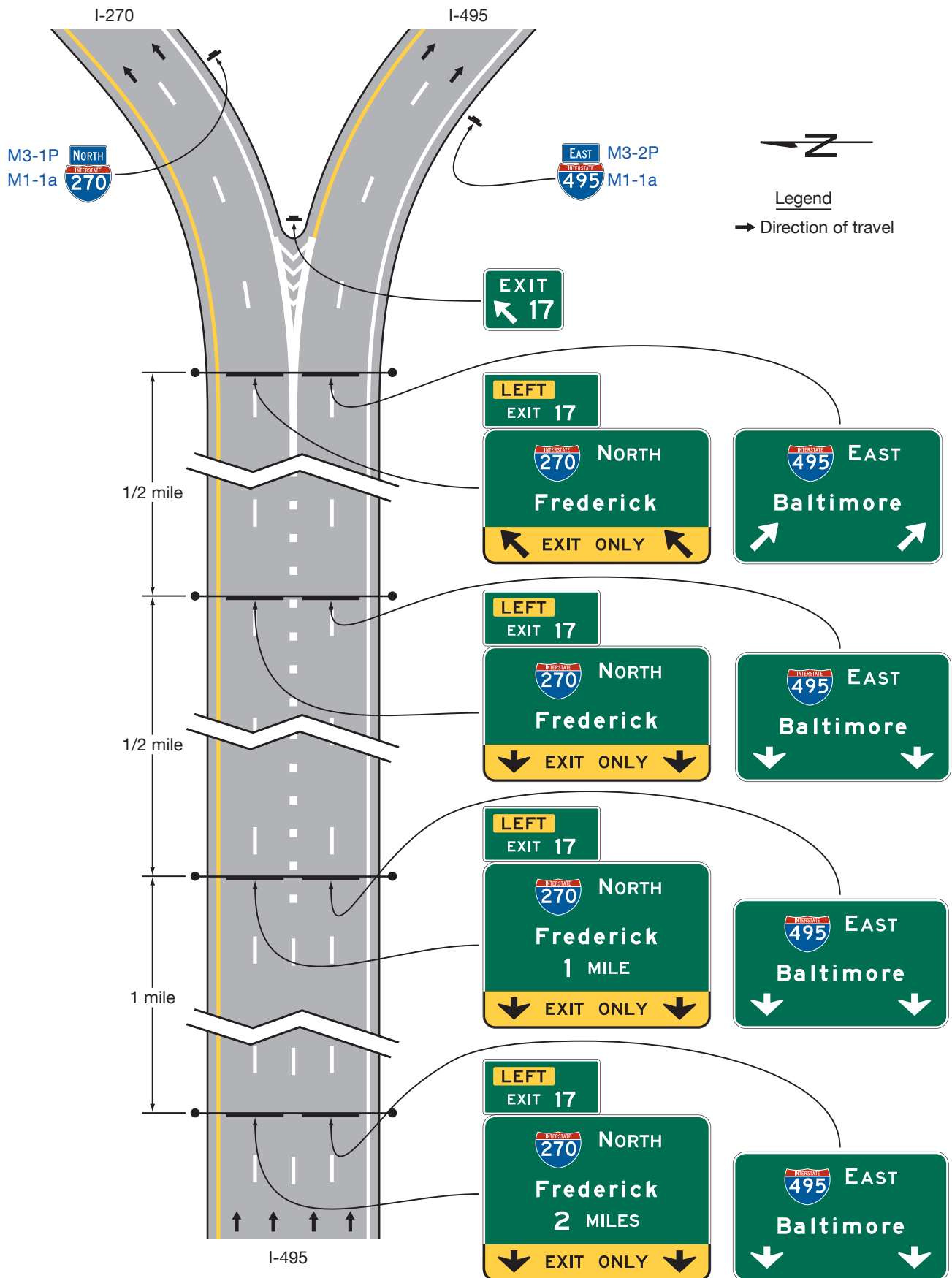
Figure 2E-34. Example of Guide Signs for a Split with Dedicated Lanes
