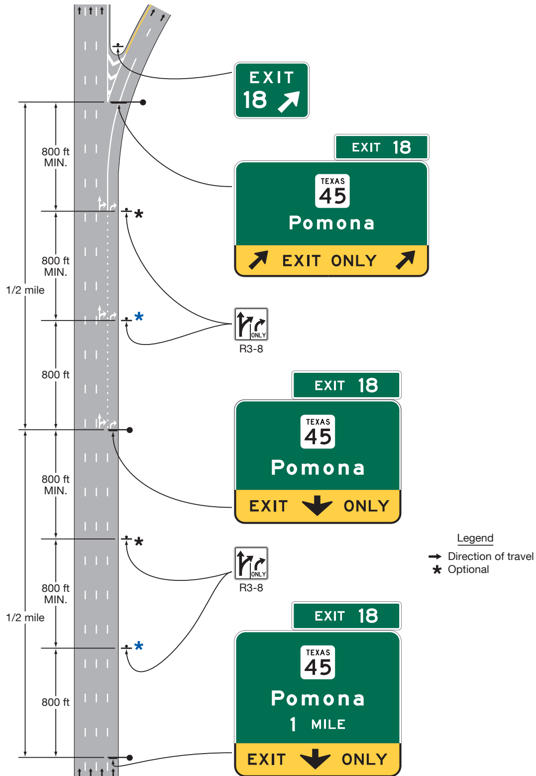
Figure 2E-46. Example of Signing for a Two-Lane Intermediate or Minor Interchange Exit with an Option Lane and a Dropped Lane
