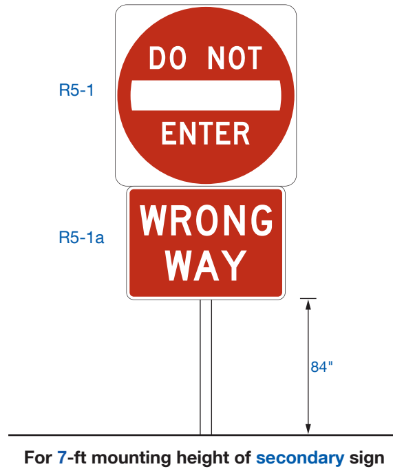
Figure 2B-17. Example of a WRONG WAY and DO NOT ENTER Sign Assembly for Wrong-Way Traffic Control
