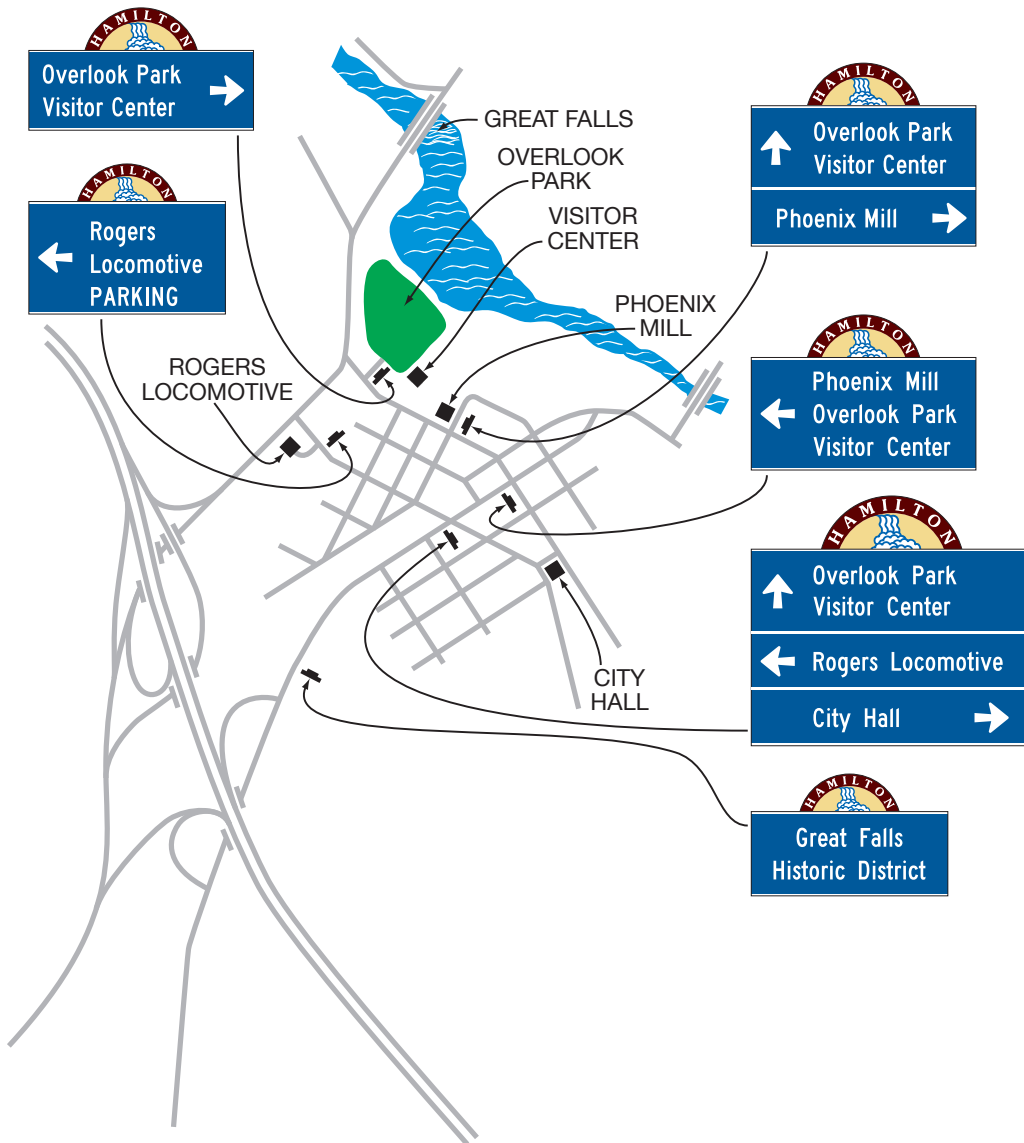
Figure 2D-31. Examples of Community Wayfinding Guide Sign System Showing Direction from a Freeway or Expressway
