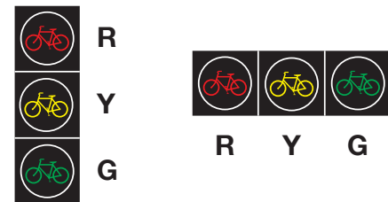
Figure 4H-1. Typical Arrangements of Bicycle Signal Faces
