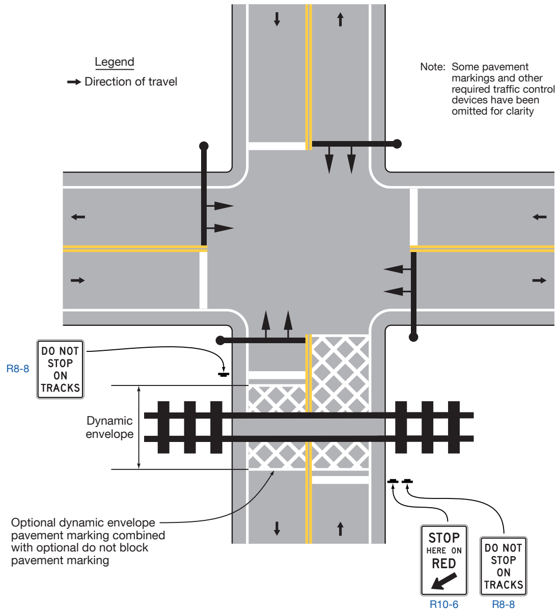
Figure 8C-4. Example of Dynamic Envelope and Do Not Block Pavement Markings at Grade Crossings
