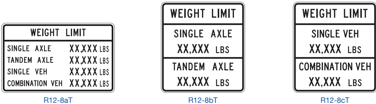
Figure 2B-30. Road Closed and Weight Limit Signs (Sheet 2 of 2)
