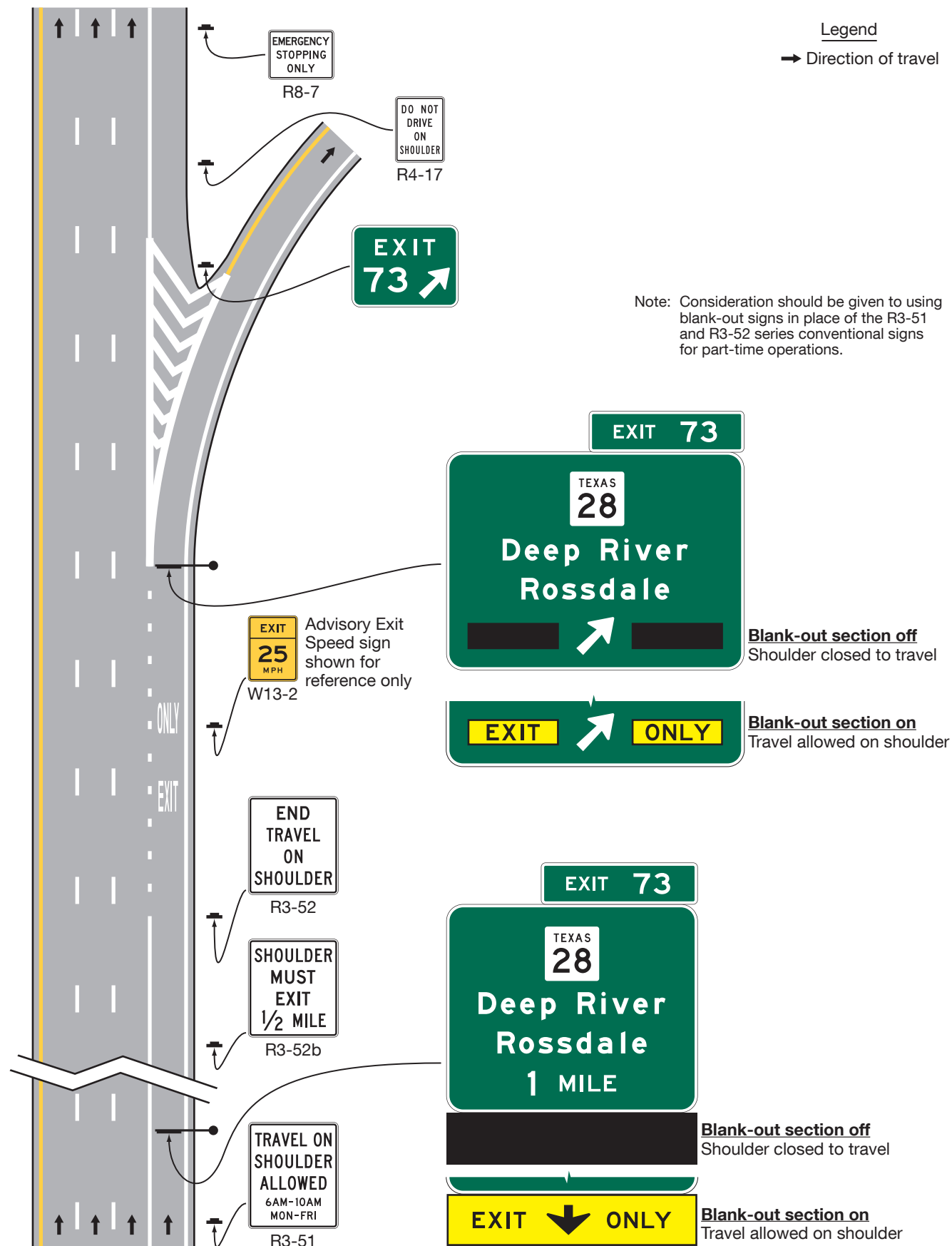
Figure 2G-32. Examples of Signing for Part-Time Travel on Shoulder (Sheet 4 of 4)
