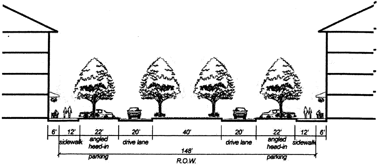
Retail Street Section A
