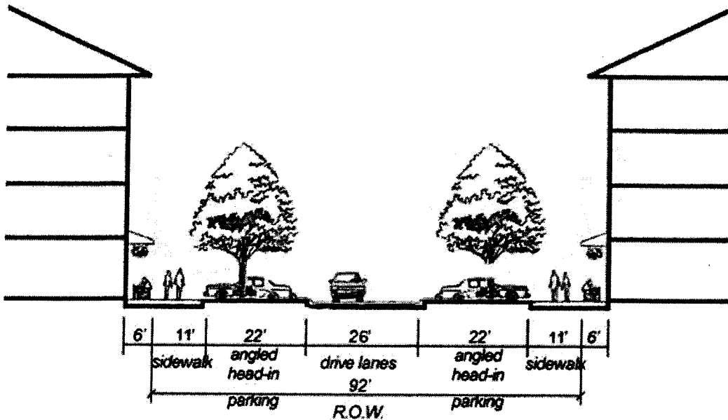
Retail Street Section B
