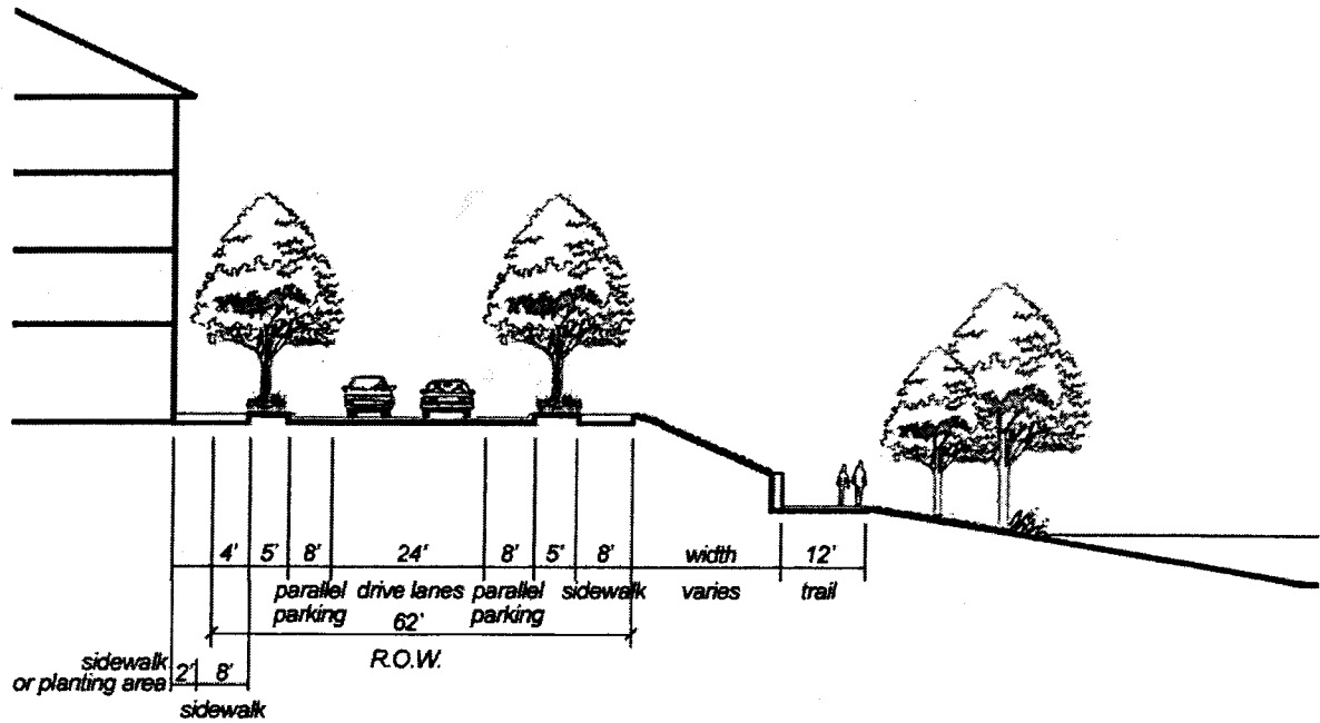
Park Side Street Section
