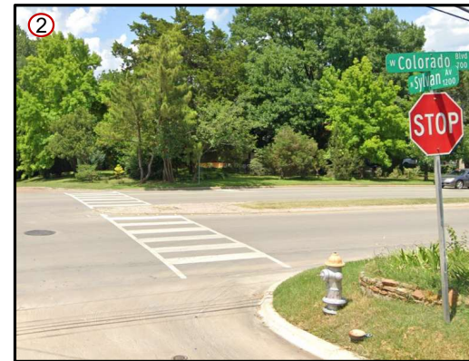
Pedestrian crossing with no controlled pedestrian signal or pedestrian ramps
