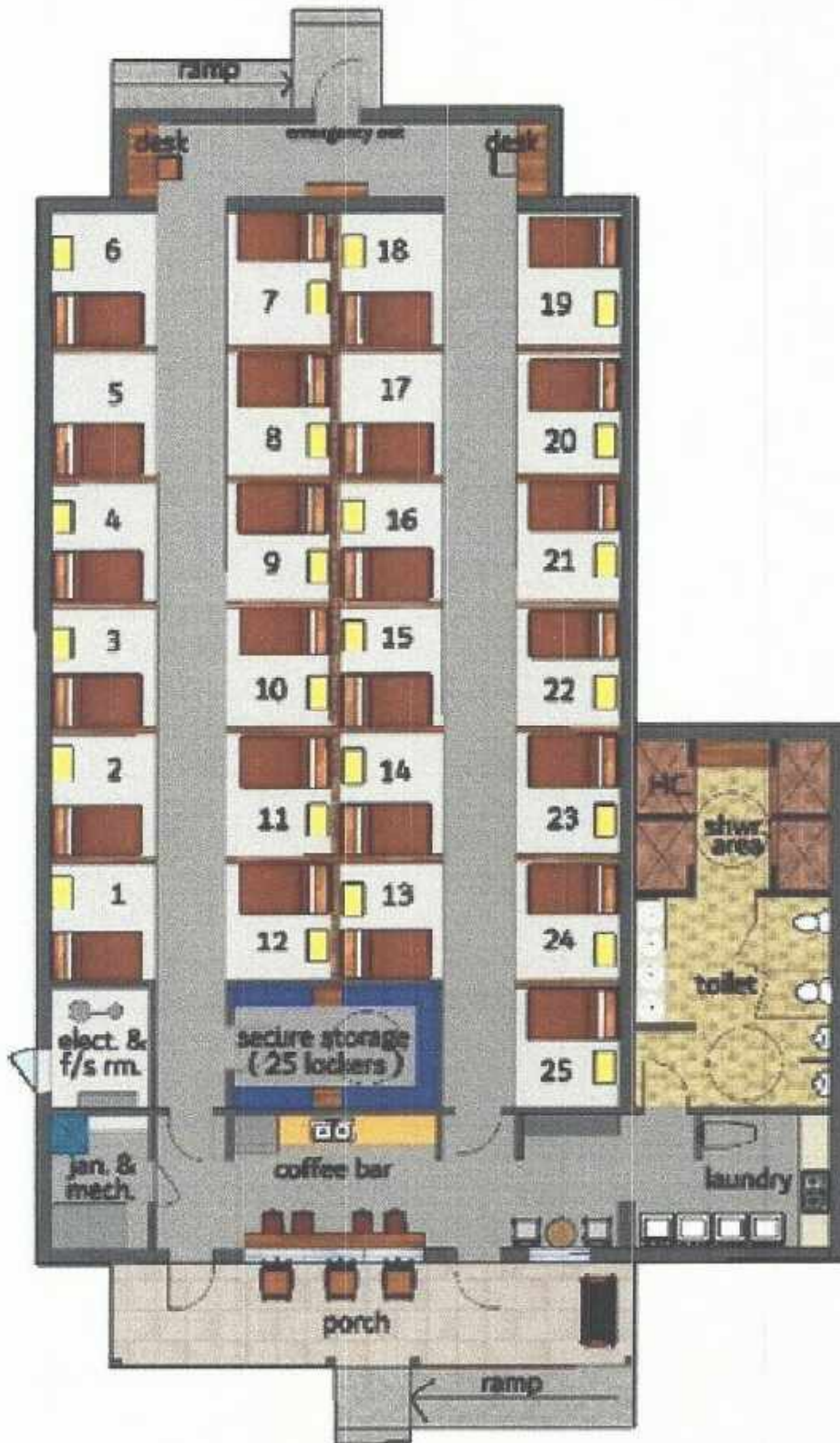
typical resident unit floor plan
