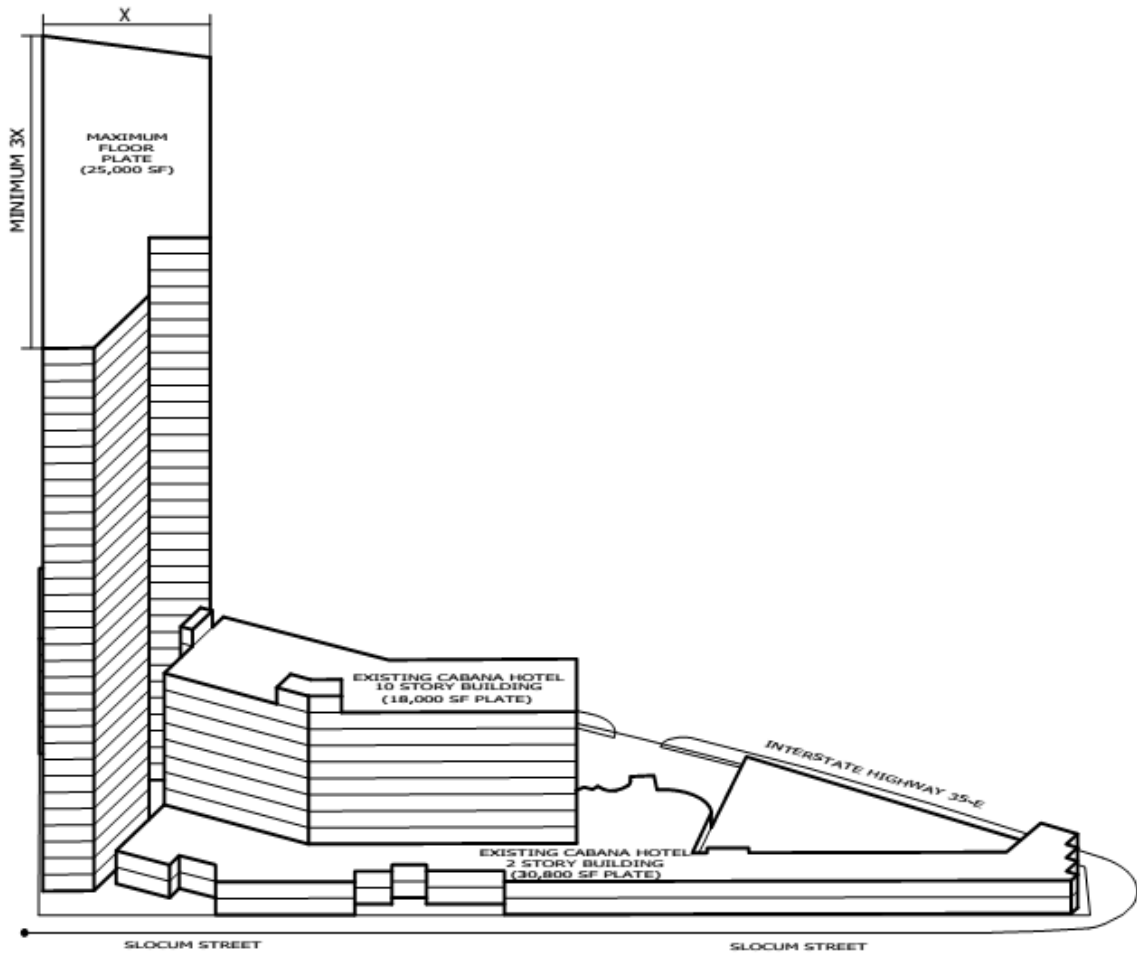
TOWER DIAGRAM
