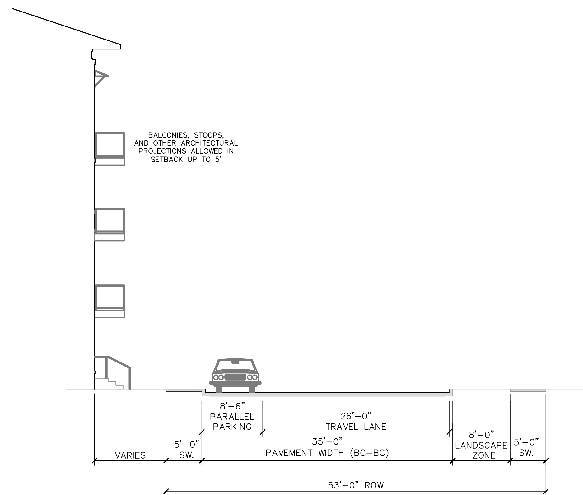
CROSS SECTION R-R PROPOSED 53' RIGHT-OF-WAY W/ PARALLEL PARKING (ONE SIDE)
