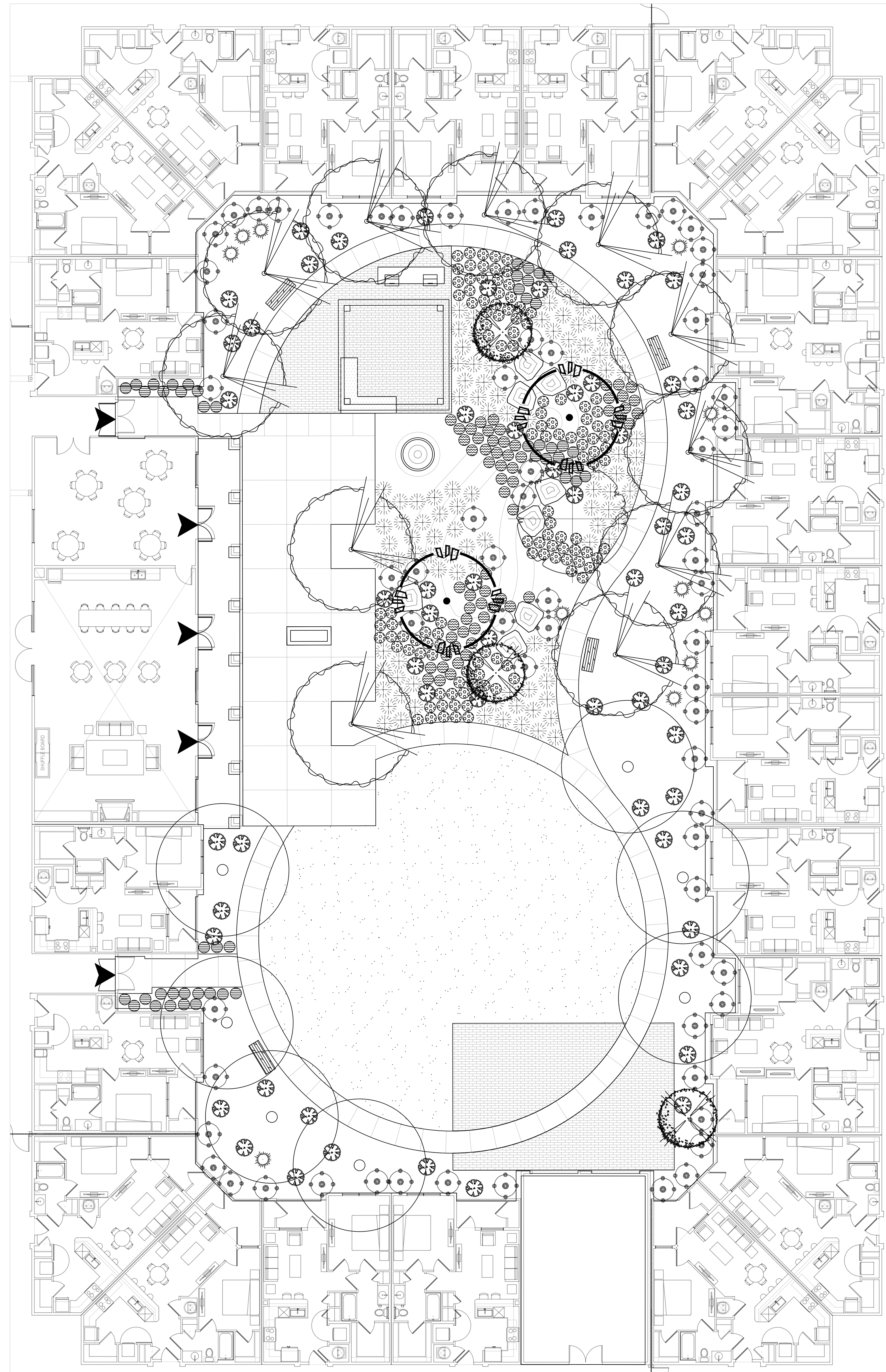
LANDSCAPE PLAN COURTYARD
