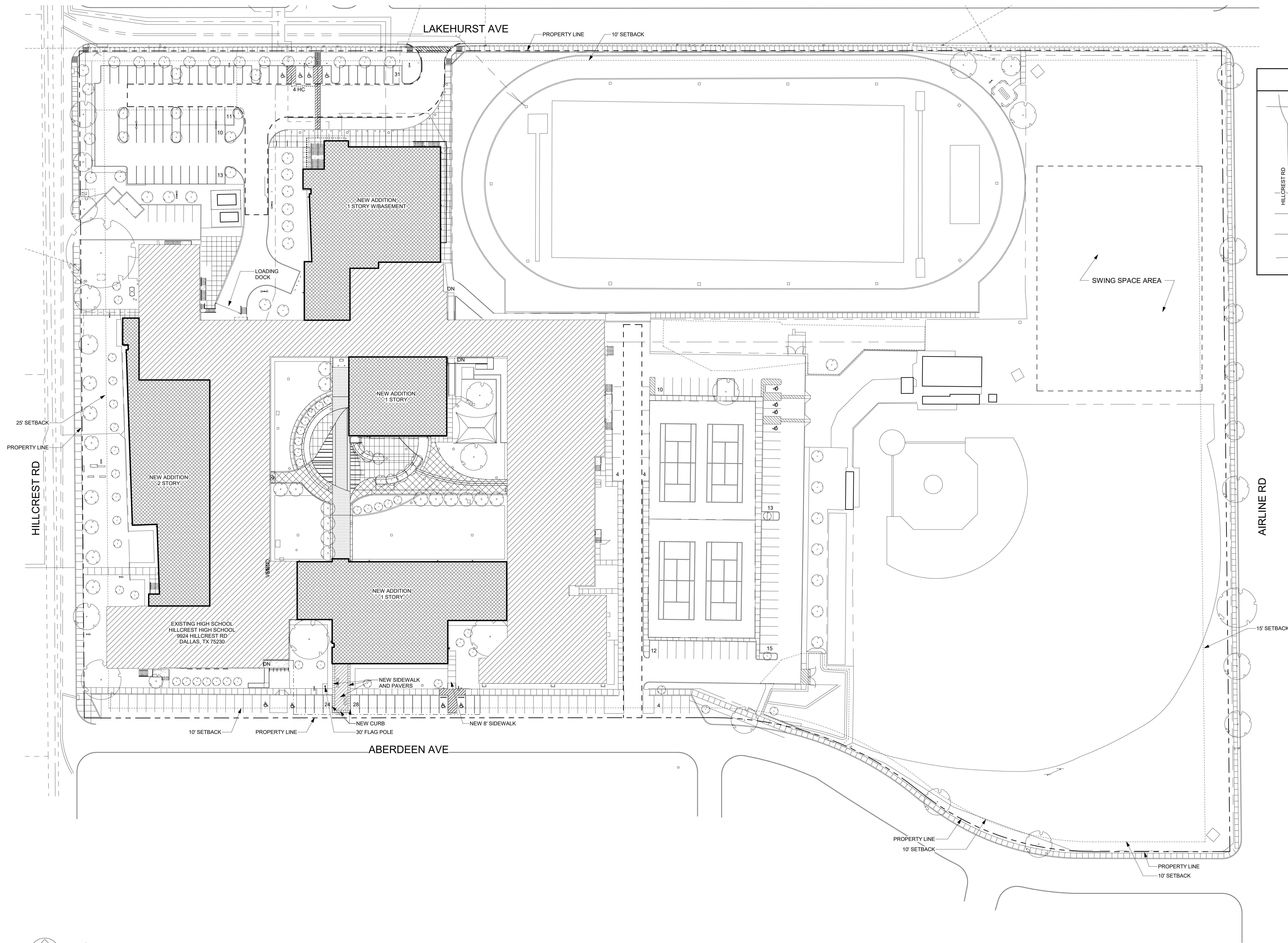
1 Development Plan 1" = 40'-0"
