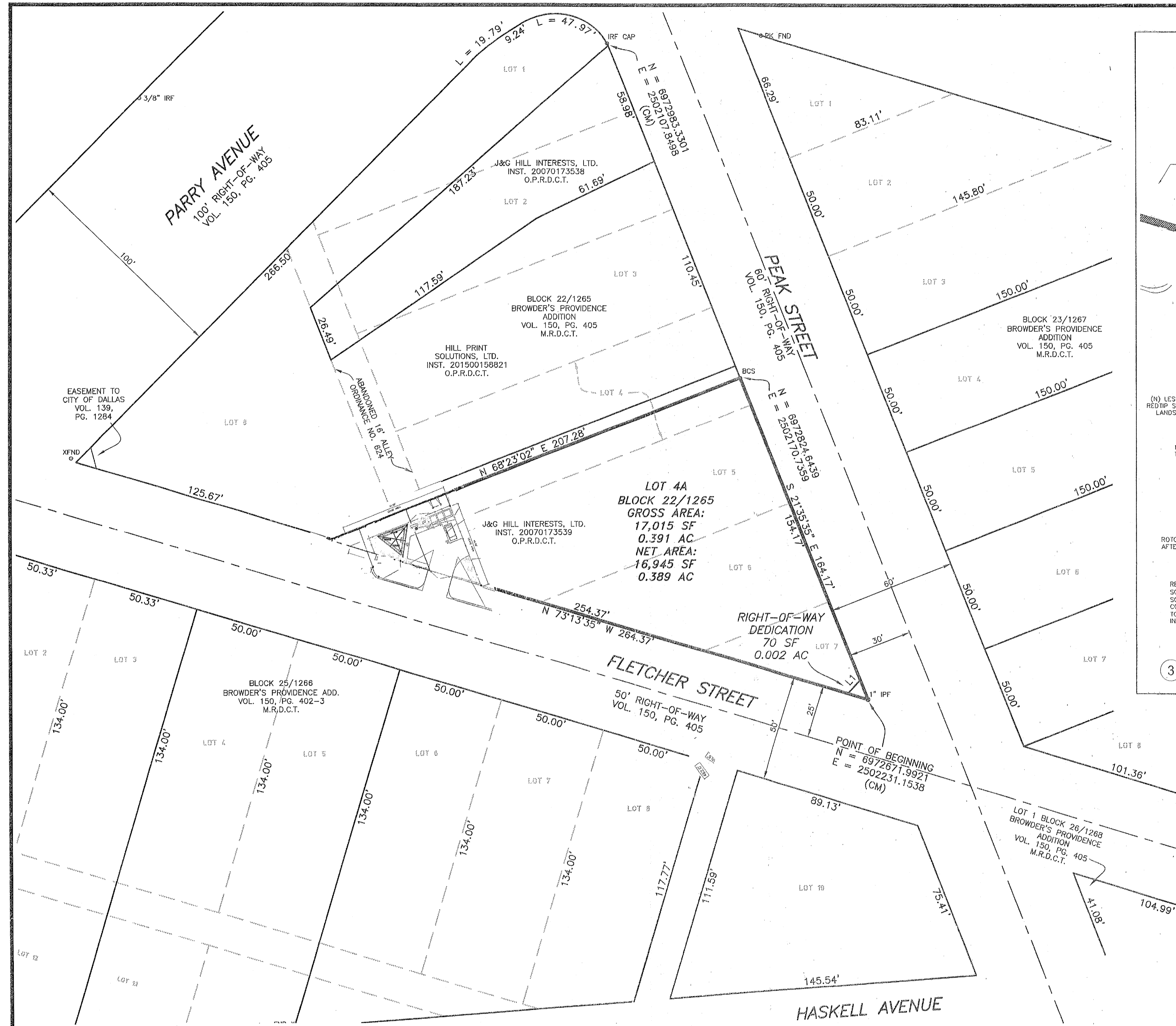
SITE PLAN FULL BLOCK
