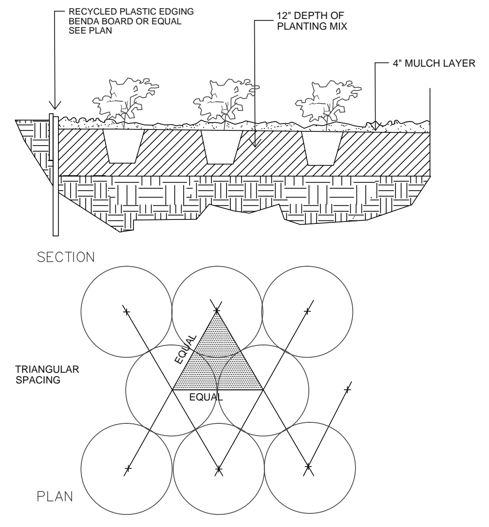
4 GROUNDCOVER PLANTING SCALE: NONE
