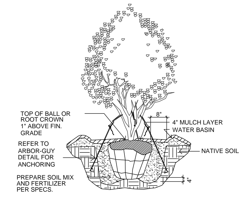
2 MULTI-TRUNK PLANTING SCALE: NONE
