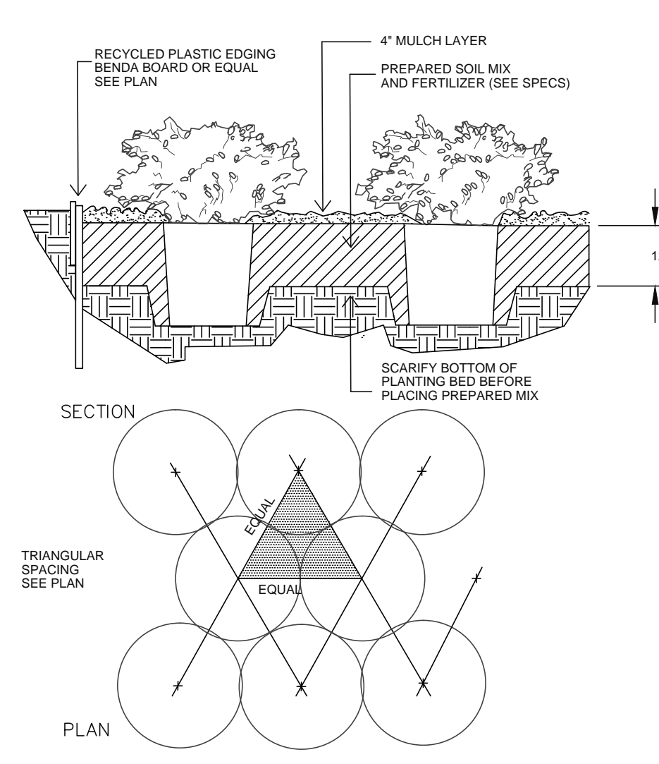
3 SHRUB PLANTING SCALE: NONE
