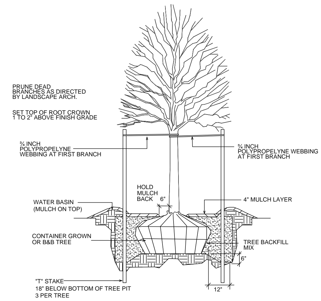
1 CANOPY TREE PLANTING SCALE: NONE
