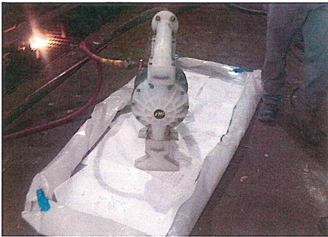
13. View of poly-pump and secondary containment prior to pumping chromic acid waste from sumps.
