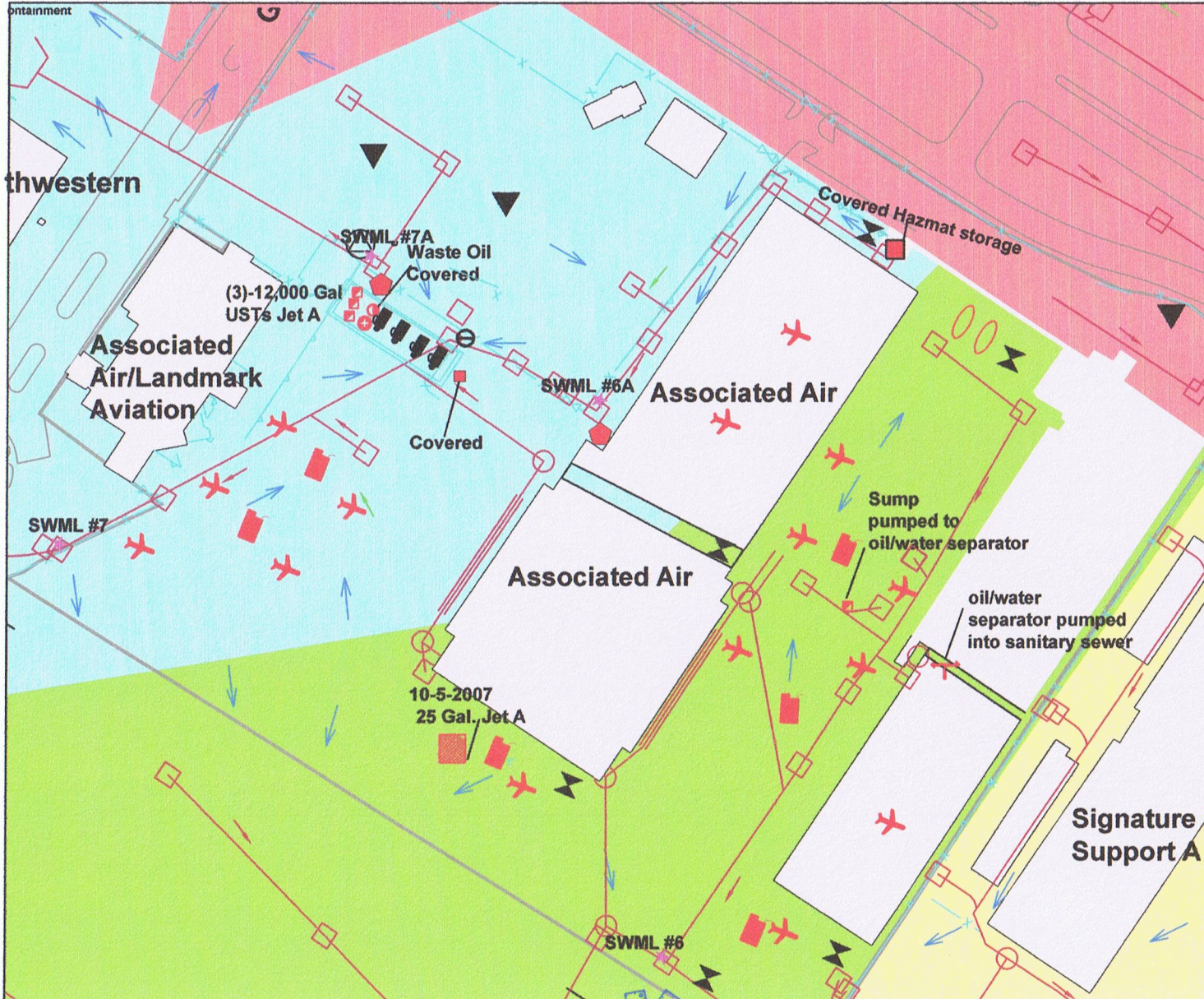
SWPPP Love Field Airport Site Map Associated Air/Landmark Aviation A Figure 5a April 2009 Sheet 1 of 2
