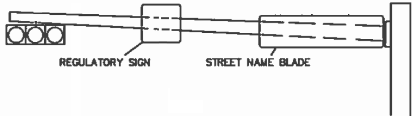
TYPICAL SIGN PLACEMENTS ON SIGNAL MAST ARMS
